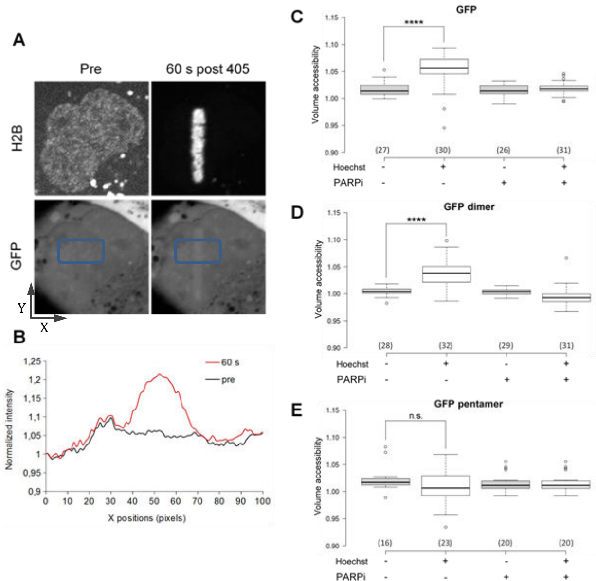
Figure 34: Impact of the DNA damage-induced chromatin relaxation on the volume exclusion effect caused by macromolecular crowding.
