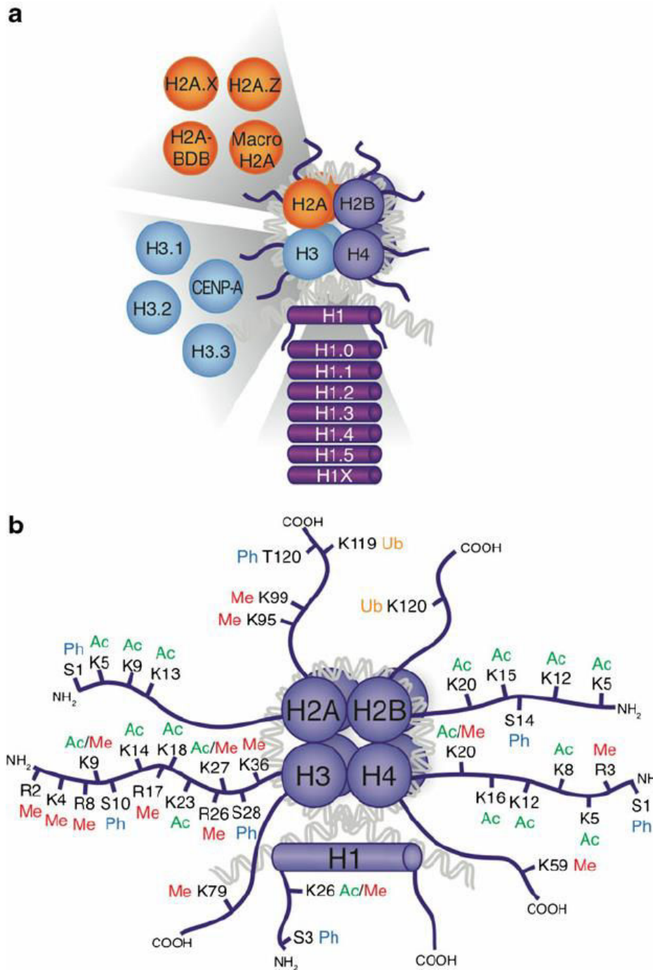
Figure 10: Histone post-translational modifications and variants.
