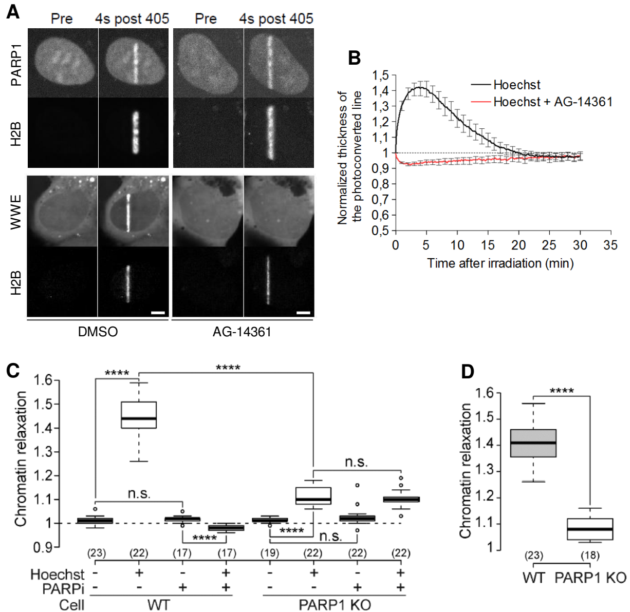
Figure 23: PARP1 activity controls chromatin relaxation at DNA damage sites.
