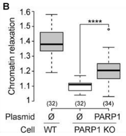
Figure 24: PARP1 is the key player regulating chromatin compaction state at DNA damage sites.
