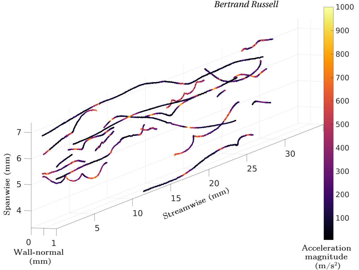
Figure 2.1: Selected tracer particle trajectories in the near wall region ( y^+ = 0 - 75 ) of a turbulent channel, representing the first fully resolved Lagrangian measurements ever made in such a flow. Note the extreme accelerations, up to 100 times that of gravity.
