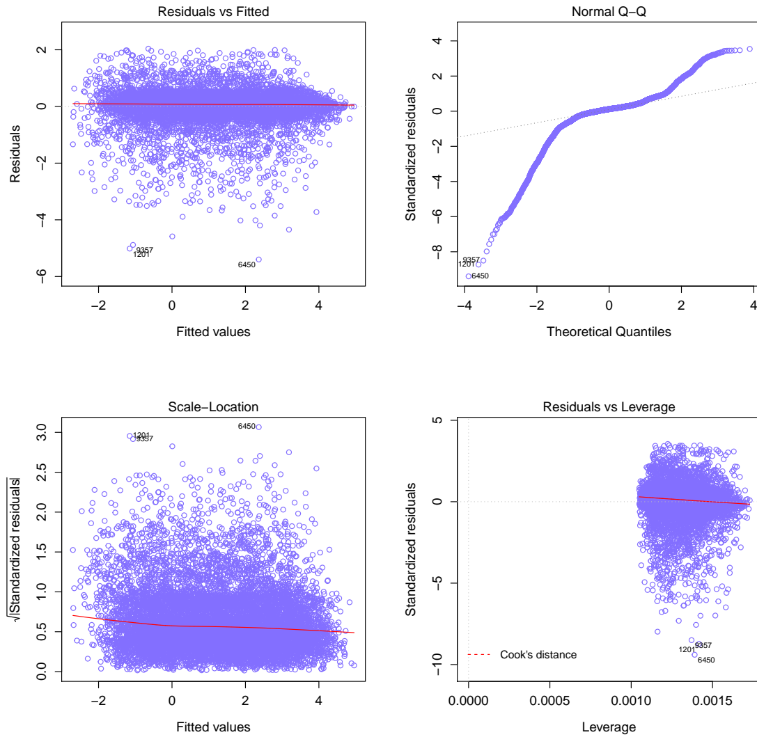
Figure 3.11: Diagnostic plots for the study of the regression model.
