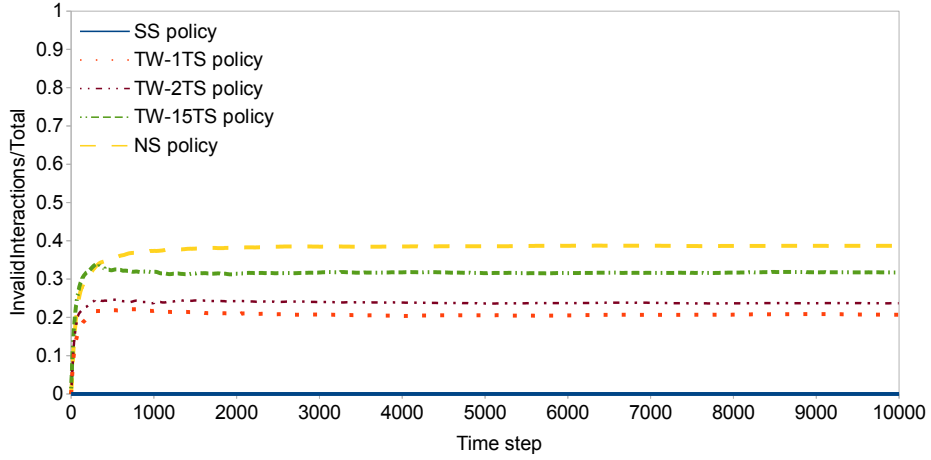
Figure 6.7: Invalid-TS Interactions between 8 machines in prey-predator model. In case of 8 or 4 machines (figure 6.6) we have the same percentage of these interactions. This is because, in both situations agents have 4 edge-zones to swap between machines.
