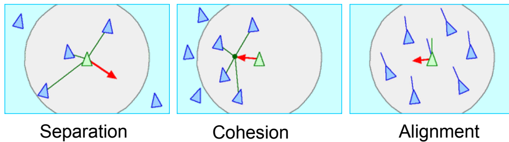
Figure 5.3: In flocking behaviour model: three main rules create the steering behaviour [Reynolds, 1987]: cohesion , alignment and separation .
