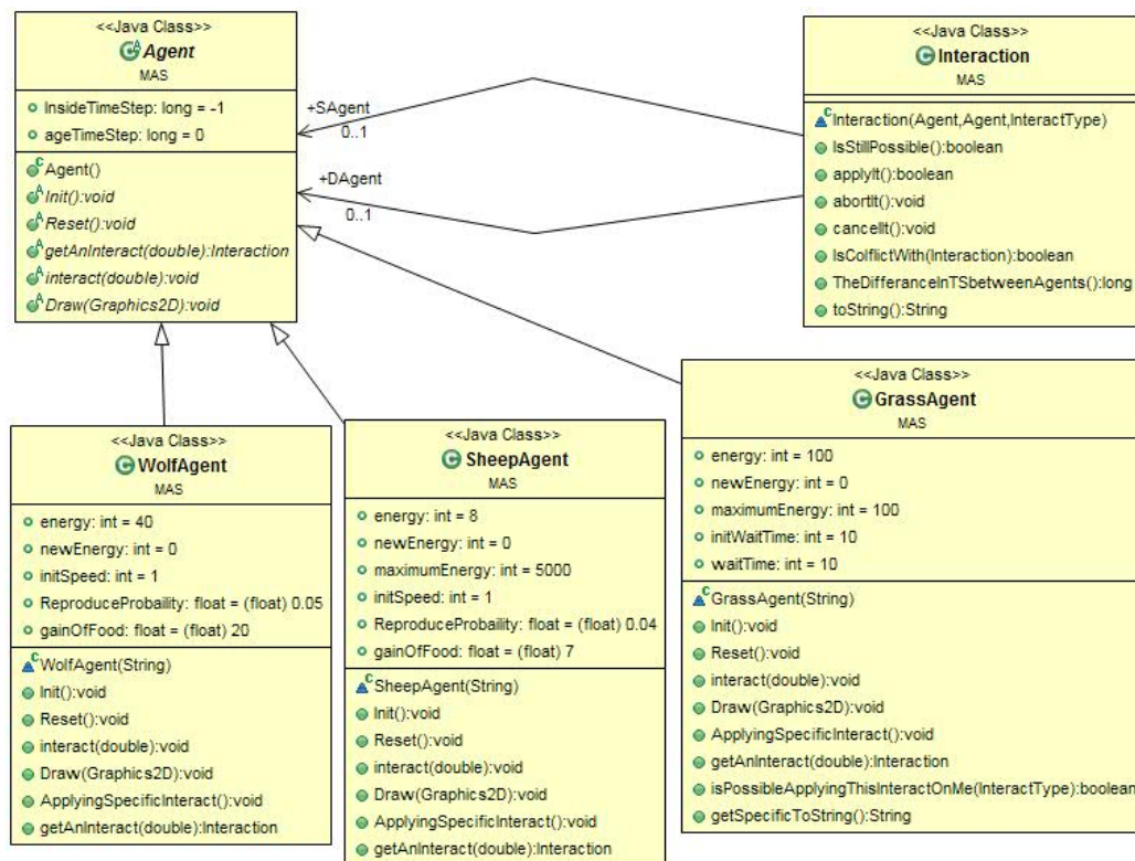
Figure 4.4: Agents UML class diagram for prey-predator model. Each agent type has to define a list of abstract functions to allow simulation from lunching the interaction process. The user can create many types of agents according to his application, and all these types must be inherited from the agent abstract class.
