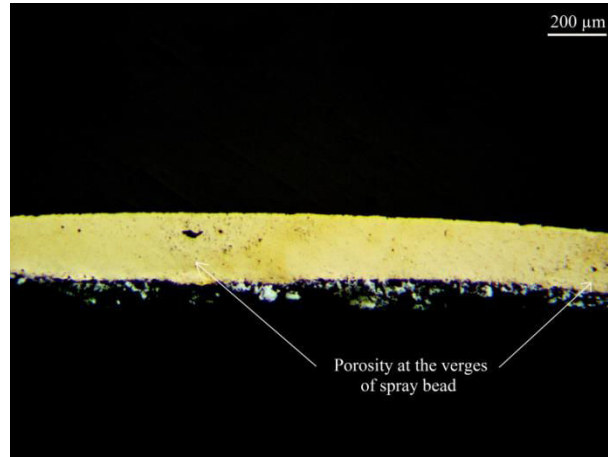
Fig. 86 Cu3 coating on PA6 with Sn+Al 2 O 3 interlayer (light microscope)
