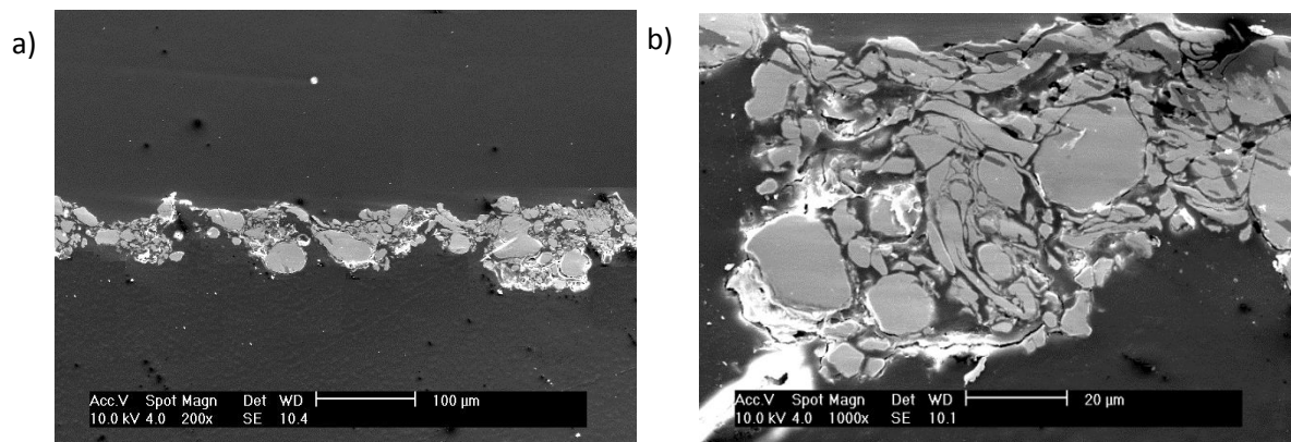
Fig. 63 Copper tracks deposited for parameters CC2 given in Tab. 11 (200x (a), 1000x (b), SEM)
