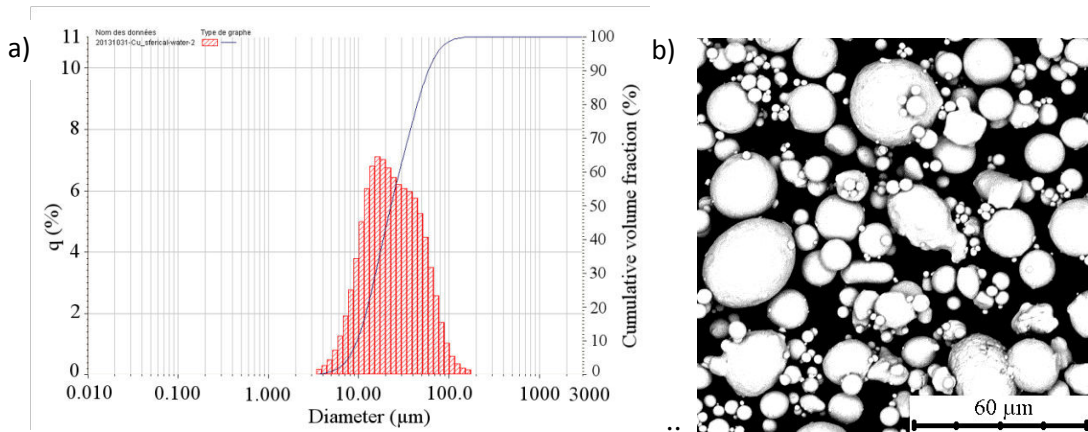
Fig. 29 Spherical copper powder: particles size distribution (a) and morphology (b)
