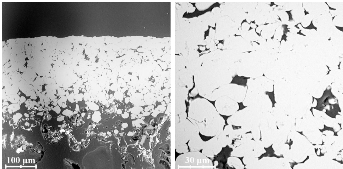
Fig. 82 Aluminum coating sprayed in two passes (A12-400 vel=3000) on PA6 (SEM)
