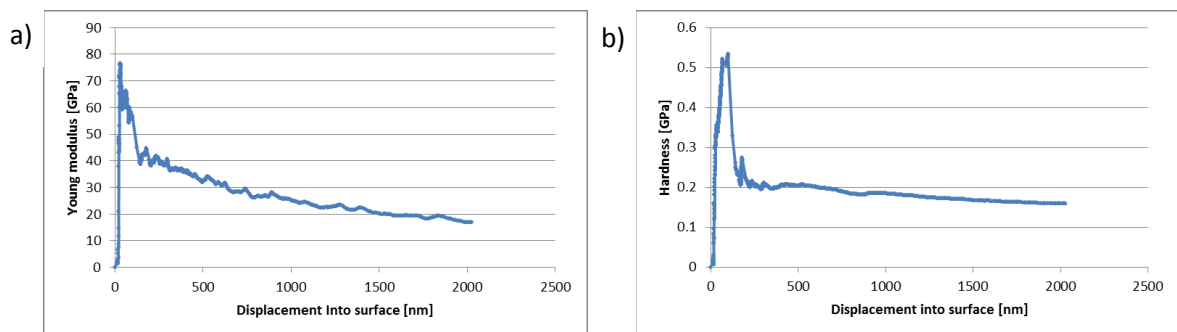
Fig. 78 Young modulus and hardness curve for Sn coating on PA6
