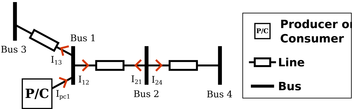
Figure 3.6: Current Flows
