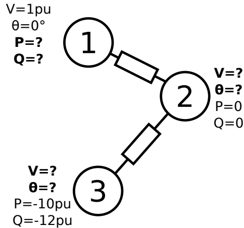
Figure 6.1: Example of Load Flow Problem
