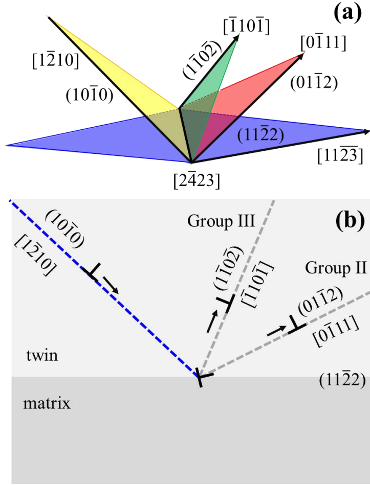
Fig. 4. 13 (a) Illustration of the common line between a prismatic plane, a Group II twinning plane, a Group III twinning plane and a primary twin plane along [2\bar{4}23] . (b) Schematic of reaction of a prismatic dislocation at a primary twin boundary into a Group II or a Group III twin dislocation plus a residual dislocation.
