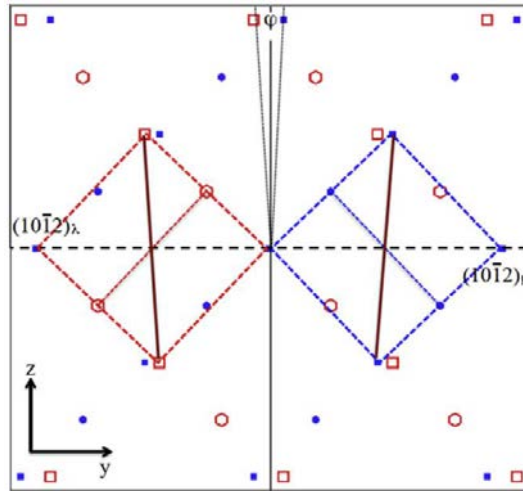
Fig. 1. 7 Coherent dichromatic complexes for a \{10\bar{1}2\} twin. The (1\bar{1}00) prism plane on the right and the equivalent (\bar{1}100) on the left are shown as solid lines. Both transposed to the centre with rotation angle \phi shown [117].
