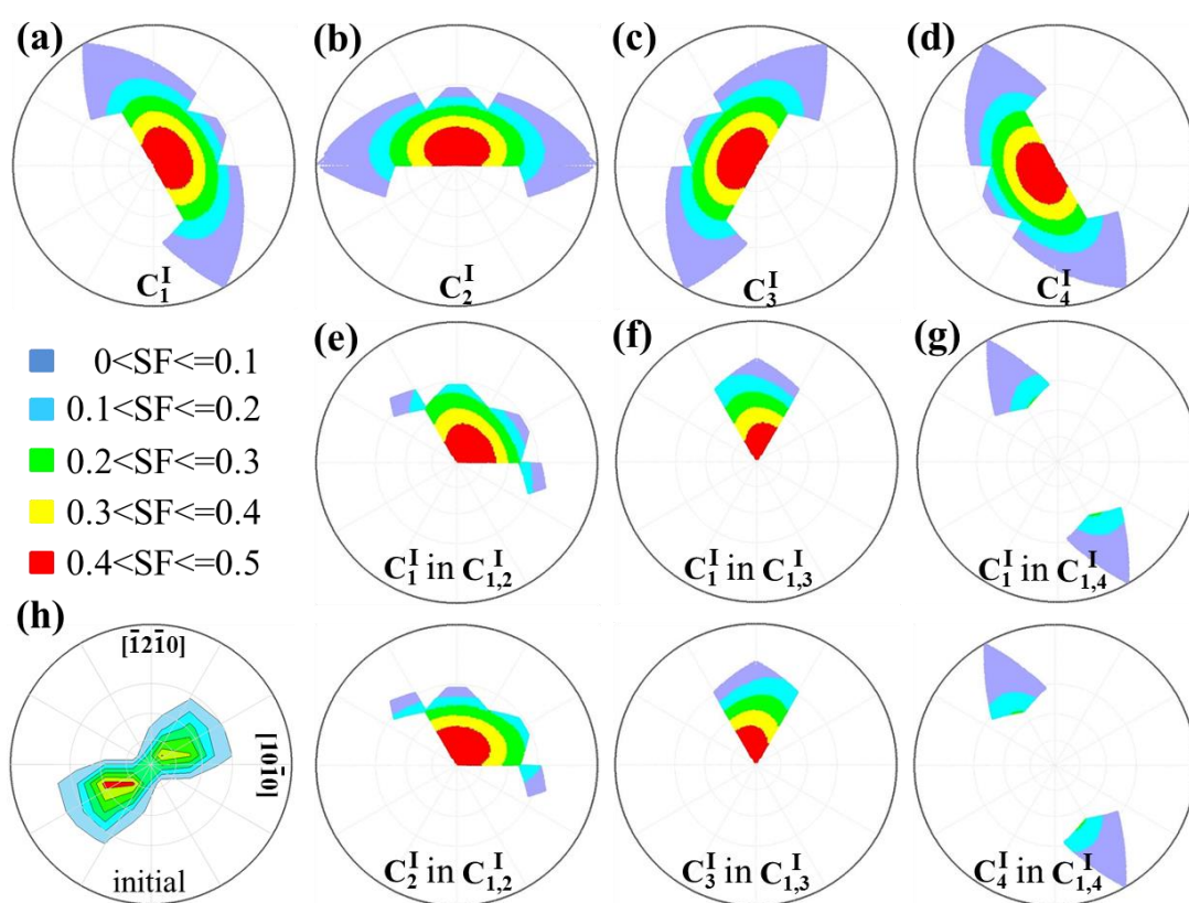
Fig. 5. 11 Loading domains associated with formation of TTJs (a) C_1^I , (b) C_2^I , (c) C_3^I , and (d) C_4^I . The common loading domains associated with the formation of TTJs (e) C_1^I in C_{1,2}^I and C_2^I in C_{1,2}^I , (f) C_1^I and C_3^I in C_{1,3}^I and (g) C_1^I and C_4^I in C_{1,4}^I . (h) Inverse pole figure of the initial grains.
