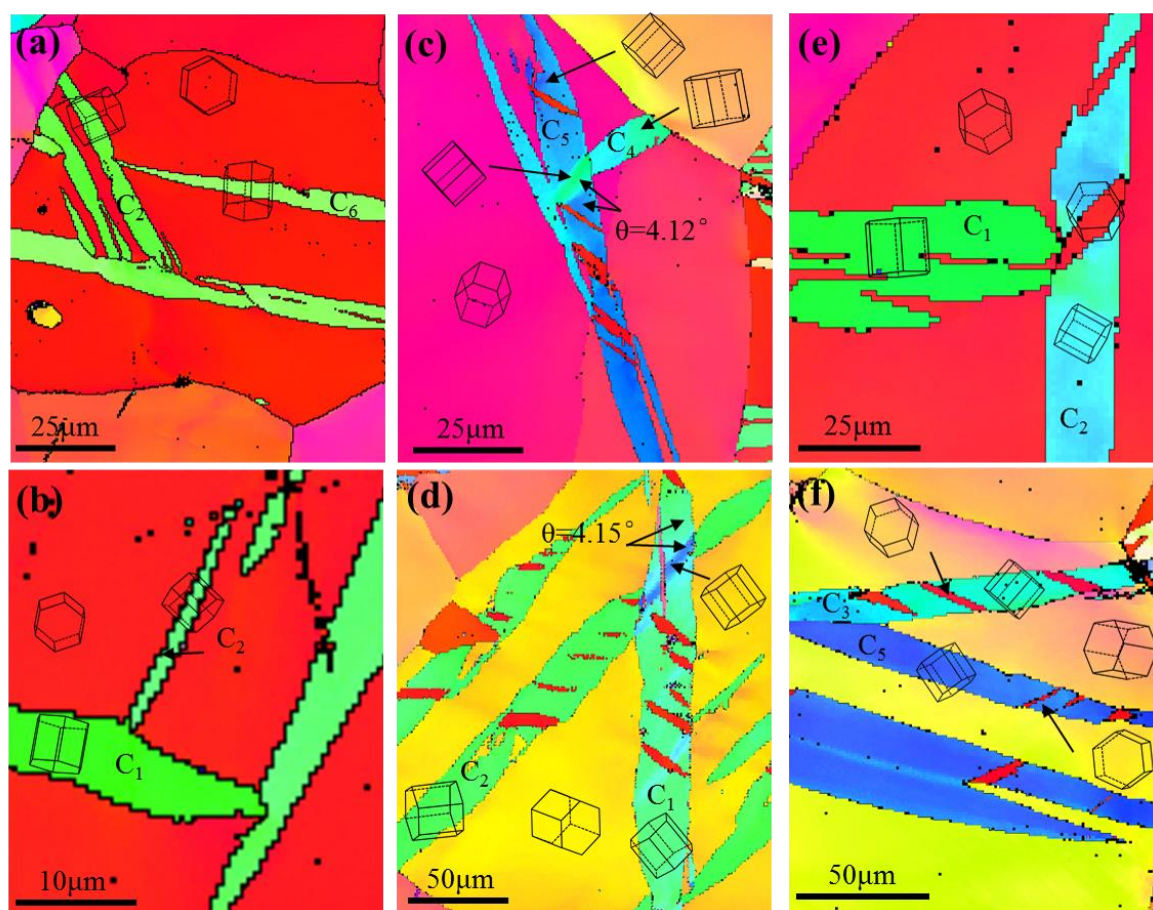
Fig. 5.4 (a-b) “Quilted-looking” structure of twin-twin junctions, (c-d) “Crossing” structure of twin-twin junctions, (e-f) Double twinning when twin-twin junctions form.
