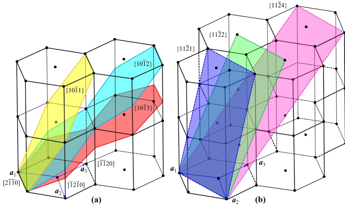
Fig. 1. 4 Main twinning systems in \alpha -titanium: (a) \{10\bar{1}1\} twinning plane in yellow, \{10\bar{1}2\} twinning plane in light blue and \{10\bar{1}3\} twinning plane in red (b) \{11\bar{2}1\} twinning plane in blue, \{11\bar{2}2\} twinning plane in green and \{11\bar{2}4\} twinning plane in pink.
