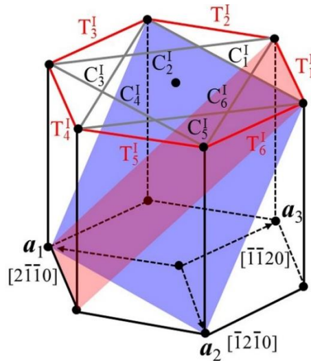
Fig. 4. 3 The crystallography of hexagonal structure. Two shadow planes are twin planes associated with contraction twin \{11\bar{2}2\} , C_1^I (blue), and extension twin \{10\bar{1}2\} , T_1^I (pink).
