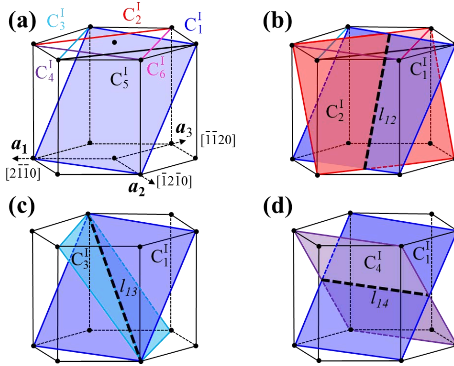
Fig. 5. 1 (a) Six \{11\bar{2}\} \langle 11\bar{2}\bar{3} \rangle ( C_i^I ) twin variants form three types of twin-twin junctions. (b) Type I C_{i,i+1}^I with the intersection line along [0\bar{2}23] ; (c) Type II C_{i,i+2}^I with the intersection line along [2\bar{4}23] ; (d) Type III C_{i,i+3}^I with the intersection line along [1\bar{1}00] . The bold dashed black lines indicate the intersection line.
