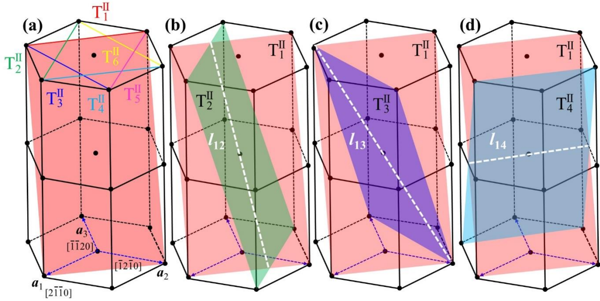
Fig. 5. 13 (a) Six \{11\bar{2}1\} \langle\bar{1}\bar{1}26\rangle ( T_i^{\text{II}} ) twin variants form three types of twin-twin junctions. (b) Type I T_{i,i+1}^{\text{II}} with the intersection line along [0\bar{0}13] ; (c) Type II T_{i,i+2}^{\text{II}} with the intersection line along [1\bar{2}13] ; (d) Type III T_{i,i+3}^{\text{II}} with the intersection line along [1\bar{1}00] . The dashed white lines indicate the intersection line.
