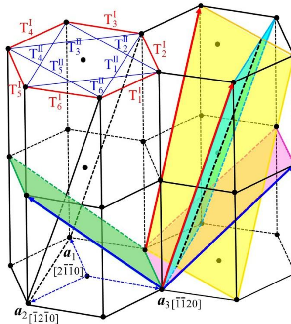
Fig. 3. 3 The crystallography of twins in hexagonal structure. Four shadow planes are twin planes associated with two \{11\bar{2}1\} twins, T_1^{\text{II}} (light green) and T_2^{\text{II}} (yellow), and two \{10\bar{1}2\} twins T_2^{\text{I}} (pink) and T_5^{\text{I}} (green). Two red arrows indicate the twinning shear directions of \{11\bar{2}1\} twins, and the blue arrows represent the twinning shear directions of \{10\bar{1}2\} twins.
