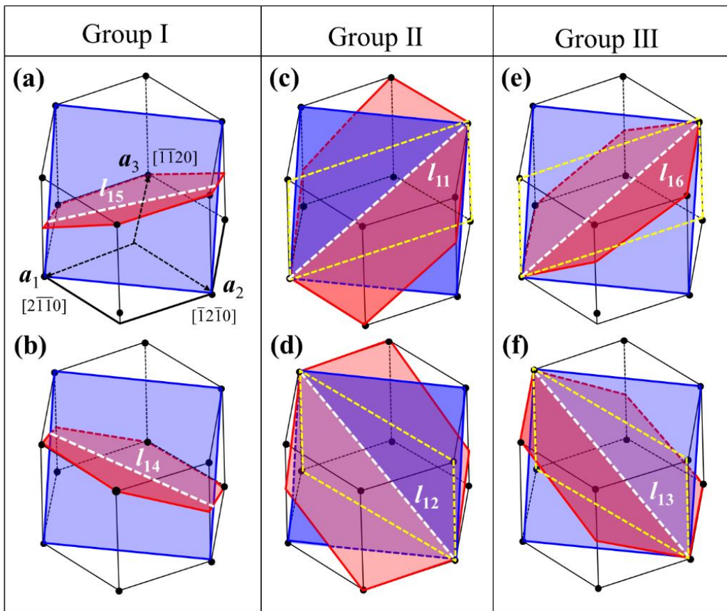
Fig. 4. 12 Crystallography of \{11\bar{2}2\} \rightarrow \{10\bar{1}2\} double twins. The blue plane denotes the primary twin C_i^I , and the pink plane represents the secondary twin T_j^I . The white dashed line indicates the intersection, l_{ij} , between the primary twin C_i^I and the secondary twin T_j^I . The yellow dashed lines outline a \{10\bar{1}0\} prismatic plane.
