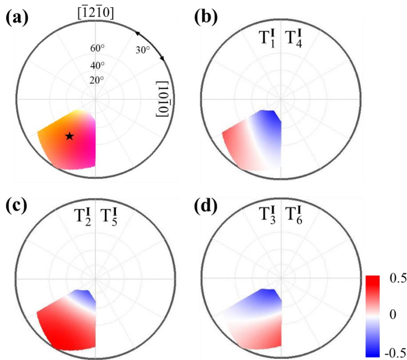
Fig. 3. 8 Inverse pole figures of the Schmid factor of twinning systems subjected to compression: (a) the loading domain in which SFs of T_1^{II} and T_2^{II} twins are positive and are greater than other four equivalent variants. Under this loading domain, the SF associated with sequential twin variants (b) T_1^I and T_4^I , (c) T_2^I and T_5^I , and (d) T_3^I and T_6^I . The blue color represents negative SFs, and red represents positive SFs (shown by the colorbar).
