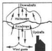
Raindrops and ice crystals drag air downward.
