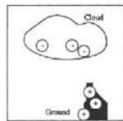
Lightning results from the difference in electrical charges between cloud and ground.
