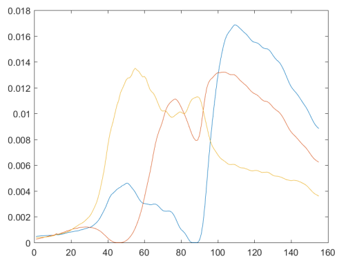
(c) NMF-multiplicatif
