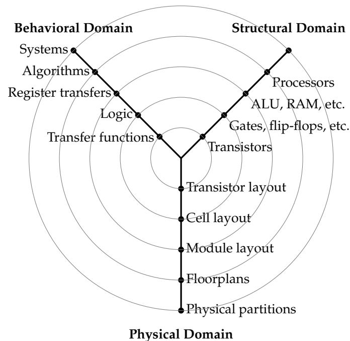
Figure 2.1: Gajski-Kuhn Y-chart [GK83].
