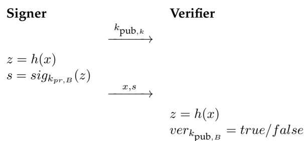
Figure 2.28: Basic protocol for digital signatures with a hash function.
