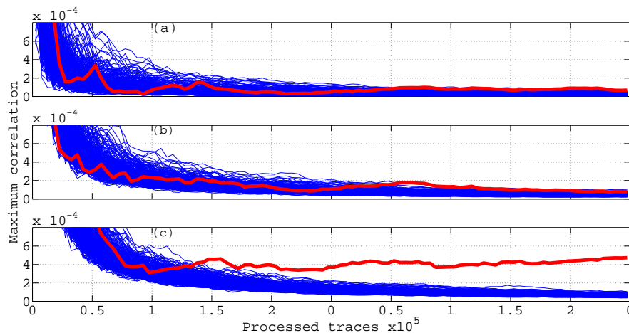
Figure 4.39: Maximum correlation coefficient for a byte of the last round AES key with simulated DVS. (a) CPA (b) CSBA (c) CIFA.
