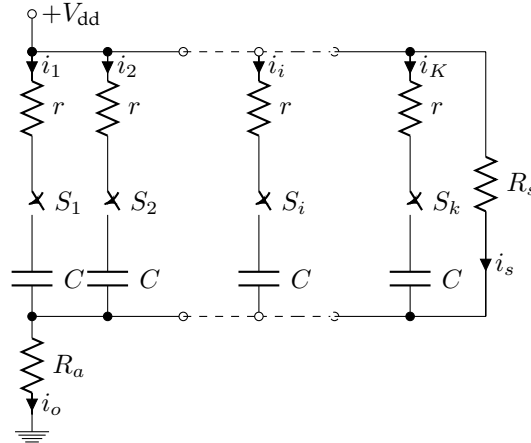
Figure 4.27: Inverters switch simulation.
