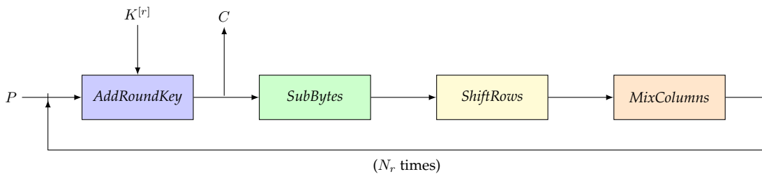
Figure 4.2: AES encryption flowchart.
