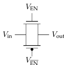
Figure 2.9: CMOS transmission gate.
