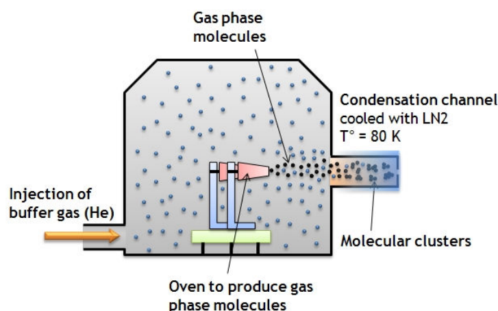
Figure 2.10 Design of the gas aggregation cluster source with marked important construction elements. The realization is a modified version of the cluster source developed by C. Bréchnac et al. [48].
