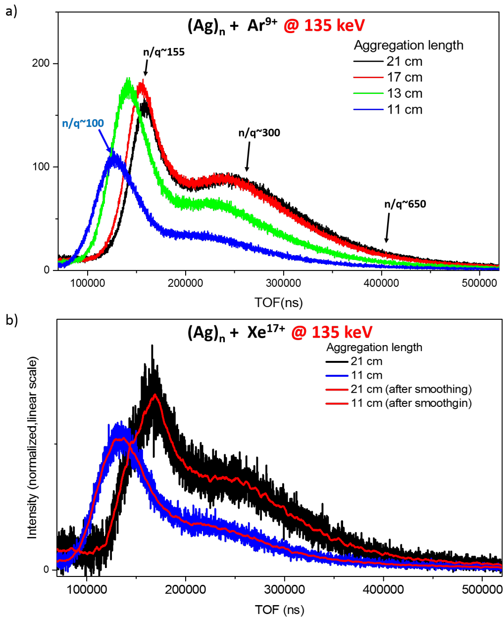
Figure 5.52 Mass spectra in the n/q range >50 and <700 for two different projectiles: a) Ar^{9+} and b) Xe^{17+} . The spectra correspond to different aggregation lengths in the magnetron cluster source.
