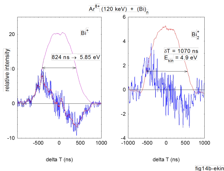
Figure 5.12 Peak forms of the monomer and dimer produced in collisions of \text{Ar}^{8+} ions with Bi clusters. The red and pink curves represent the relative peak intensity measured as a function of time.
