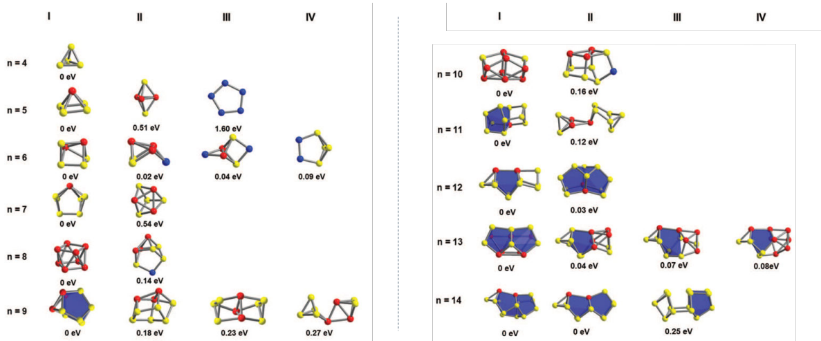
Figure 5.9 Calculated local minimum structures for \text{Bi}_4^+ to \text{Bi}_{14}^+ with optimized geometries at DFT level, based on the work of the group of Kappes, [79]. Roman numbers correspond to respective global minima (different isomers) while arabic number describe the number of Bi atoms in the cluster. Color of an atom refers to coordination number : 2-blue, 3-yellow, >4-red. Taken from [79].
