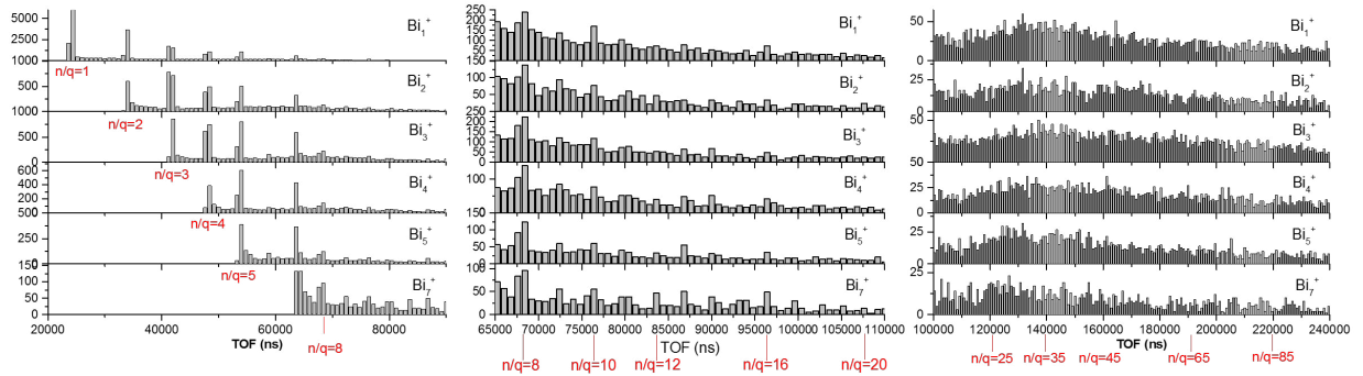
Figure 5.20 Correlations of small \text{Bi}_n^+ fragments with larger residues.
