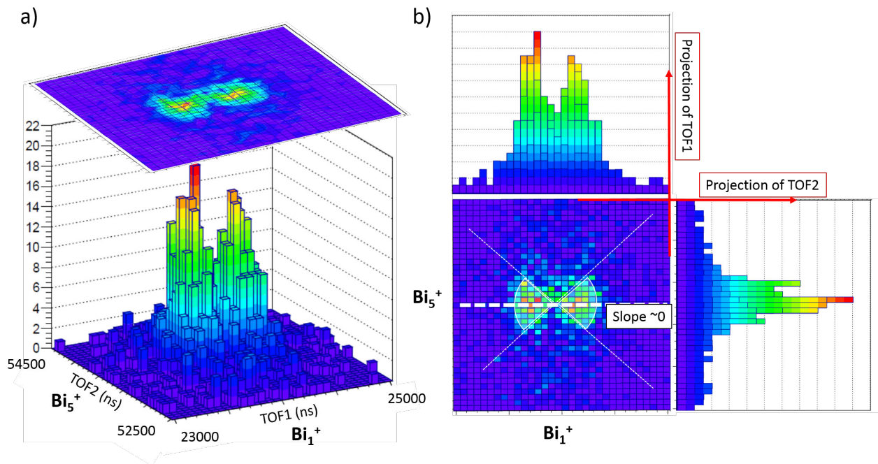
Figure 5.34 a) 3-dimensional intensity histogram of the island of the correlated pair ( \text{Bi}_1^+, \text{Bi}_5^+ ), b) 2d TOF representation of the same island with horizontal and vertical profile cuts.
