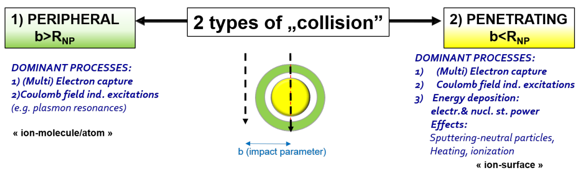
Figure 3.3 Schematical separation of the collision between a charged projectile and a metallic nanosphere based on the impact parameter: peripheral collisions (with impact parameters larger than the radius of the cluster) and penetrating collisions (with impact parameter smaller than cluster radius) with associated phenomena.
