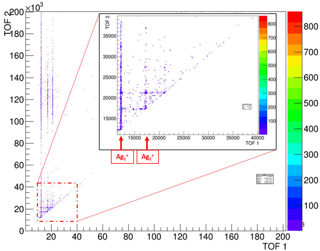
Figure 2.24 The coincidence map of fragments resulting from collisions of Ne^{6+} ions at E_{kin} = 90 keV with Ag_n . The inset in the right upper corner is a zoom into small TOF1 and TOF2 regions showing the characteristic coincidence islands and time of flights of silver monomers or dimers with residues of silver clusters. The color of the map represents the number of counts, and TOF1/TOF2 are given in \mu s .
