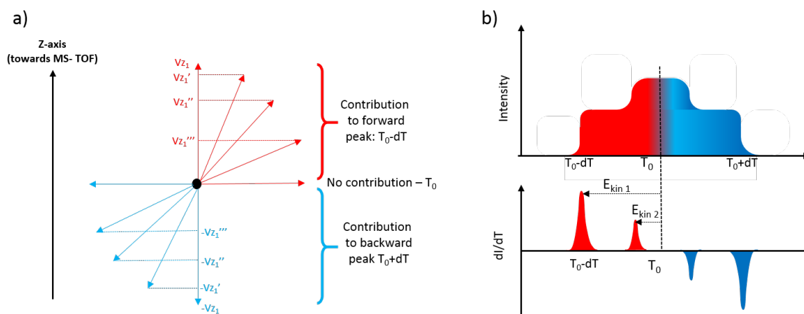
Figure 5.10 a) Schematical representation of the fragmentation of a charged particle into all possible directions with the given kinetic energy, with marked z-component of the velocity affecting time-of-flight. b) Upper graph shows hypothetical time-of-flight spectrum for a fragment with given mass m with two specific kinetic energies (all fragments emitted isotropically are detected), while the lower graph is the result after differentiation with characteristic peaks revealing kinetic energy components to the TOF spectra.
