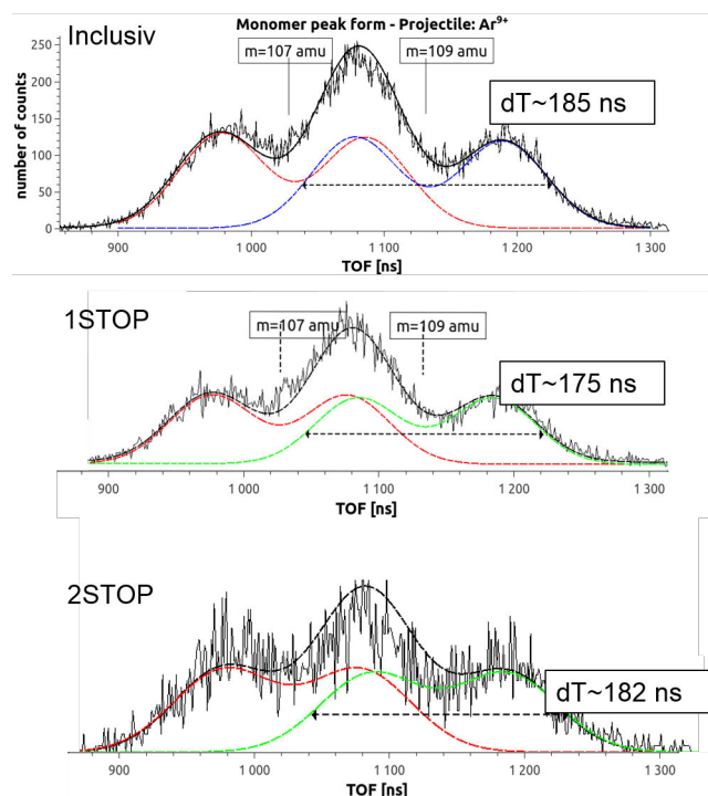
Figure 5.51 The comparison of the peak-forms (with hypothetical fits) of Ag monomer in case of inclusiv and 1,2 STOP spectra for the collision of silver neutral nanoparticles with Ar^{9+} at kinetic energy of 135 keV.
