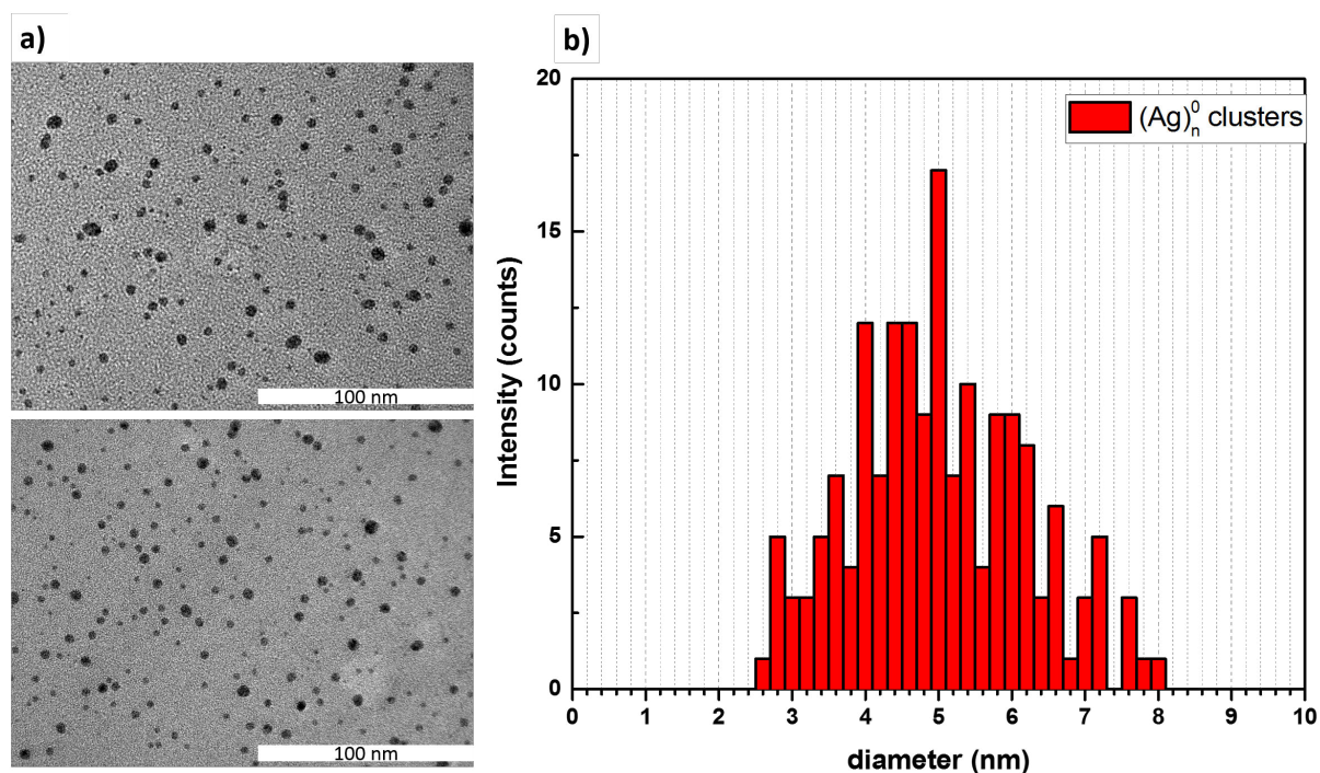
Figure 4.9 Deposited clusters on a SiO 2 substrate; b) histogram showing the size distribution of deposited neutral Ag n clusters
