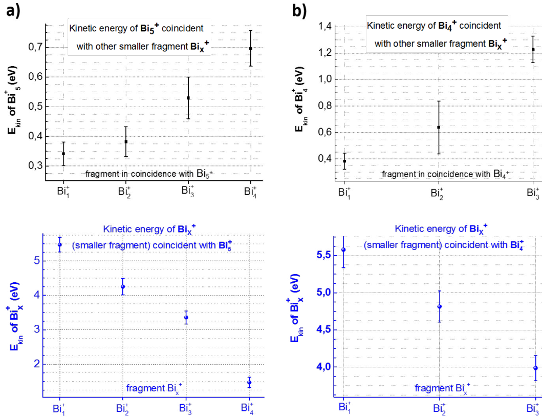
Figure 5.31 The measured kinetic energies of Bi pentamer (a-upper graph) and smaller fragment \text{Bi}_x^+ (a-lower graph) for correlation islands series ( \text{Bi}_{x=1-4}^+, \text{Bi}_5^+ ). b)- the Analogical graphs for series of ( \text{Bi}_{x=1-3}^+, \text{Bi}_4^+ ).
