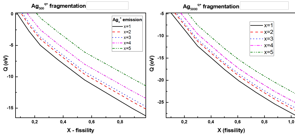
Figure 3.9 The Q values for different \text{Ag}_x^+ fragmentation channels in asymmetric fission in case of silver clusters with n=500 and n=5000 atoms as a function of their fissilities.
