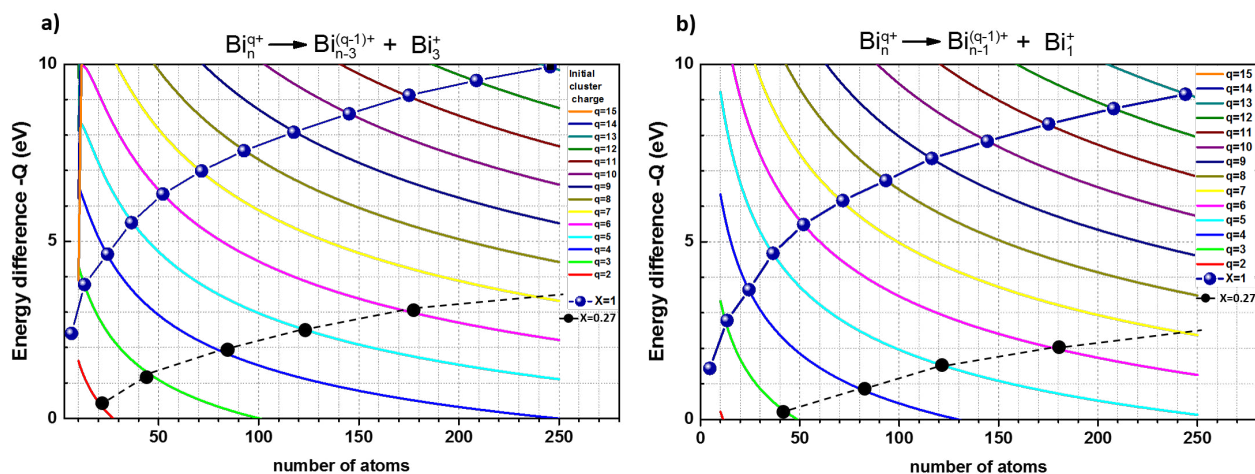
Figure 5.27 Q -values as a function of the cluster size for given charge states in case of the trimer emission a) and b) monomer emission.
