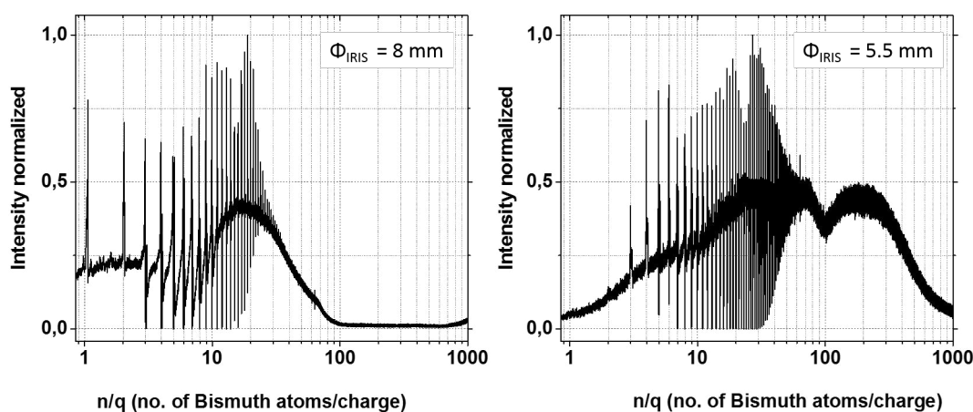
Figure 4.2 The mass spectra of positively charged Bi clusters produced by magnetron cluster source for two different IRIS diameters: a) \Phi_{IRIS}=8 mm and; b) \Phi_{IRIS}=5.5 mm.
