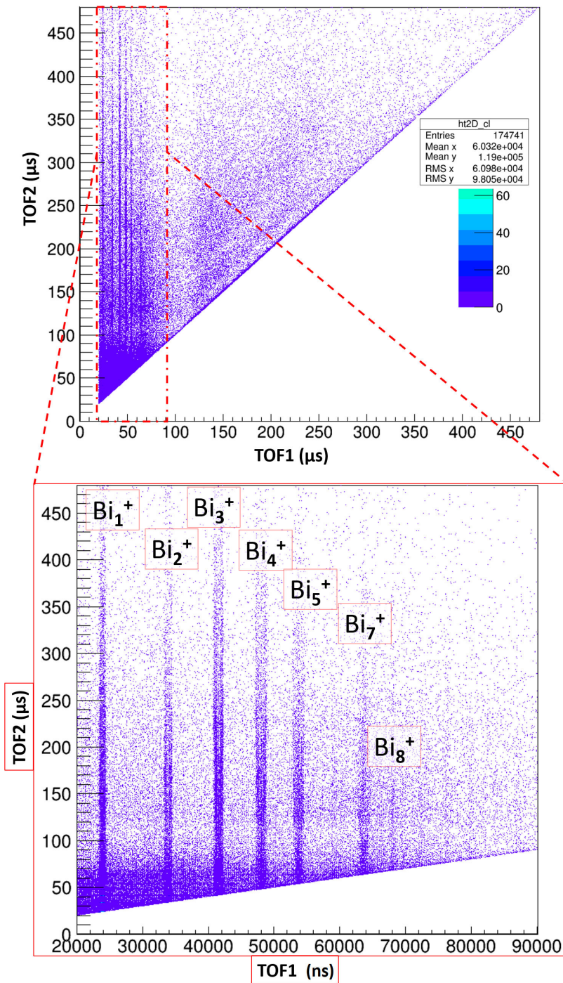
Figure 5.18 Two-dimensional representation of 2-Stop events of the corrected cleaned data set resulting from collisions of Bi_n with Ar^{8+} at 120 keV.
