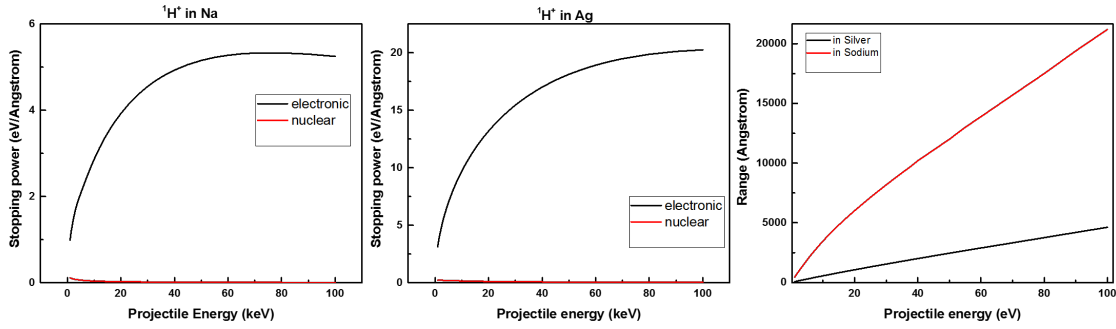
Figure 3.12 Illustration of the electronic and nuclear stopping power dependencies of protons in sodium and silver as a function of the kinetic energy (left and middle). In figure on the right the penetration depth is shown as a function of the energy. Results are based on SRIM Program calculations with ( E=1 to 100 keV).
