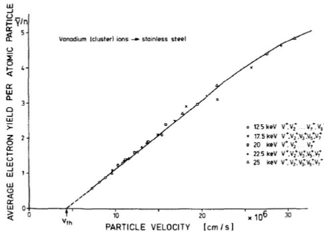
Figure 2.19 The average electron yield induced by the impact of energetic vanadium clusters V_n^+ ( n=1 to 9 ) on stainless steel with kinetic energies E_{kin} from 12.5 keV to 25 keV, [63].
