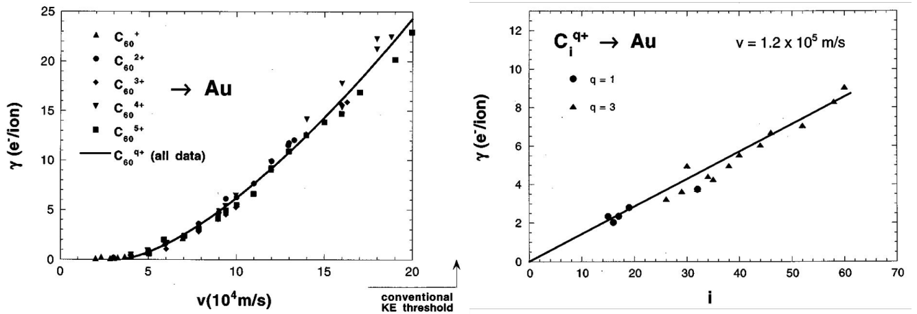
Figure 2.18 On the left: the yield for the production of secondary electrons produced by impact of singly and multiply charged C_{60}^{q+} (for q=1 to 5 ) fullerenes on a gold surface as a function of their velocity. On the right: the yield of produced secondary electrons as a function of the fullerene cluster size and charge state ( C_i^{q+} for i=15 to 60 and q=1 and for a given velocity of a projectile, [62].
