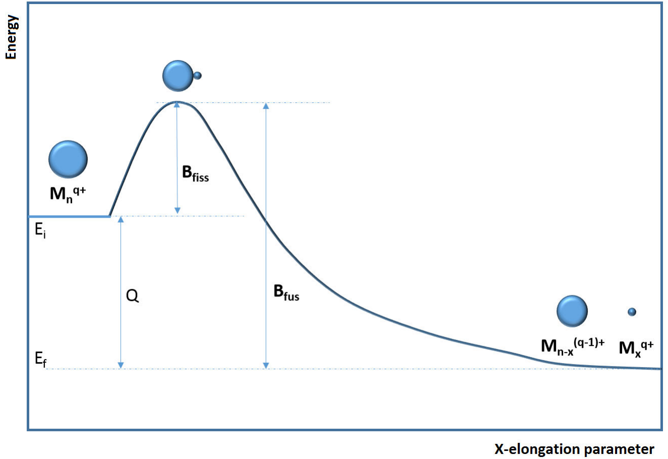
Figure 3.8 Fragmentation scheme for a multiply charged silver cluster based on the liquid drop model. It illustrates the relation between different fundamental quantities. The Y axis represents the energy of the system and X is the elongation coordinate (for large values it is the distance between the small fragment and the residue). Shown are the initial and final total energies of the system E_i and E_f , the fission and fusion barriers B_{fiss} and B_{fus} as well as their difference Q .
