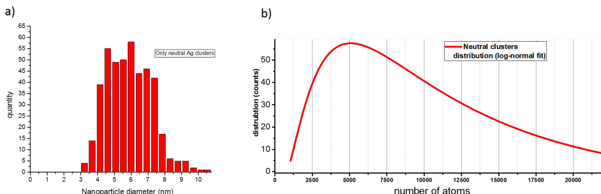
Figure 5.39 a) Size distribution of silver nanoparticles as a function of their diameter; b) Size distribution of silver nanoparticles as a function of the number of atoms (log-normal fit).
