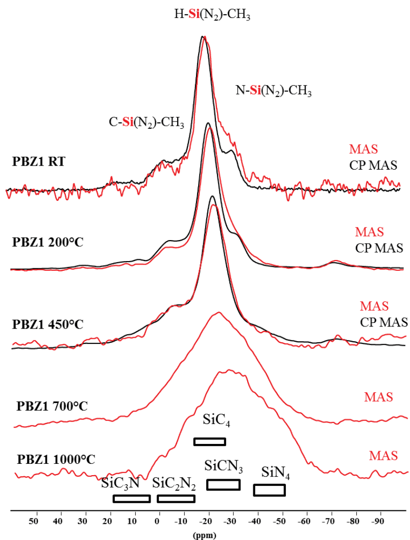
Figure V-38: ^{29}\text{Si} MAS (red) and CP MAS (black) NMR spectra of PBZ1 from RT to 1000°C.
