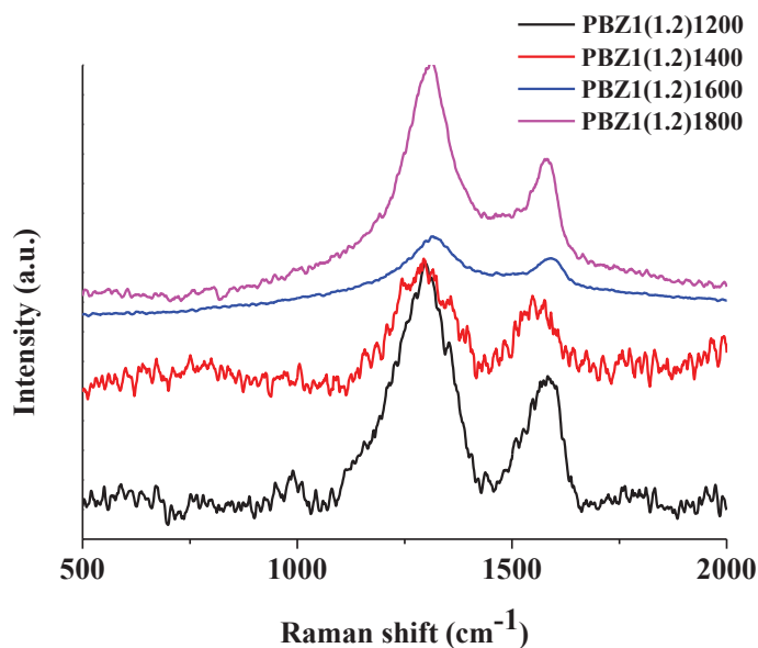
Figure V-42: Raman spectra of SiBCN powders obtained from sample PBZ1 annealed under \text{N}_2 at 1200, 1400, 1600 and 1800°C.
