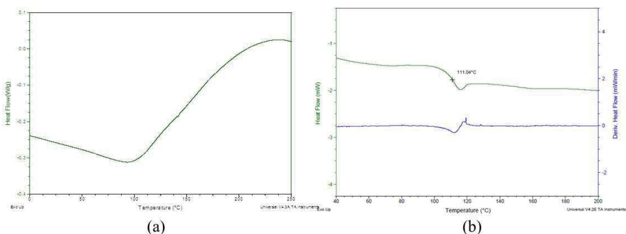
Figure V-24: DSC curves for (a) PAAZ and (b) PMMA-25 \mu\text{m} under \text{N}_2 with 5^\circ\text{C}.\text{min}^{-1} as heating rate.
