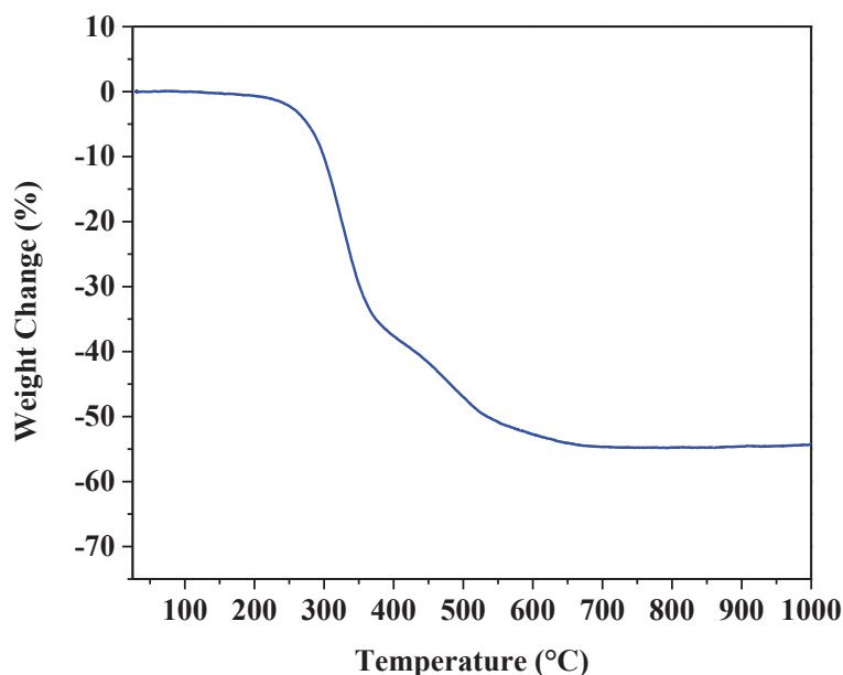
Figure V-12: TGA curve of boron-modified polysilazane of the type (B[C_2H_4SiCH_3NH])_3)_n under N_2 up to 1000^\circ C with a heating rate of 5^\circ C \cdot min^{-1} .
