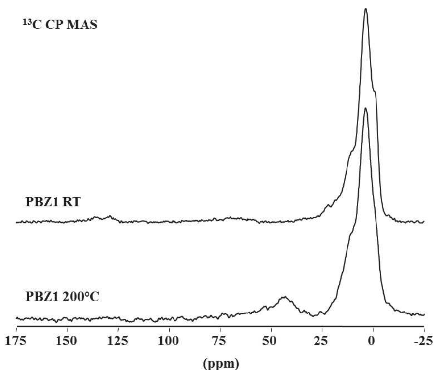
Figure V-37: ^{13}\text{C} MAS NMR spectra of PBZ1(1.2) and N 2 -treated intermediate at 200°C.
