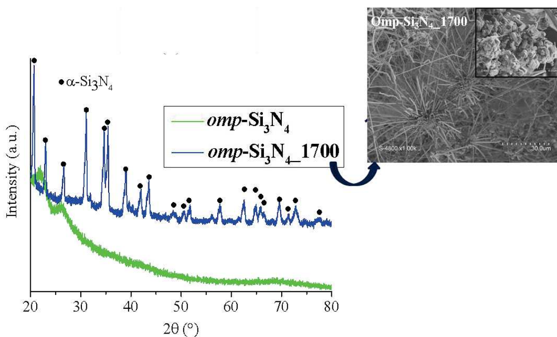
Figure IV-29: XRD patterns of omp - \text{Si}_3\text{N}_4 and omp \text{Si}_3\text{N}_4 _1700.
