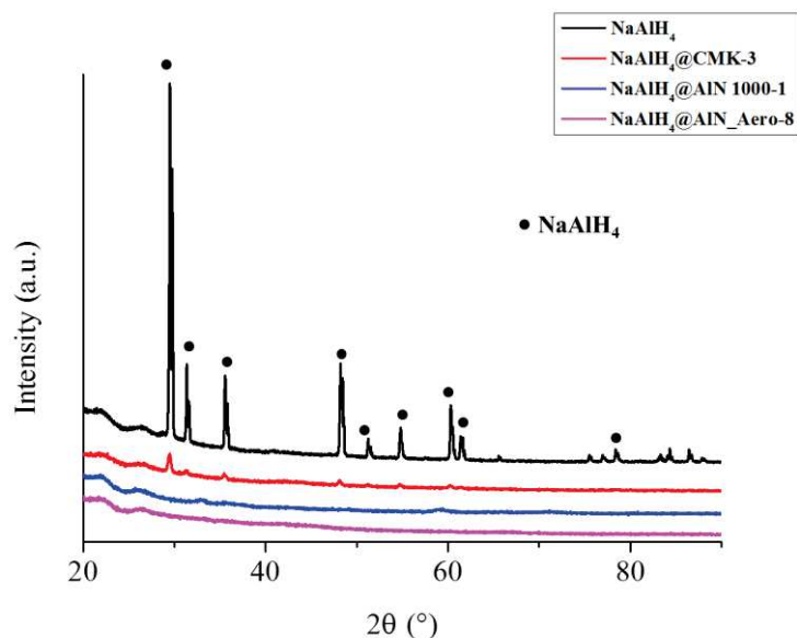
Figure II-23: XRD patterns of neat NaAlH 4 , NaAlH 4 @CMK-3, NaAlH 4 @AlN 1000-1 and NaAlH 4 @AlN_Aero-8.
