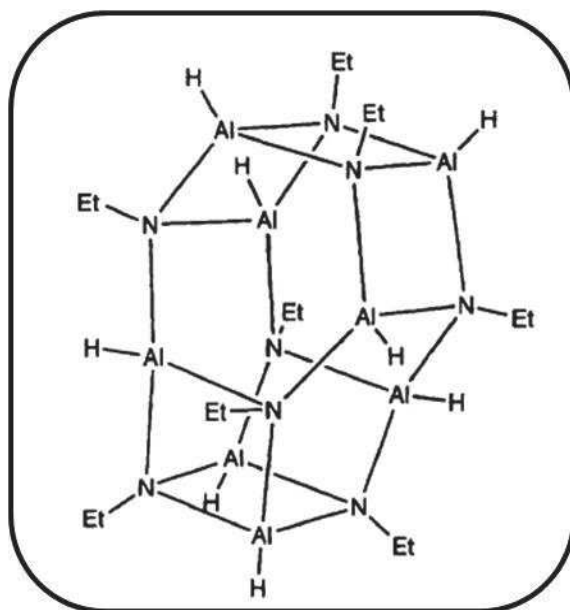
Figure I-13: Structure of poly(ethylaluminum hydride) [125].
