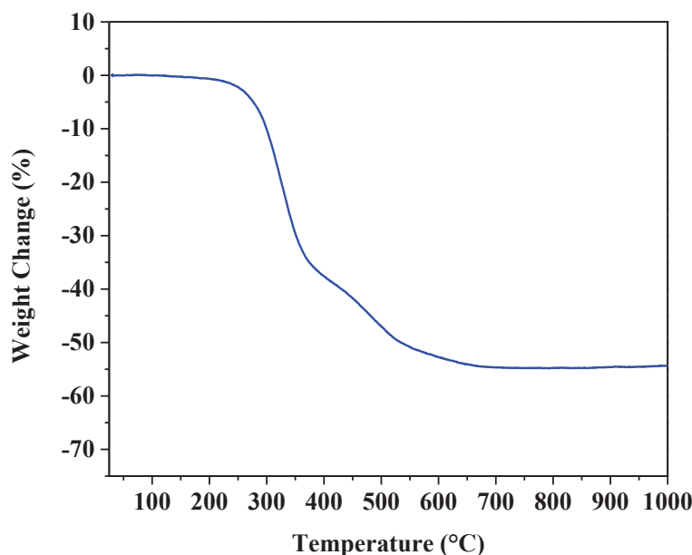
Figure V-12: TGA curve of boron-modified polysilazane of the type (B[C_2H_4SiCH_3NH])_3)_n under N_2 up to 1000°C with a heating rate of 5^\circ\text{C}.\text{min}^{-1} .
