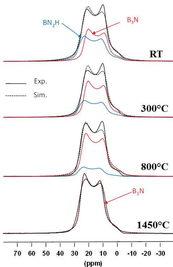
Figure III-4: Solid-state ^{11}\text{B} MAS NMR experimental and simulated spectra of PB and N 2 -treated intermediates at 300, 800 and 1450°C.
