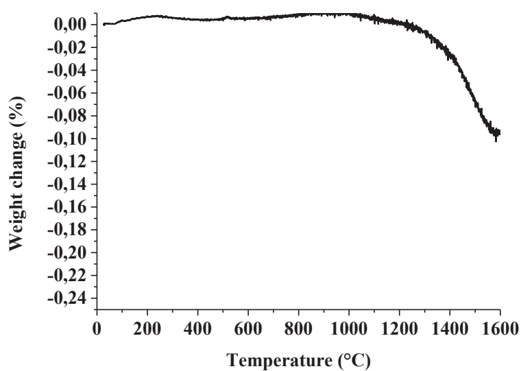
Figure V-43: HTTGA curve of PBZ1(1.2)1000 during annealing to 1600°C under \text{N}_2 (heating rate 5°C.min ^{-1} ).
