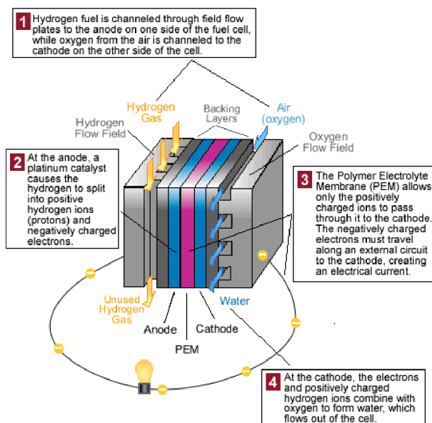
Figure IV-1: PEMFC system [278].
