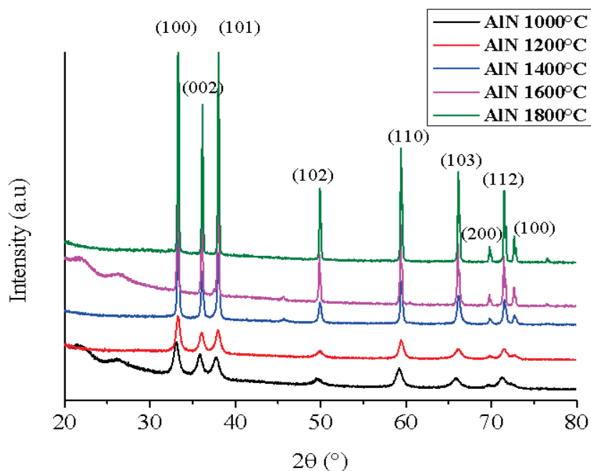
Figure II-9: XRD patterns of PEIA-1000 between 1000 and 1800°C under N 2 .
