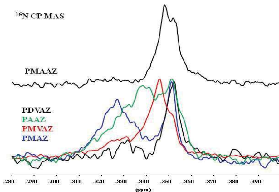
Figure V-10: ^{15}\text{N} MAS NMR spectra of PMAAZ, PMVAZ, PAAZ, PMAAZ and PDVAZ.
