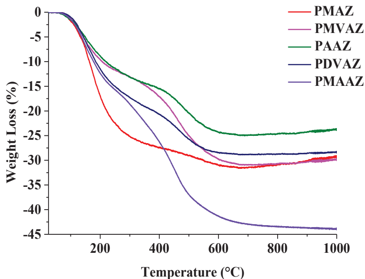
Figure V-11: TGA curves of PMAZ , PMVAZ , PAAZ , PMAAZ and PDVAZ under N 2 up to 1000°C (5°C.min -1 ).
