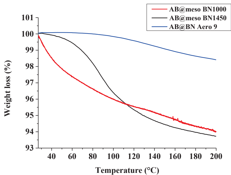
Figure ANNEX B-2: TGA curves of AB@mesoBN1000, AB@mesoBN1450 and AB@BN Aero 9 under \text{N}_2 up to 200 ^{\circ}\text{C} with a heating rate of 5^{\circ}\text{C}.\text{min}^{-1} .
