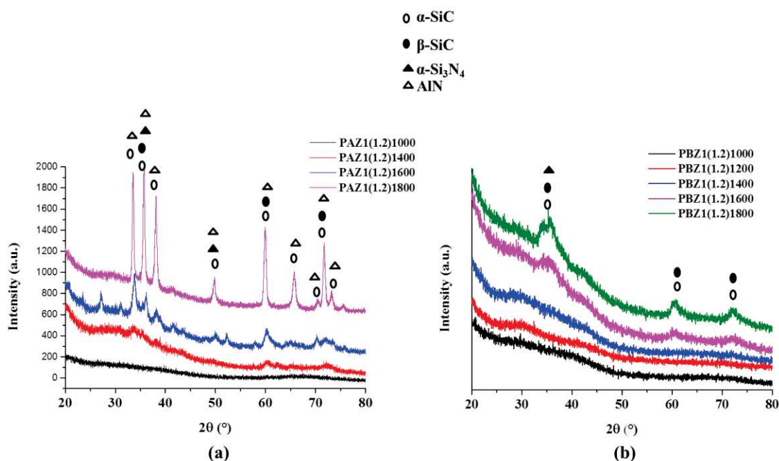
Figure V-41: XRD patterns of (a) PAZ1(1.2) and (b) PBZ1(1.2) heat-treated at 1000, 1400, 1600 and 1800°C.
