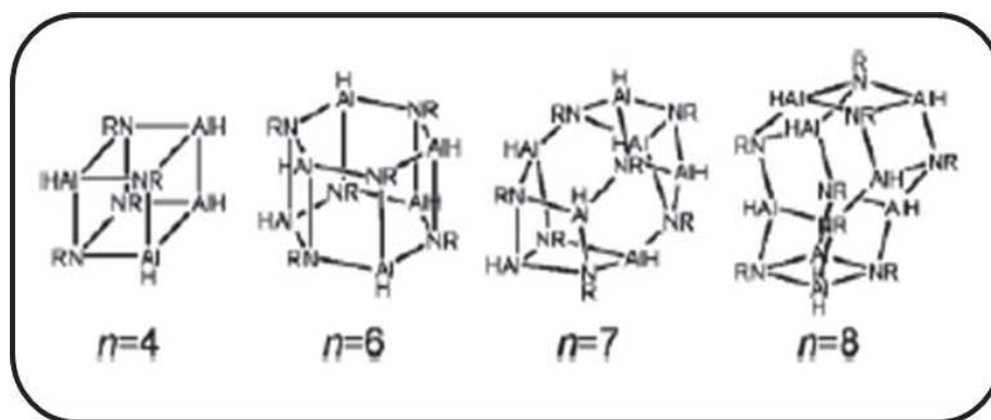
Figure I-12: Structure of poly(alkyliminoalane) [\text{HAlNR}]_n with n = 4, 6, 7, 8 [154].
