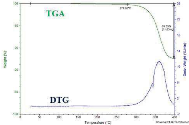
Figure V-25: TGA and DTG curves for PMMA-25 \mu\text{m} under \text{N}_2 with 5^\circ\text{C}.\text{min}^{-1} as heating rate.
