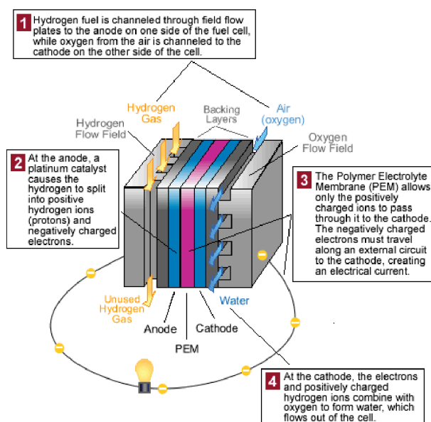
Figure IV-1: PEMFC system [278].
