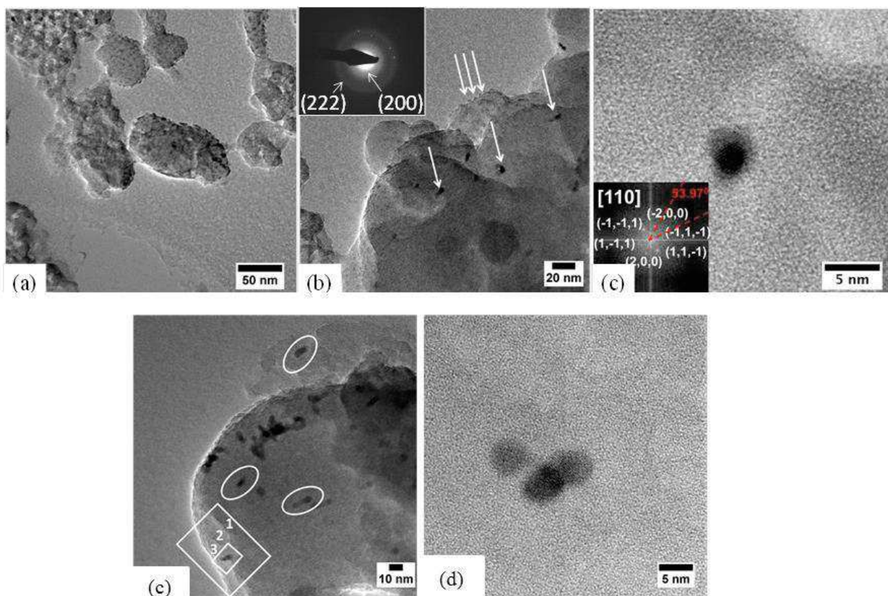
Figure IV-34: TEM images of \text{Pt}/omp\text{-Si}_3\text{N}_4 .
