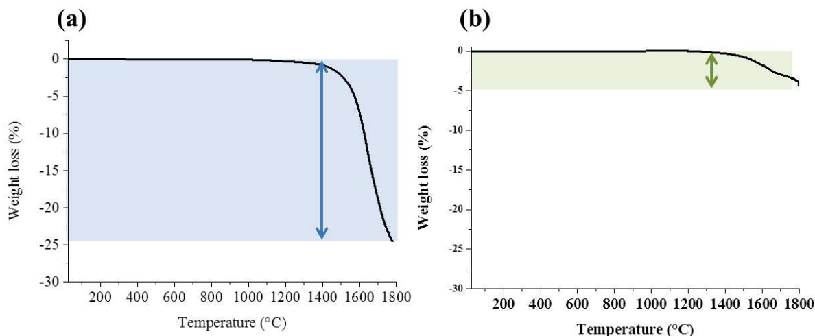
Figure V-29: HTTGA curve of (a) PAAZ30/PMMA70-80-74-1000°C and (b) PAAZ-1000°C under N_2 up to 1800°C with a heating rate of 5^{\circ}C.min^{-1} .
