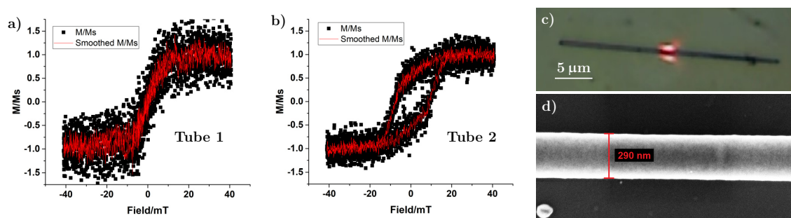
Fig. 8.9: Magnetometry on a single tube - magneto-optics with focused laser. Hysteresis loops for the axial magnetic field (longitudinal MOKE): a) slanted curve, b) rather squared loop obtained on another tube. Average of 100 loops with a short acquisition time (0.9 s). Data processed in OriginPro: line subtracted, normalized, smoothed: average of 7 adjacent points (red curve) – original curve had 5000 points (black points). c) Optical image (magnification 100x) of a tube with the diffracted laser spot, the magnetic field is applied in the horizontal direction, close to parallel to the tube axis. d) Scanning electron microscopy image of a central part of the tube from c).
