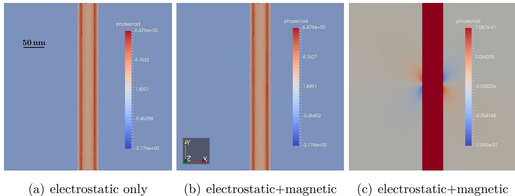
Fig. S4: Simulation of electron holography phase map with electrostatic contribution for Bloch wall (radial magnetization) in between 2 opposite azimuthal domains in a tube (for magnetic part only see in Fig. S3a). (a) Electrostatic part only. The highest phase shift is close to tube edges where the electron path travelled through the tube is the longest; the spatial extent corresponds roughly to the tube wall (shell) thickness. (b) and (c) depict both electrostatic and magnetic parts scaled to (a) full range of the phase, (b) small range around zero. The electrostatic part dominates and in experiment one cannot probably clearly see the weak magnetic signal without removing the electrostatic contribution. Even here it is almost impossible to spot a small difference between (a) and (b).
