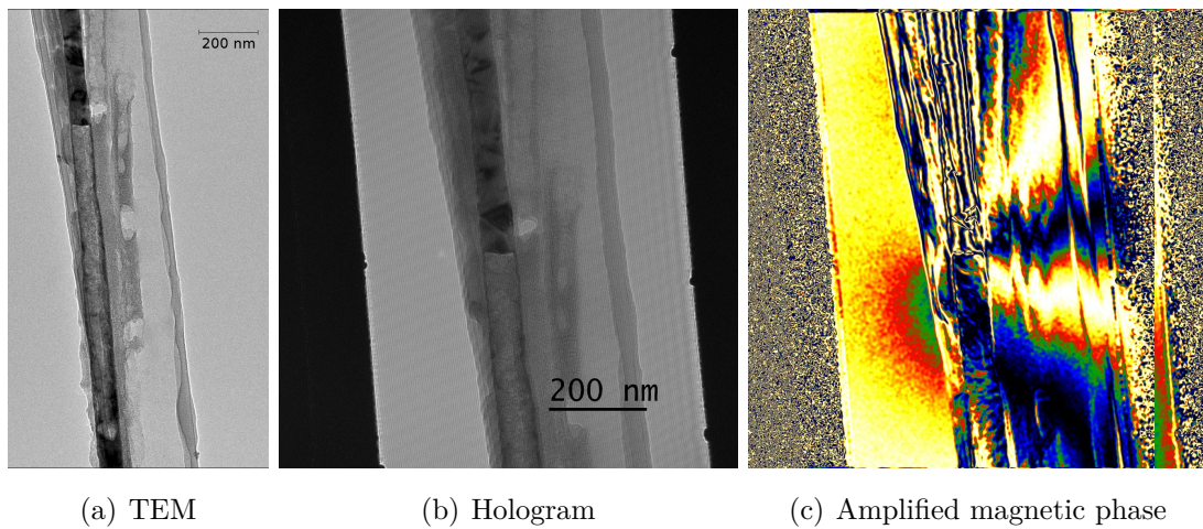
Fig. 7.5: Electron holography on wire-tube-wire Ni nanostructure. (a) TEM image of the whole tube part with wire segments at both ends that extend microns in both directions. (b) Hologram of the upper wire-tube transition and (c) corresponding "amplified" magnetic phase shift reconstruction -\cos(3\phi_m) is displayed instead of the magnetic phase \phi_m . Here we can observe stray field coming from the wire-tube transition (mainly to the right of the structure). Except for the transition, magnetization seems to be uniform, along the wire axis. Unfortunately, we cannot say much about the tube part. Low tube wall thickness, together with possible oxidation and lower Ni magnetic moment provides only a feeble signal.
