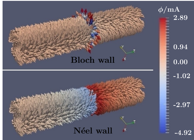
Fig. 9.2: Micromagnetic modelling of Bloch and Néel wall in a tube with two opposite azimuthal domains. Example for tube diameter of 120 nm, shell thickness 30 nm, length 1000 nm, and cell size < 4 nm. The effective anisotropy constants (hard axis along the tube) are 30 \text{ kJ/m}^3 and 100 \text{ kJ/m}^3 for obtaining Néel and Bloch walls, respectively. Colouring reflects magnetic charges whose spatial extent is significantly larger for the Néel wall. For better view on the magnetization consult unrolled maps in Fig. 9.3.
