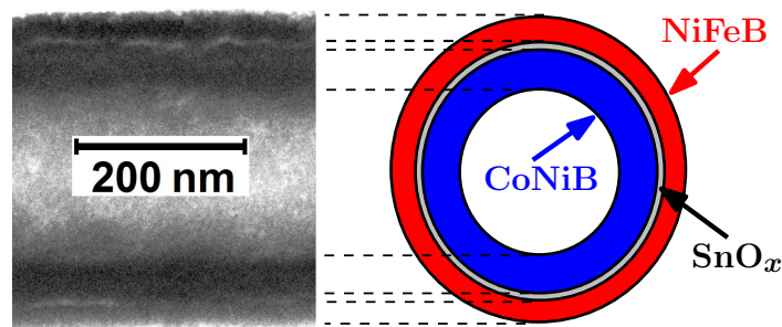
Fig. 11.1: Multilayered tube with a non-magnetic (oxide) spacer. Experimental realization (left) – transmission electron microscopy of a tube segment (electrons arrive perpendicular to the tube axis). The oxide spacer appears as a brighter line in the tube wall. Scheme to the right highlights the different layers of the tube.
