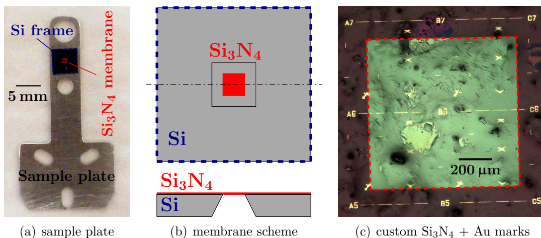
Fig. 5.6: \text{Si}_3\text{N}_4 membranes for STXM. a) Photo of a metallic sample plate with the membrane (edge of the Si support frame is 5 mm), X-rays arrive perpendicular to the plane. b) Scheme of the \text{Si}_3\text{N}_4 membrane on the Si support frame (bottom and cross-section side view). c) Optical image (top view) of a custom-made \text{Si}_3\text{N}_4 membrane (Nanofab, Institut Néel) with Au (40 nm) alignment marks. The brighter inner square highlighted by the dashed red square corresponds to the membrane "window" (membrane edge 0.7 mm, thickness 200 nm). There are magnetic tubes dispersed on top of the membrane as well as many impurities from the template dissolution. These impurities (extreme case shown, cleaner samples with aligned tubes were used as well) are not an issue for STXM, however, for XMCD-PEEM such sample would be unusable.
