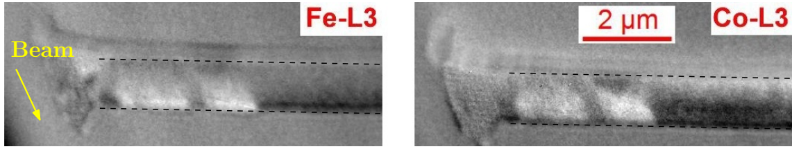
Fig. 11.5: NiFeB/Pd(incomplete)/CoNiB – coupled magnetic layers (SS147 sample). XMCD-PEEM images Fe-L 3 and Co-L 3 edge, respectively. Arrow depicts the beam direction; the approximate shadow extent is marked by dashed lines. The gradual change in the contrast in the shadow suggests azimuthal magnetization in both layers. Tube end displays similar defect as in Fig. 11.4.
