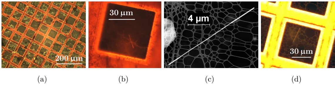
Fig. 5.9: Nanostructures on TEM grids for electron holography imaging. (a) Optical image of a larger part of the Cu grid. The size of each window is around 55\ \mu\text{m} . (b) closer look with optics on a NiCo nanowire on the porous carbon film at the bottom of the window. (c) Scanning electron microscopy of another NiCo diameter modulated nanowire. (d) Optical image of a CoNiB tube on the film.
