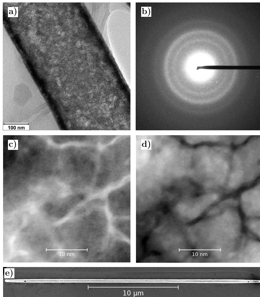
Fig. 8.1: Structure of electroless-deposited CoNiB nanotubes (SS53 sample). a) Transmission electron microscopy image of a nanocrystalline CoNiB tube and b) corresponding selected area (240 nm in diameter) electron diffraction pattern showing diffuse rings originating from nanograins with all possible crystallographic orientations. c) Closer look on the grains with scanning transmission electron microscopy in bright and d) dark field ( Z contrast, heavier elements appear brighter). e) Scanning electron microscopy image of a whole tube (another tube, same batch). STEM images courtesy of Eric Gautier.
