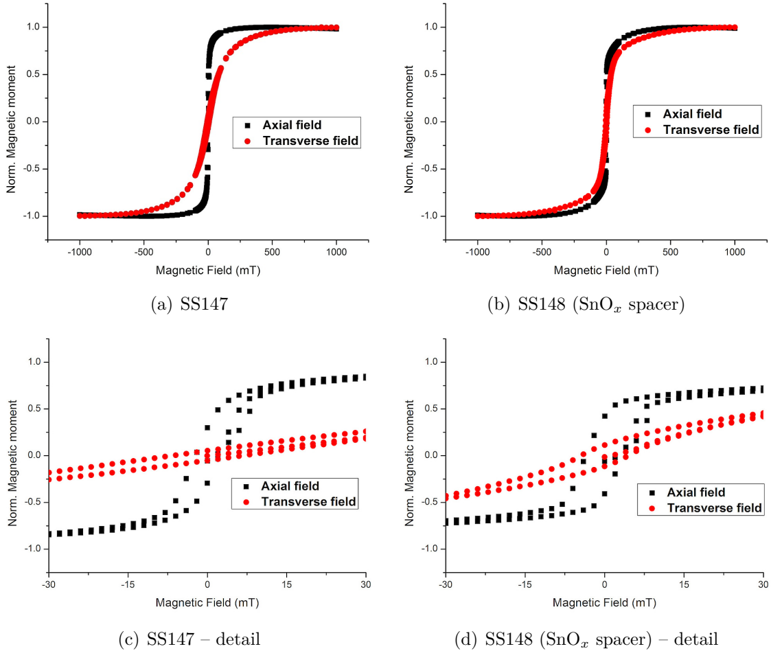
Fig. 11.8: Magnetometry on arrays of multilayered tubes. (a), (c) SS147 NiFeB/CoNiB, the Pd spacer is either completely missing, or at least discontinuous in many cases. (b), (d) SS148 containing some NiFeB/SnO x /CoNiB with a good spacer, leading to decoupling of the two magnetic layers.
