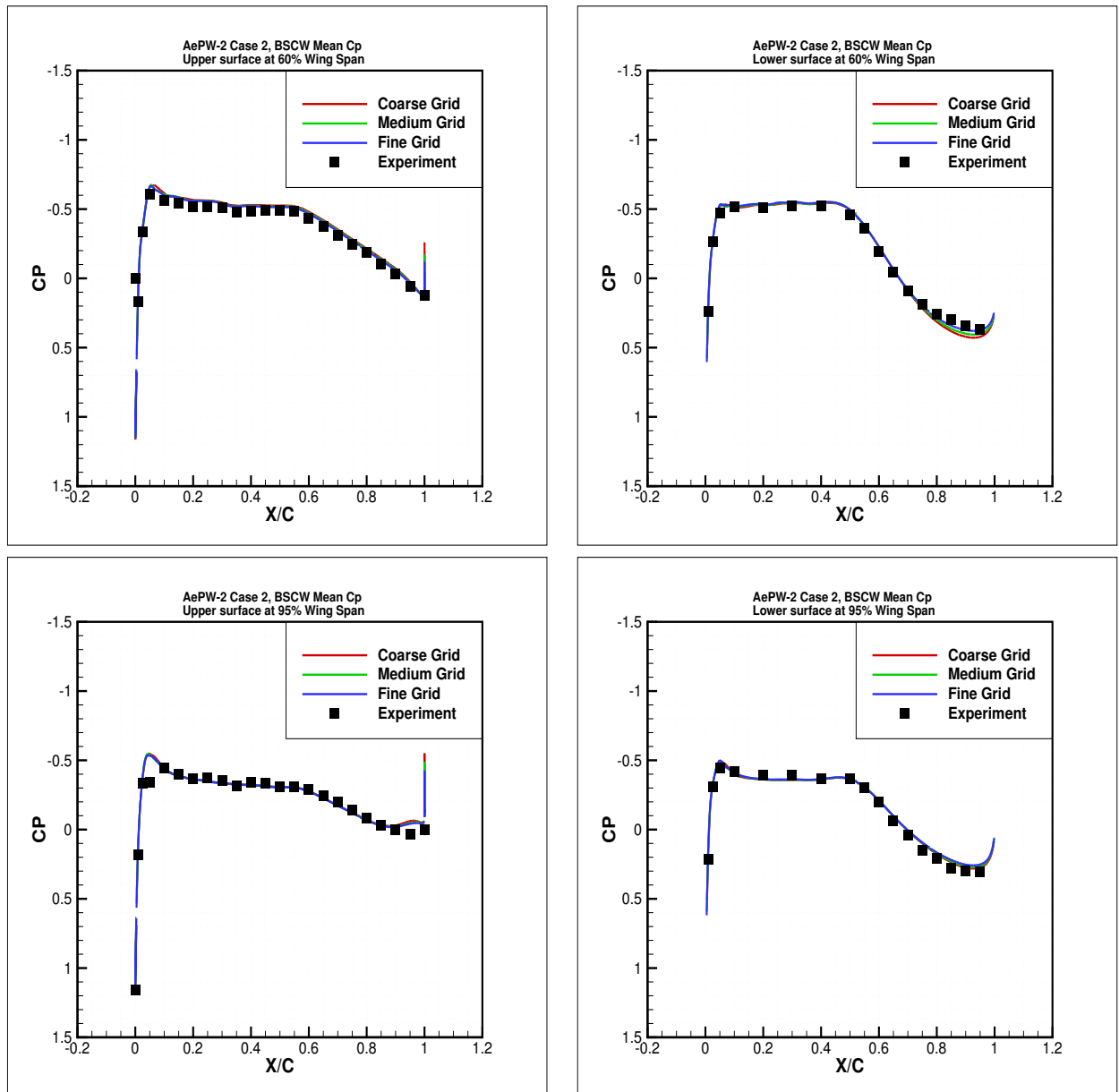
Figure B.10: Case 2 (Mach 0.74, Re = 1.09 \times 10^7 , AoA = 0^\circ ): Mean C_p for unforced system data at 60% and 95% wing span with the k - \epsilon turbulence model.
