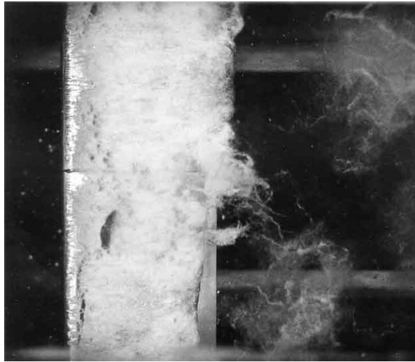
Figure 1.4: Sheet cavitation.
