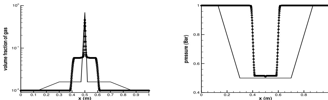
Figure 4.5: Water-air mixture expansion tube problem |u| = 2 \text{ m/s} . Void fraction and pressure profiles by central scheme with 3-equation model (symbols) and 7-equation model (solid line).
