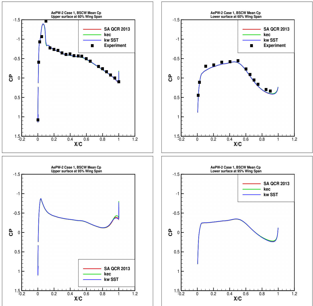
Figure B.7: Case 1 (Mach 0.7, Re = 1.12 \times 10^7 , AoA = 3^\circ ): Mean C_p for unforced system data at 60% and 95% wing span with the fine grid.
