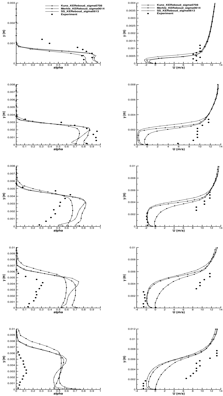
Figure 5.17: Time-averaged void ratio (left) and velocity (right) profiles from station 1 to 5 - k - \epsilon model with the Reboud correction comparison
