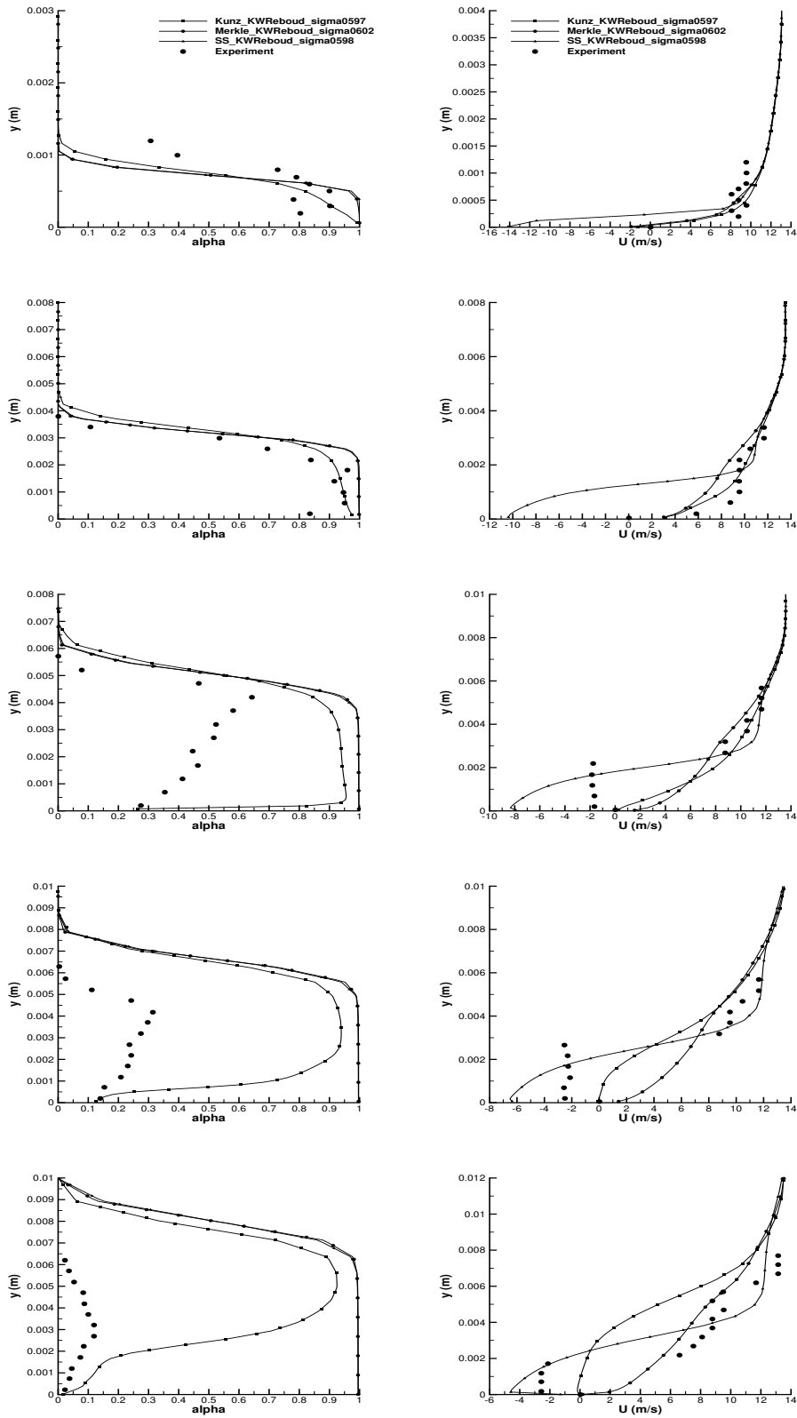
Figure 5.21: Time-averaged void ratio (left) and velocity (right) profiles from station 1 to 5 - k - \omega SST model with the Rebound correction comparison
