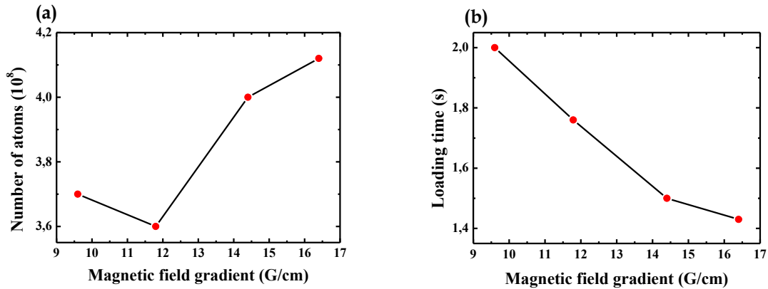
Figure 5.8: Comparison between (a) magnetic field gradient and number of atoms (b) magnetic field gradient and loading time.
