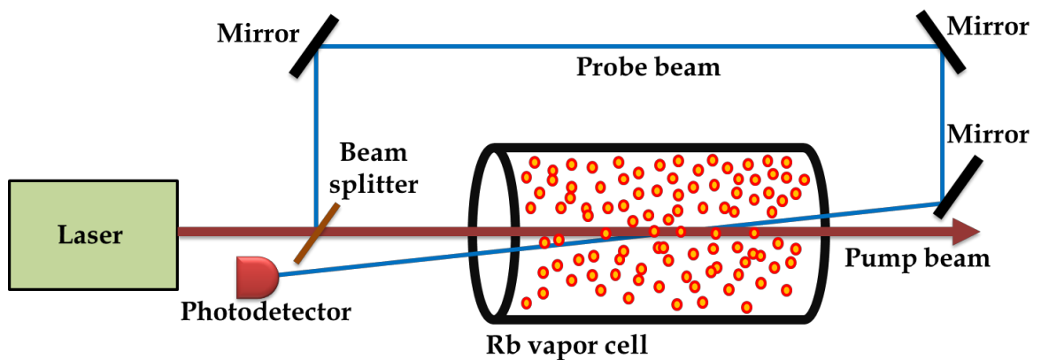
Figure 4.10: The optical layout for saturated absorption spectroscopy.
