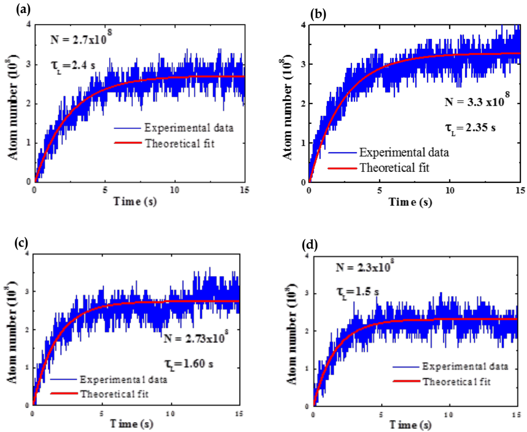
Figure 5.5: Loading curves for measurement of number of atoms of Rb^{87} at different magnetic field gradients (a) 8.8 G/cm (b) 11.8 G/cm (c) 14.4 G/cm (d) 16.4 G/cm. While laser intensity (8 mW/cm 2 ) and current for Rb source (4.5 A) are constant. The curve was fitted a function of the form equation (5.19) (red curve).
