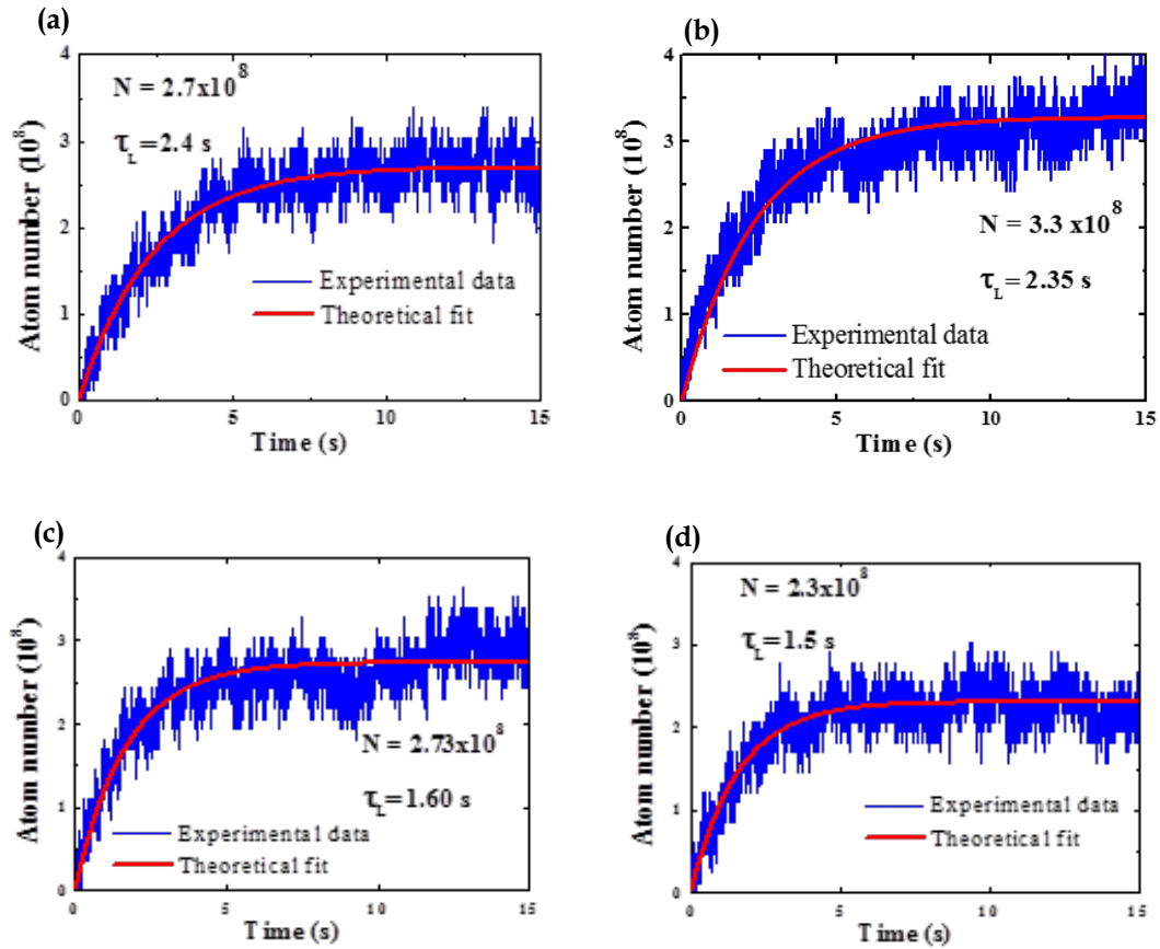
Figure 5.5: Loading curves for measurement of number of atoms of \text{Rb}^{87} at different magnetic field gradients (a) 8.8 G/cm (b) 11.8 G/cm (c) 14.4 G/cm (d) 16.4 G/cm. While laser intensity ( 8 \text{ mW/cm}^2 ) and current for Rb source (4.5 A) are constant. The curve was fitted a function of the form equation (5.19) (red curve).
