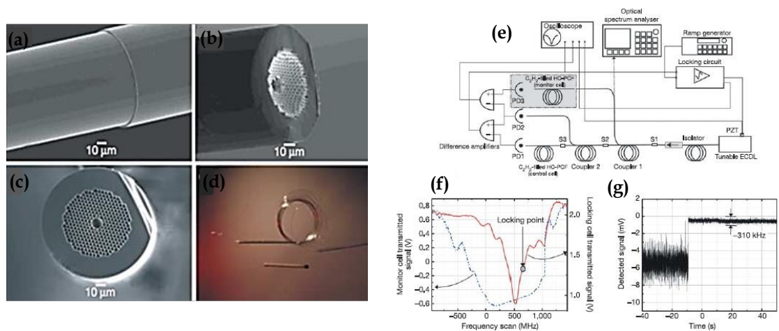
Figure 1.15: (a) Side view of splice: An HC-PCF spliced with single mode fibre (SMF) (b) End view of an HC-PCF when cleaved at the junction of the splice. (c) Shows clearly the preservation of structure when cleaved few mm from splice. Fibre is same as in (a) and (b). (d) Photograph of a 5-m-long hydrogen-filled HC-PCF gas cell. Its size is comparable with matchstick (e) frequency stabilization set up (f) small circle on red curve shows the locking point of P9 absorption line of acetylene (g) left-hand side part of trace: is frequency fluctuation when laser is free running- right-hand side part of trace: when laser is locked, exhibits maximum r.m.s frequency deviation of 310 KHz (figures taken from [14]).
