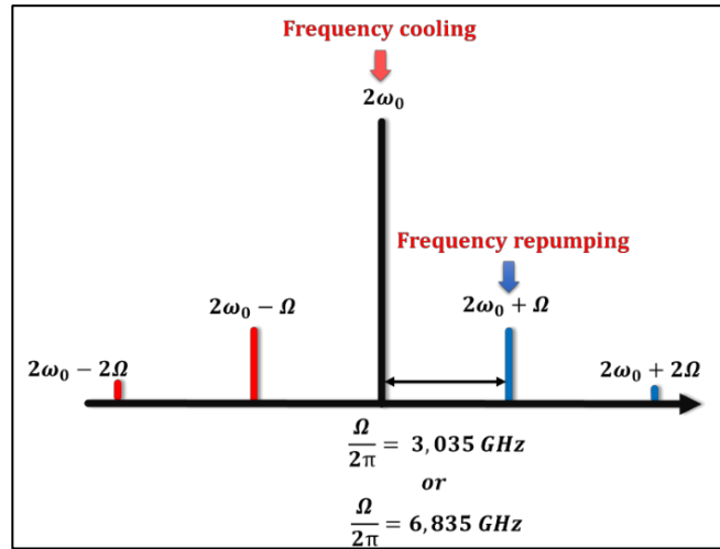
Figure 4.6: Carrier and sidebands generated after passing through the non-linear crystal.
