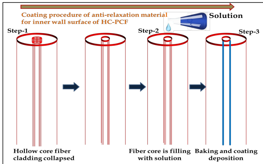
Figure 3.17: Illustration of coating procedure of the inner core wall surface of HC-PCF. In first step, cladding is collapsed, second step is about filling of solution and third step is for baking and coating deposition.
