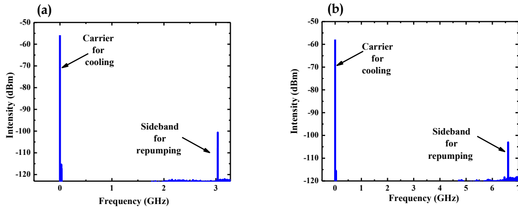
Figure 4.7: Spectra of generated sidebands (a) 3.036 GHz (b) 6.835 GHz for repumping laser for ^{85}\text{Rb} and ^{87}\text{Rb} respectively.
