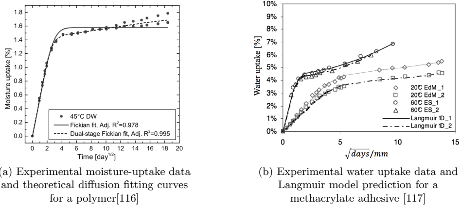
Figure 1.35: Non-Fickian behaviour
