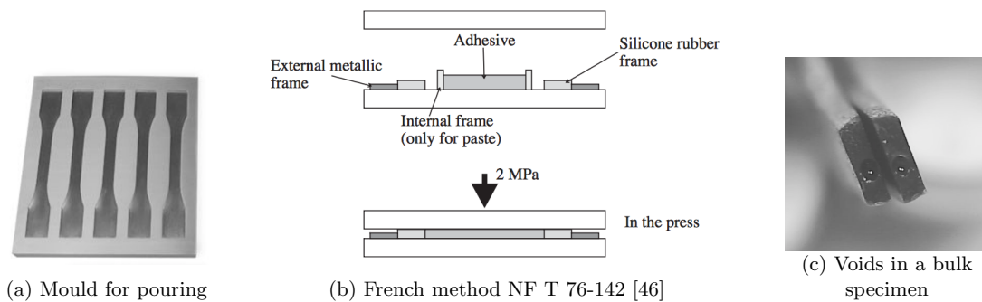
Figure 1.6: Manufacturing of bulk specimens
