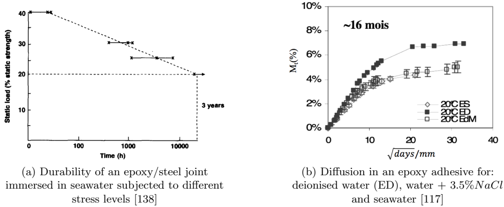
Figure 1.43: Water diffusion in an epoxy adhesive
