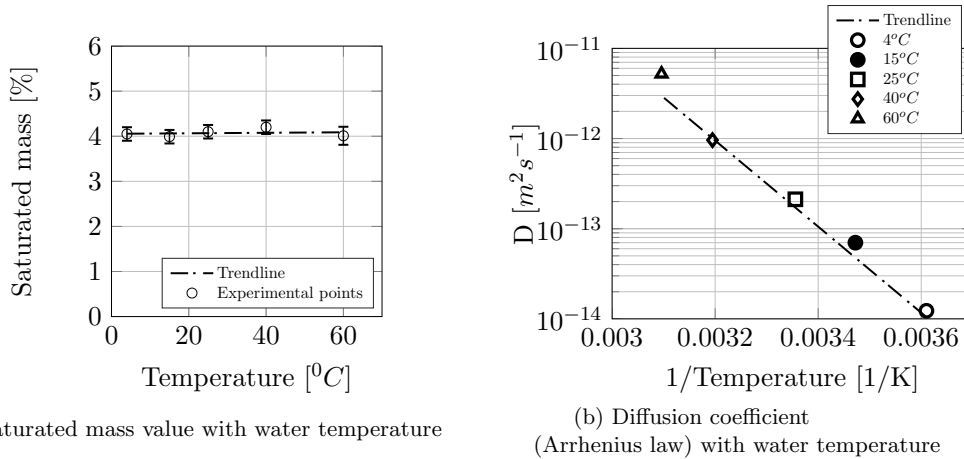
Figure 4.5: Evolution of saturated mass and diffusion coefficient with water temperature
