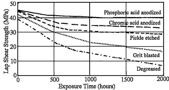
Figure 1.46: Epoxy adhesive exposed to water at 50^{\circ}C [20]
