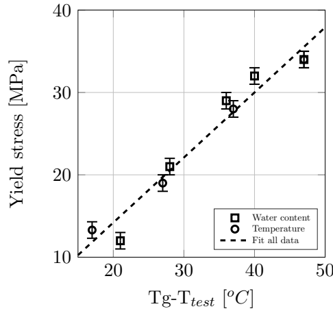
Figure 5.21: Relationship between yield stress and T_g - T_{test} obtained from tensile tests with several water contents at 21°C, and at several testing temperatures on dry specimens
