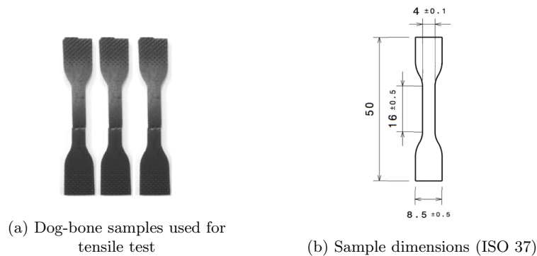
Figure 2.4: Geometry of the tensile specimens [ISO 37]
