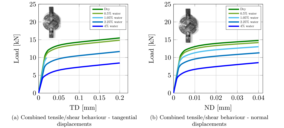
Figure 5.31: Prediction of the mechanical behaviour with the moisture dependent model
