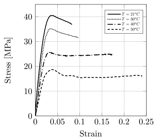
Figure 5.19: Tensile behaviour as a function of testing temperature on dry sample
