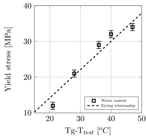
Figure 5.18: Relationship between yield stress and T_g - T_{test} obtained from tensile tests with several water contents at 21^\circ\text{C} , and at several testing temperatures on dry specimens
