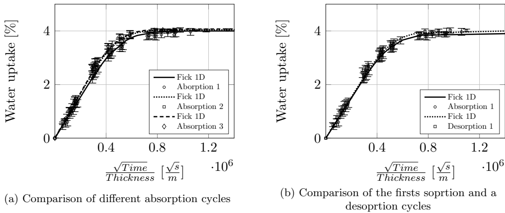
Figure 4.9: Absorption/Desorption cycles
