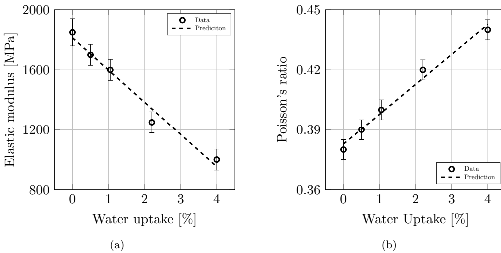
Figure 5.9: (a) Evolution of the elastic modulus with water content, (b) Evolution of Poisson's ratio with water content
