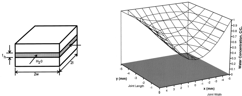
Figure 1.42: Water concentration as a function of position in a square bonded joint [19]
