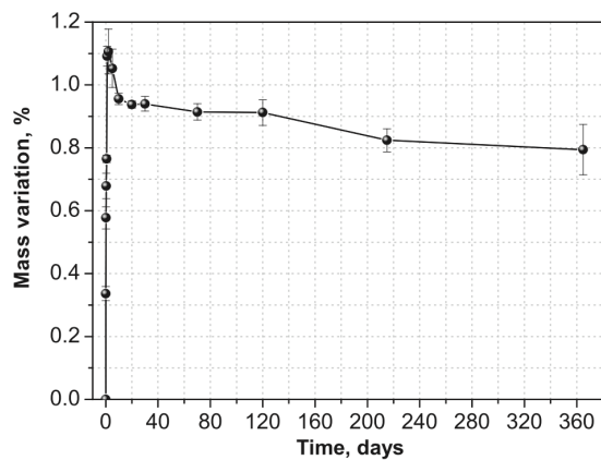
Figure 1.38: Mass variation as a function of ageing time for a polyurethane elastomer immersed in artificial seawater at 60^\circ\text{C} [16]
