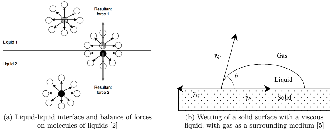
Figure 1.3: Surface energy
