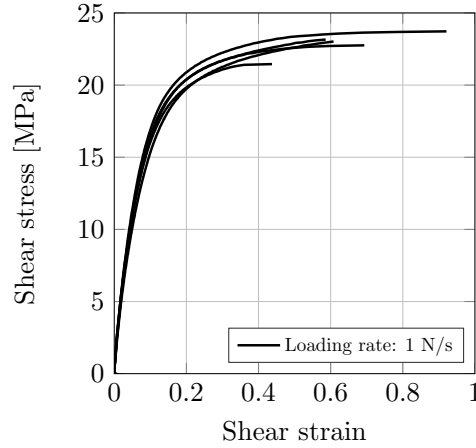
Figure 2.9: Shear behaviour on bulk specimen
