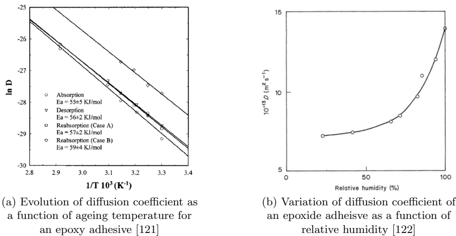
Figure 1.36: Evolution of the diffusion coefficient as a function of temperature and water activity
