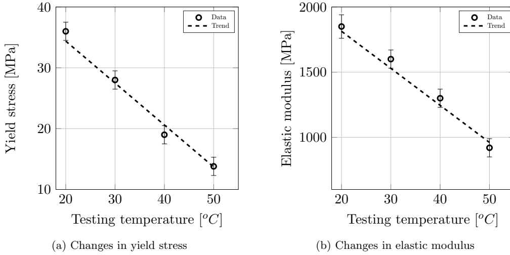
Figure 5.20: Evolution of the mechanical properties as function of testing temperature
