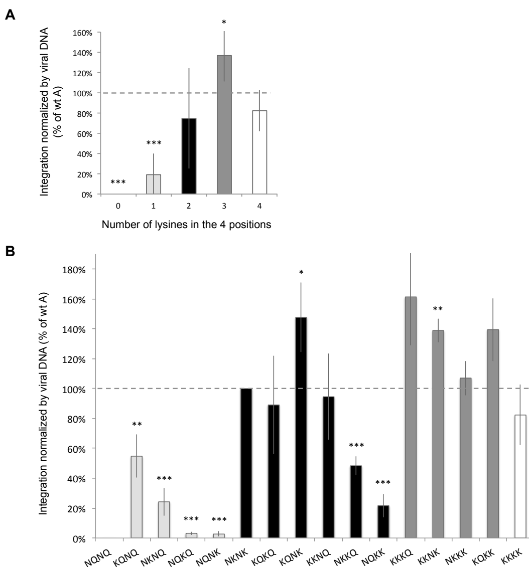
Figure 4: Panel A. Relative efficiency of integration, normalized by the amount of viral DNA, for the IN mutants grouped by the number of lysine present in the positions 222, 240, 254, 273. Panel B. Relative efficiency of integration, normalized by the amount of viral DNA, for the integrase mutants which presents 0, 1, 2, 3 or 4 K in the positions 222, 240, 254, 273. Errors bars are standard deviations. Experiments have been repeated at least 4 times. Stars represent Student statistics (NS p value>5%, * p value<5%; ** p value<1%; *** p value<0,1%).
