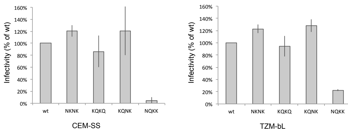
Figure 6: Infectivity of several mutations of the motif, cloned in the replicative strain PNL4-3, expressed as a percentage of the wt. Left panel. Replication-competent viruses was used to infect CEM-SS cells. The infectivity represents the percentage of infected cells compared to wt, detected by intracellular p24 staining and flow cytometry analysis. Right panel. Replication-competent viruses was used to infect TZM-bL cells. The infectivity represents the virus replication compared to wt, detected by measuring Luc reporter gene expression. The error bars represent the standard deviations of sample duplicates.
