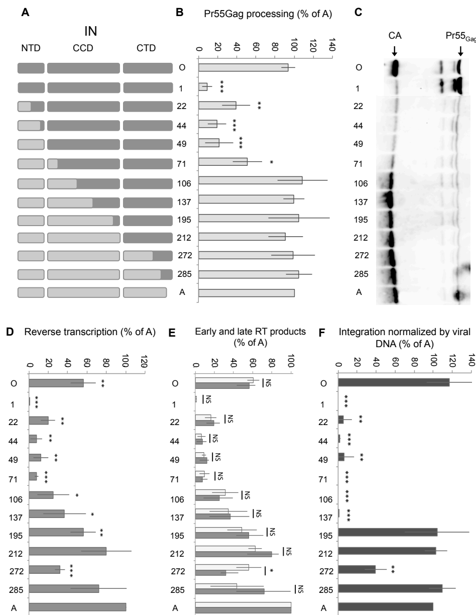
Figure 2: Functionality of viruses harbouring chimerical integrases. Panel A. Representation of the chimerical IN studied. The position of the breakpoint is given on the left, in aa from the beginning of the IN coding region. IN A is 288 aa long, while IN O is 298 aa. Panel B. Gag processing efficiency, estimated by the amount of CA compared to the amount of Gag precursors detected by Western blot. Panel C. Efficiency of reverse transcription (detection of the junction U5Ψ) for the different chimerical integrases. Panel D. Relative quantities of early (detection of the junction RU5) and late RT (detection of the junction U5Ψ) products. Panel E. Relative efficiency of integration normalized by the amount of total viral DNA, expressed as a function of A, fixed at 100%. Errors bars are standard deviations. Experiments have been repeated at least 3 times. Stars represent Student statistics. (NS p value>5%, * p value<5%; ** p value<1%; *** p value<0,1%).
