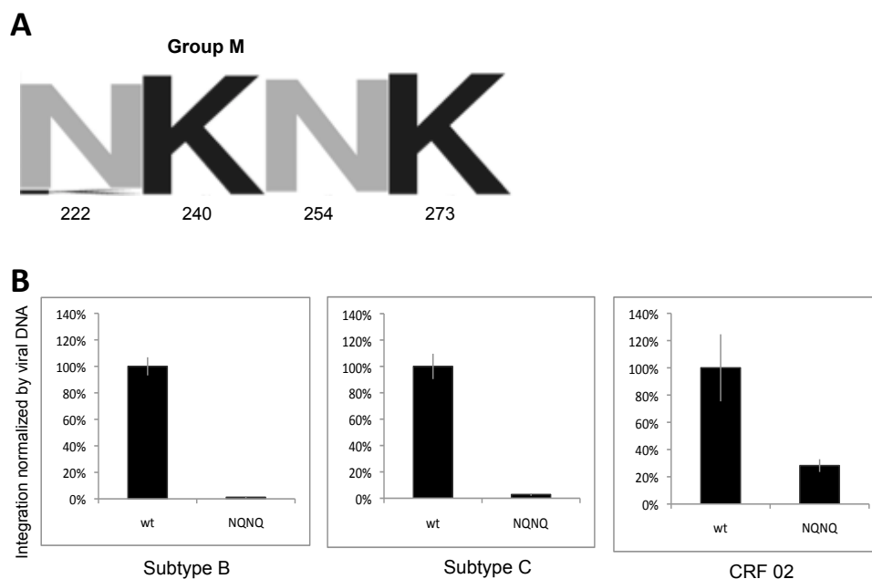
Figure 5: Panel A. Conservation logo done with the WebLogo software, http://weblogo.berkeley.edu/logo.cgi . The sequence at the positions 222, 240, 254 and 273 in group M integrases (3390 sequences from LANL database) have been aligned with CLC sequence viewer. Panel B. Relative efficiency of integration normalized by the amount of viral DNA of the mutant 0K (NQNQ) compared to the wt integrase of different group M isolates (subtype B, subtype C, CRF02). The graphic are disposed according to the phylogenetic origin of the primary isolate used, indicated below. Errors bars are standard deviations. Experiments have been repeated at least 3 times.
