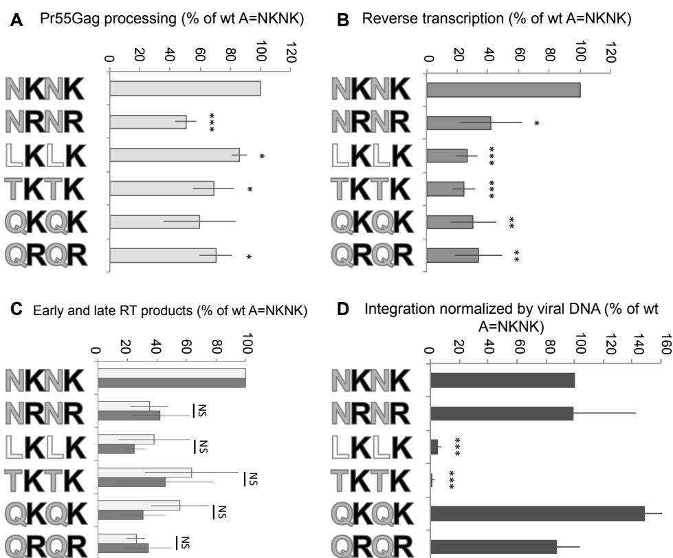
Figure 7: Panel A. Gag processing efficiency, estimated by the amount of CA compared to the amount of Gag precursors detected by Western blot, expressed as the function of the parent A, NKNK. The residue present at the four positions of the motif for each sample are indicated to the left. Panel B. Efficiency of reverse transcription (detection of the junction U5Ψ) for the different mutant integrases, expressed as a function of NKNK, fixed at 100%. Panel C. Relative quantities of early (detection of the junction RU5) and late RT detection of the junction U5Ψ) products, expressed as the function of NKNK, fixed at 100%. Panel D. Relative efficiency of integration normalized by the amount of total viral DNA, expressed as a function of NKNK, fixed at 100%. Errors bars are standard deviations. Experiments have been repeated at least 3 times. Stars represent Student statistics.
