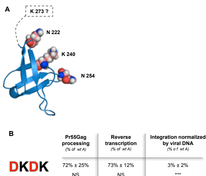
Figure 9: Panel A. Representation of the crystallographic structure of the CTD (PDB code: 1IHV). The residues 222, 240, 254 are highlight (273 is part of an unresolved tail). Panel B. Pr55Gag processing, reverse transcription and integration normalized by viral DNA for the mutant DKDK, compared to the wt A. Experience has been repeated at least 3 times, SD, Student test at one sample compared to the value of A. (NS p value>5%, * p value<5%; ** p value<1%; *** p value<0,1%).
