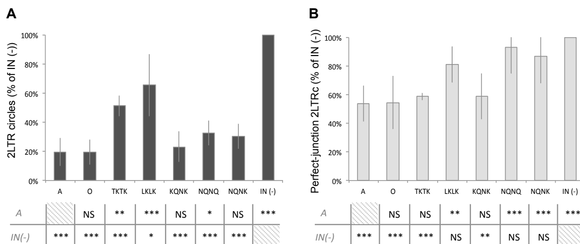
Figure 8: Panel A. Percentage of 2 LTR circles compared to total viral DNA, expressed as a percentage of the catalytic mutant IN A (mutation D 116 A), called IN(-), fixed at 100%. The table under the graphic contains the symbols that reflected the p value of a Student test compared to the parental IN A (top line) or the IN D 116 A (bottom line). Panel B. Percentage of perfect-junction 2LTRc expressed as a function of the total amount of 2LTRc, reported to IN(-), fixed at 100%. The table under the graphic contains the symbols that reflected the p value of a Student test compared to the parental IN A (top line) or the IN D 116 A (bottom line). The experiments have been repeated at least three times. Error bars are standard déviations. NS p value>5%, * p value<5%; ** p value<1%; *** p value<0,1%.
