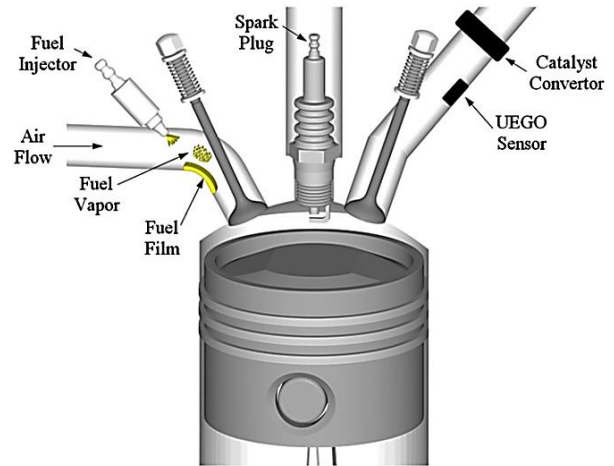
Fig. 52. Scheme of the different elements and phenomenon involved in the fuel path in (Ebrahimi et al., 2012)
