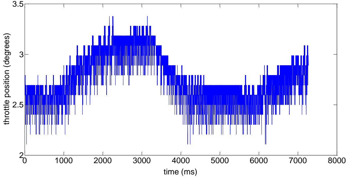
Fig. 63. Measure of the throttle position from the engine test bench
