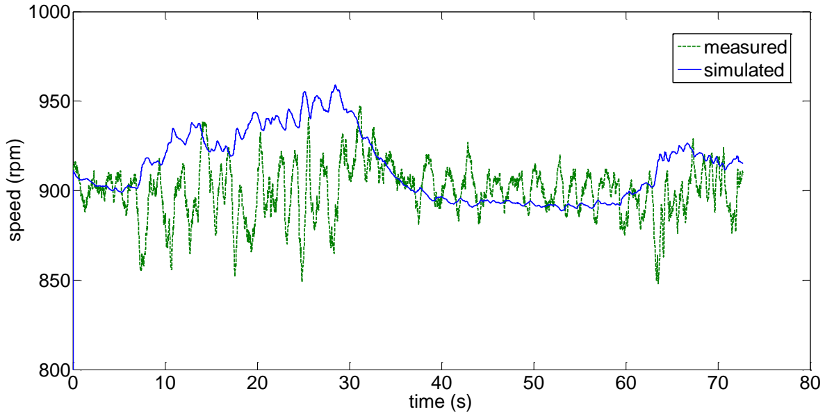
Fig. 69. Validation of the rotational dynamics model
