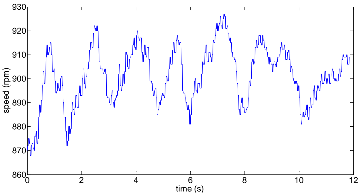
Fig. 94. Idle speed control with maps-based air-fuel ratio control
