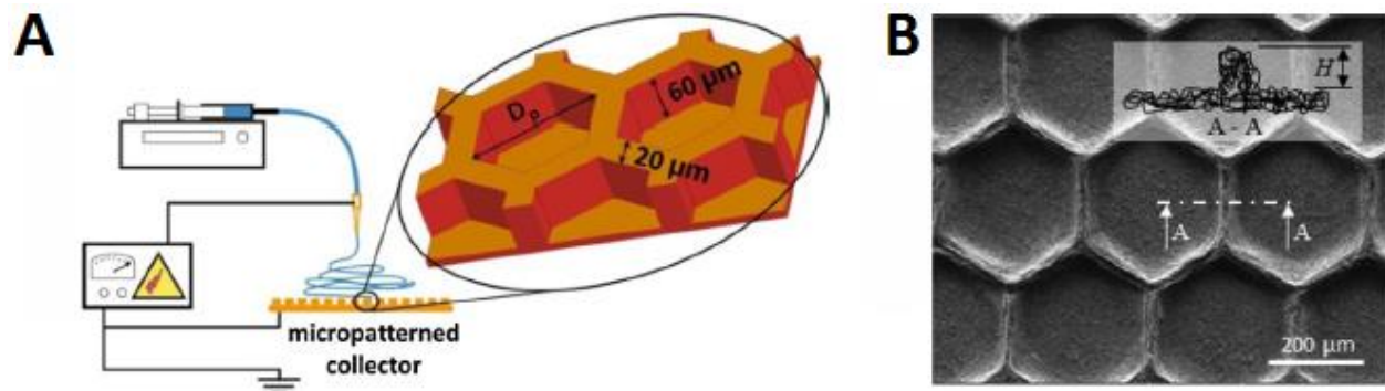
Figure 21. (A) Principle of electrospinning on micro-patterned honeycomb collectors with D_p=40 , 80 , 160 , and 360 \mu\text{m} . (B) SEM image of a PCL honeycomb scaffold obtained with D_p=360 \mu\text{m} (Nedjari et al., 2014).
