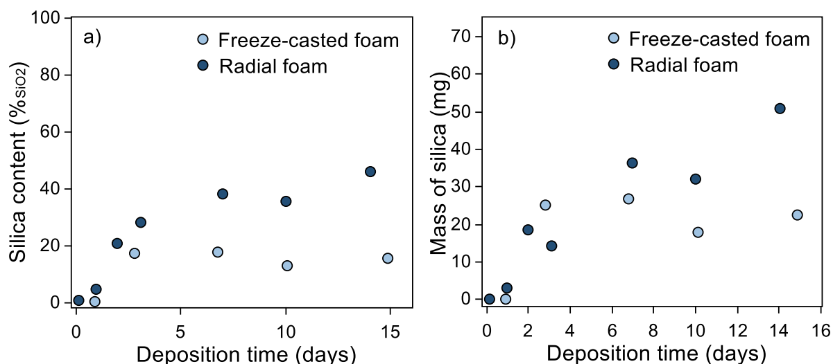
Figure III.5: Plateau in the silica content can be observed on both freeze-casted and radial foams (a). The final deposited mass is higher for radial foams (b).
