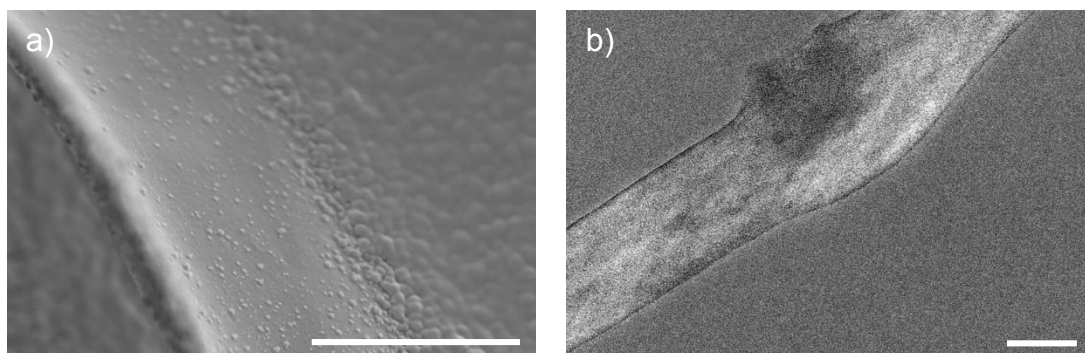
Figure III.14: Non-percolating silica layers (a) or defects in the silica layer may result in dissolution and leaching of the pectin pore wall. Scale bars: 2 \mu\text{m} for a and 200 nm for b.
