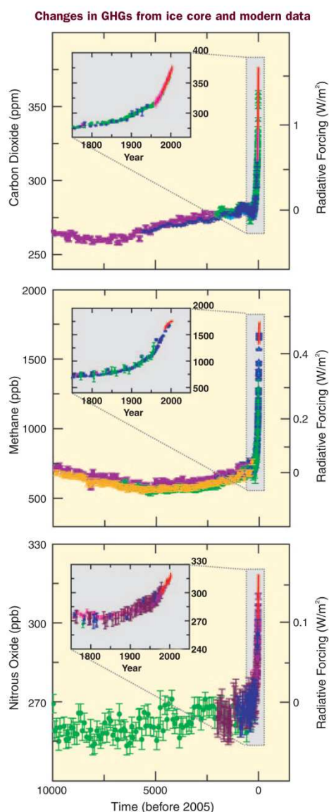
Figure 1: Atmospheric concentrations of \text{CO}_2 , \text{CH}_4 and \text{N}_2\text{O} over the last 10,000 years (large panels) and since 1750 (inset panels). Measurements are shown from ice cores (symbols with different colors for different studies) and atmospheric samples (red lines). The corresponding radiative forcings relative to 1750 are shown on the right hand axes of the large panels. Source: (Bernstein et al. 2007)
