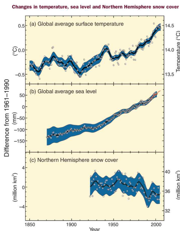
Figure 2: Observed changes in (a) global average surface temperature; (b) global average sea level from tide gauge (blue) and satellite (red) data; and (c) Northern Hemisphere snow cover for March-April. All differences are relative to corresponding averages for the period 1961-1990. Smoothed curves represent decadal averaged values while circles show yearly values. The shaded areas are the uncertainty intervals estimated from a comprehensive analysis of known uncertainties (a and b) and from the time series (c). Source: (Bernstein et al. 2007)
