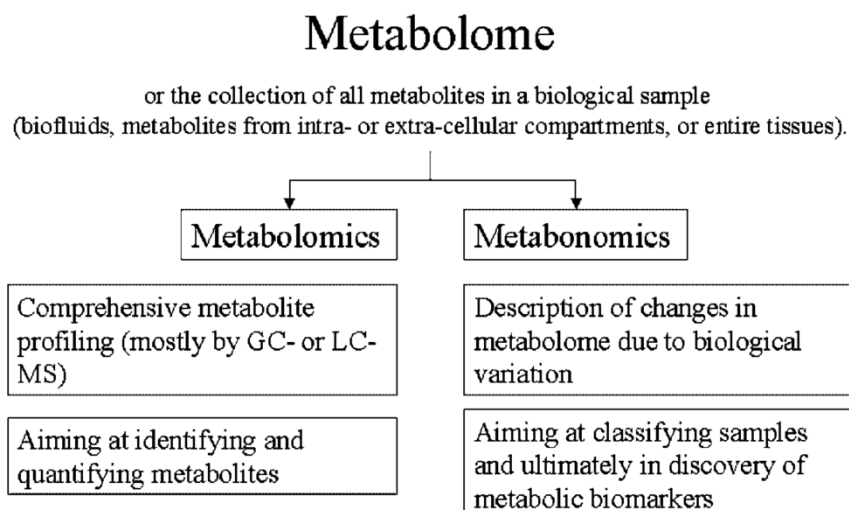
Figure 16: Goals for metabolome investigations. Strategies to tackle metabolome depend on the goal of the investigator: quantitative analyses are called the metabolomic approach, whereas classification of samples and biomarker discovery are referred to as metabonomic studies.
