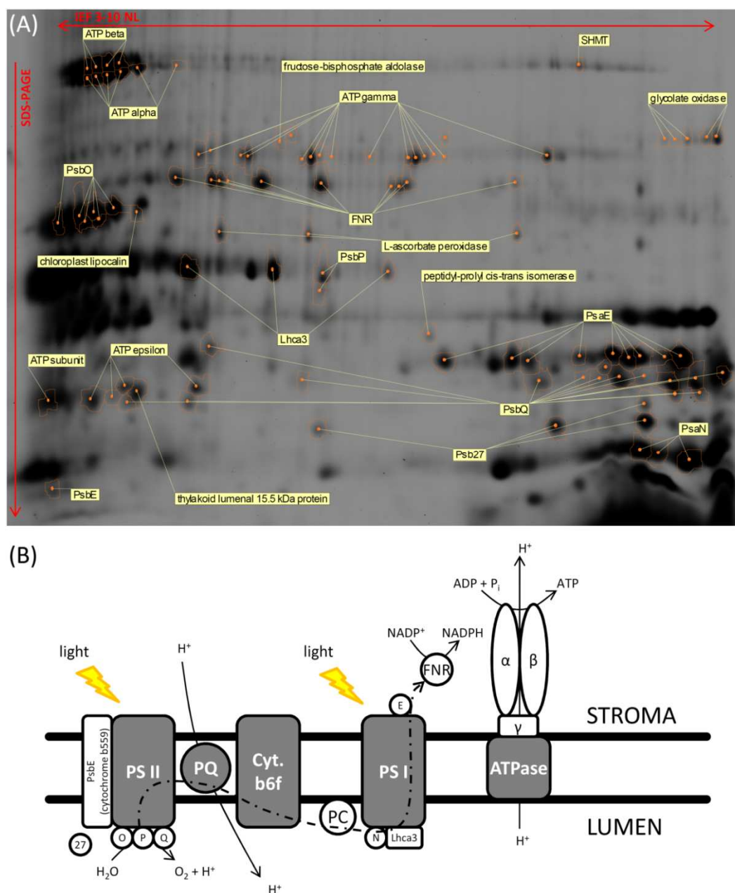
Figure 29: (A) Cy2 gel view with identified protein spots in orange. Horizontal separation was done by IEF 3-10 NL, vertical separation by SDS-PAGE as described in 3.2.3. Material and methods. (B) Representation of the chloroplast electron transport chain and the positions of the subunits that vary due to ozone exposure. White elements represent all the identified subunits that vary due to ozone, gray elements regroup the remaining subunits of the electron transport chain. Abbreviations: 27, O, P, Q = Psb27, PsbO, PsbP, PsbQ; N and E = PsaN, PsaE; PQ = plastoquinone, PC = plastocyanin, Cyt. B6f = cytochrome b6f, FNR = ferredoxin-NADP + oxidoreductase. Dashed line: electron transport path.
