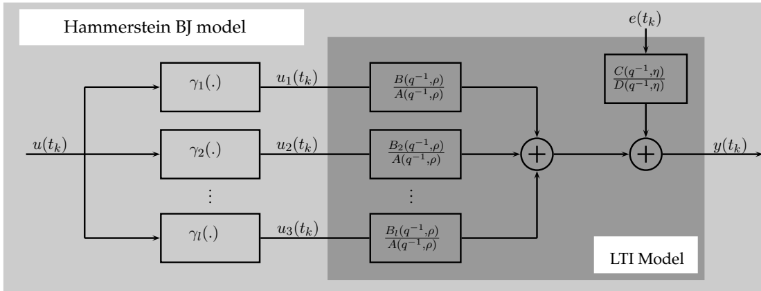
FIG. 2.2 – Hammerstein augmented model
