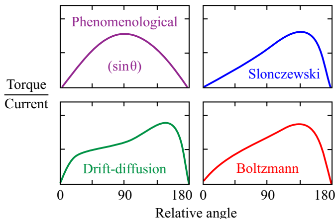
Figure 3.3 – Angular variation of the spin torque in various approaches.
