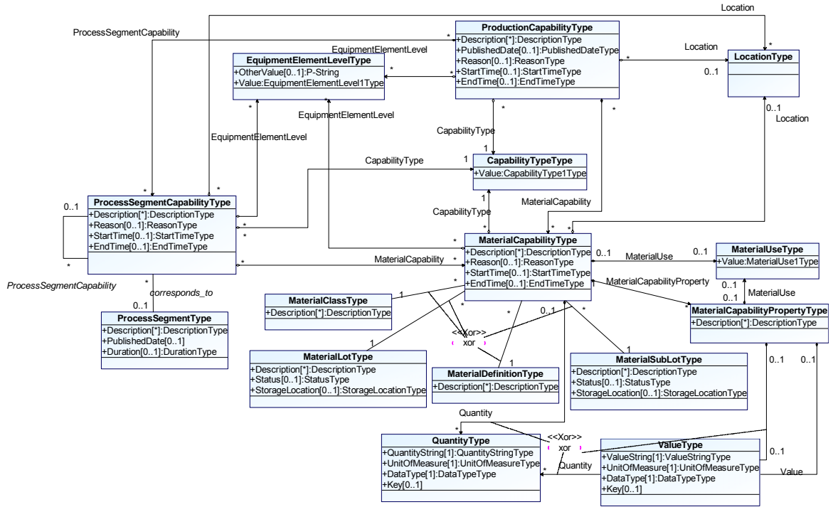
Figure 14 (a) - B2MML schemas definitions for production capability
