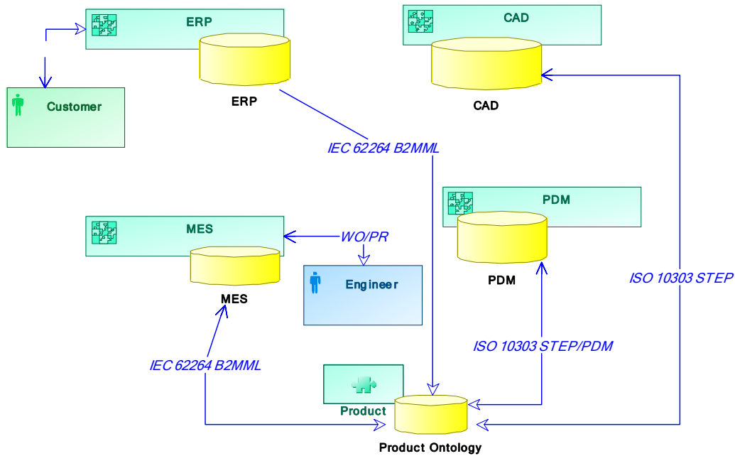
Figure 4 – Product-driven interoperability architecture
