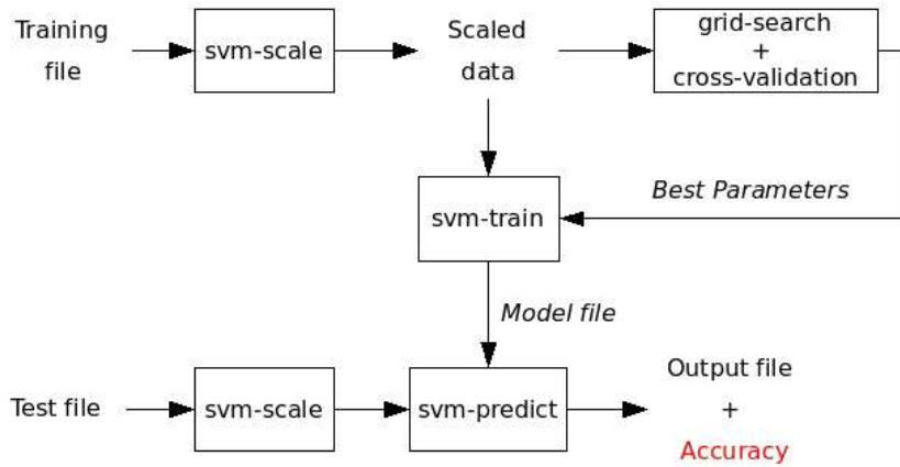
Figure 8.1: SVM flow chart
