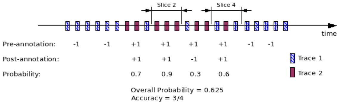
Figure 8.6: Attack detection in a mixed trace
