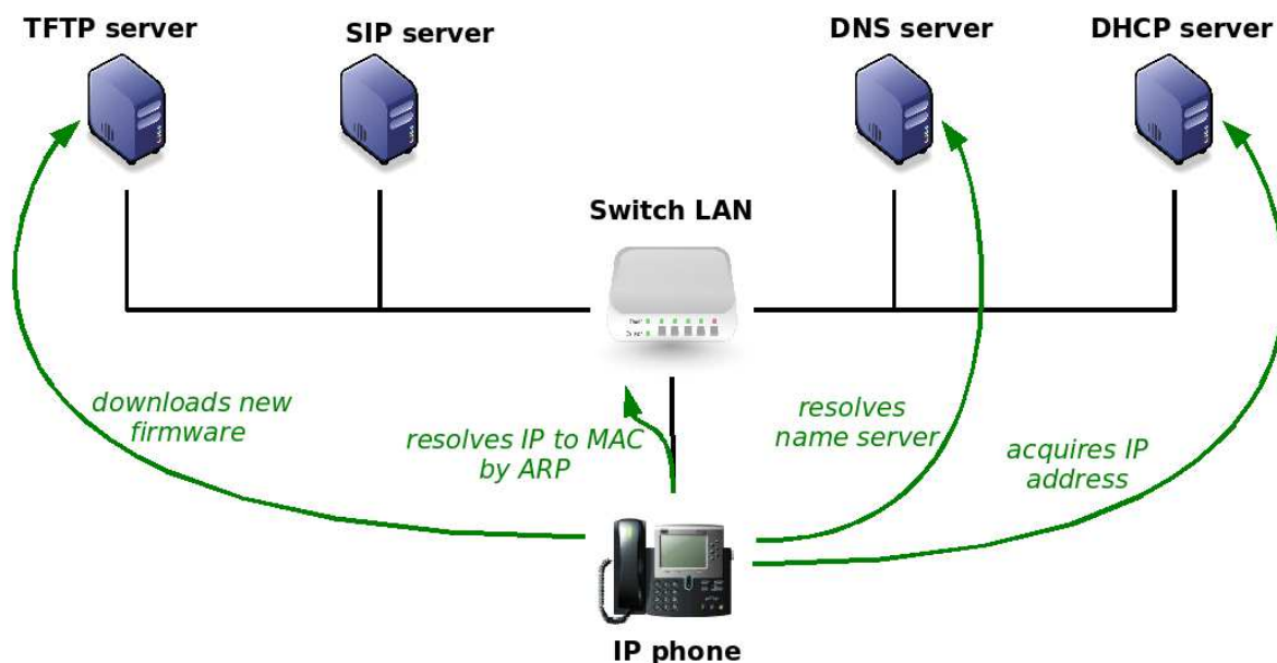
Figure 2.2: Supporting services for a SIP UA
