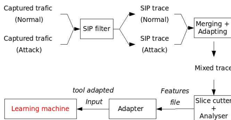
Figure 8.3: Data pre-processing flow chart
