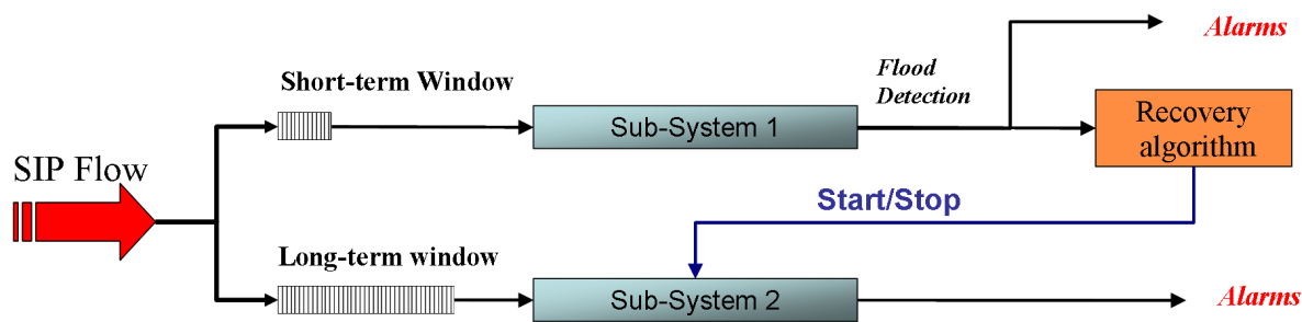
Figure 4.3: Short-term/long-term SIP traffic monitoring system
