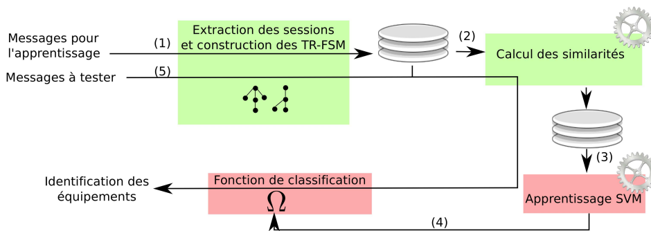
FIGURE 6.5 – Fingerprinting comportemental supervisé
