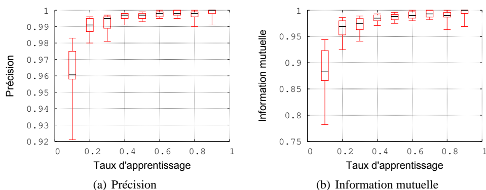
FIGURE 9.4 – Fingerpringing syntaxique supervisé, distance d_3
