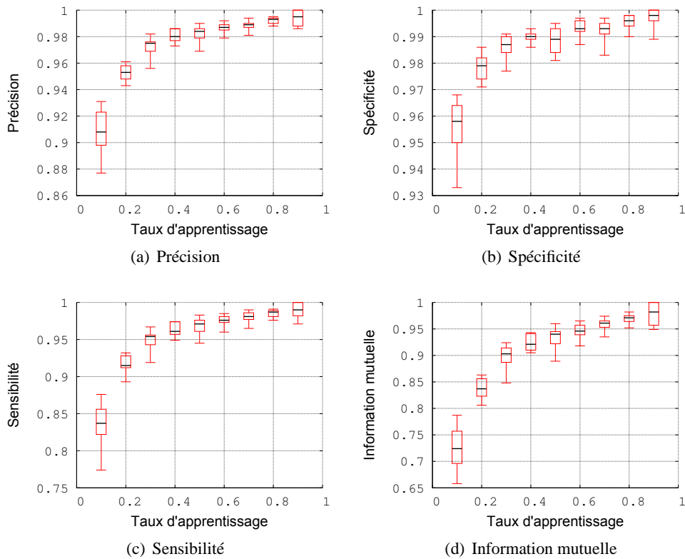
FIGURE 9.3 – Fingerprinting syntaxique supervisé, distance d_1
