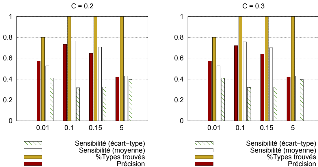
FIGURE 8.10 – SVC - SMTP dataset
