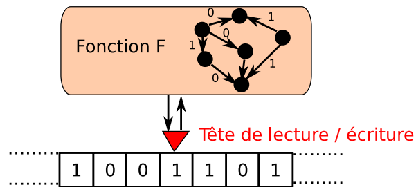
FIGURE 1.1 – Machine de Turing
