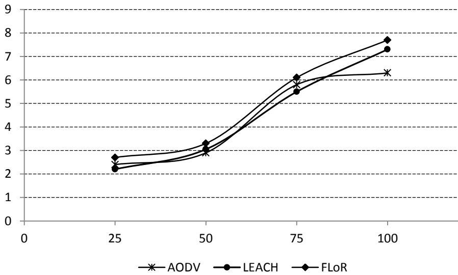
Figure 21. Throughput comparison
