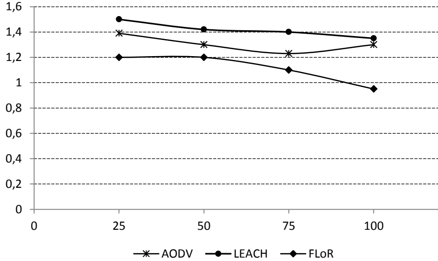
Figure 22. Routing overhead comparison
