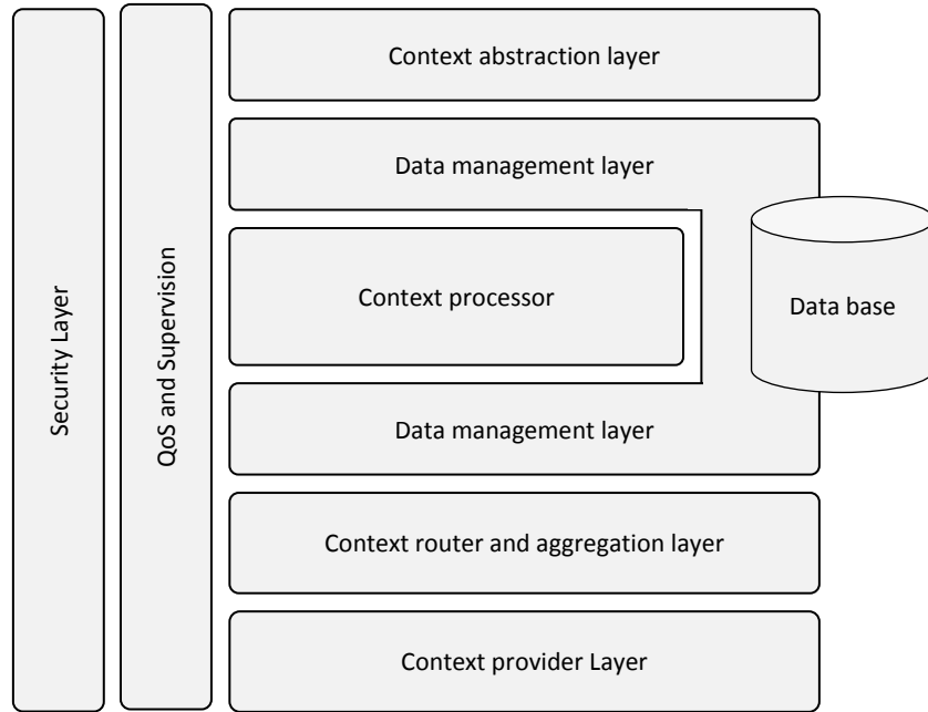
Figure 26. Reference model
