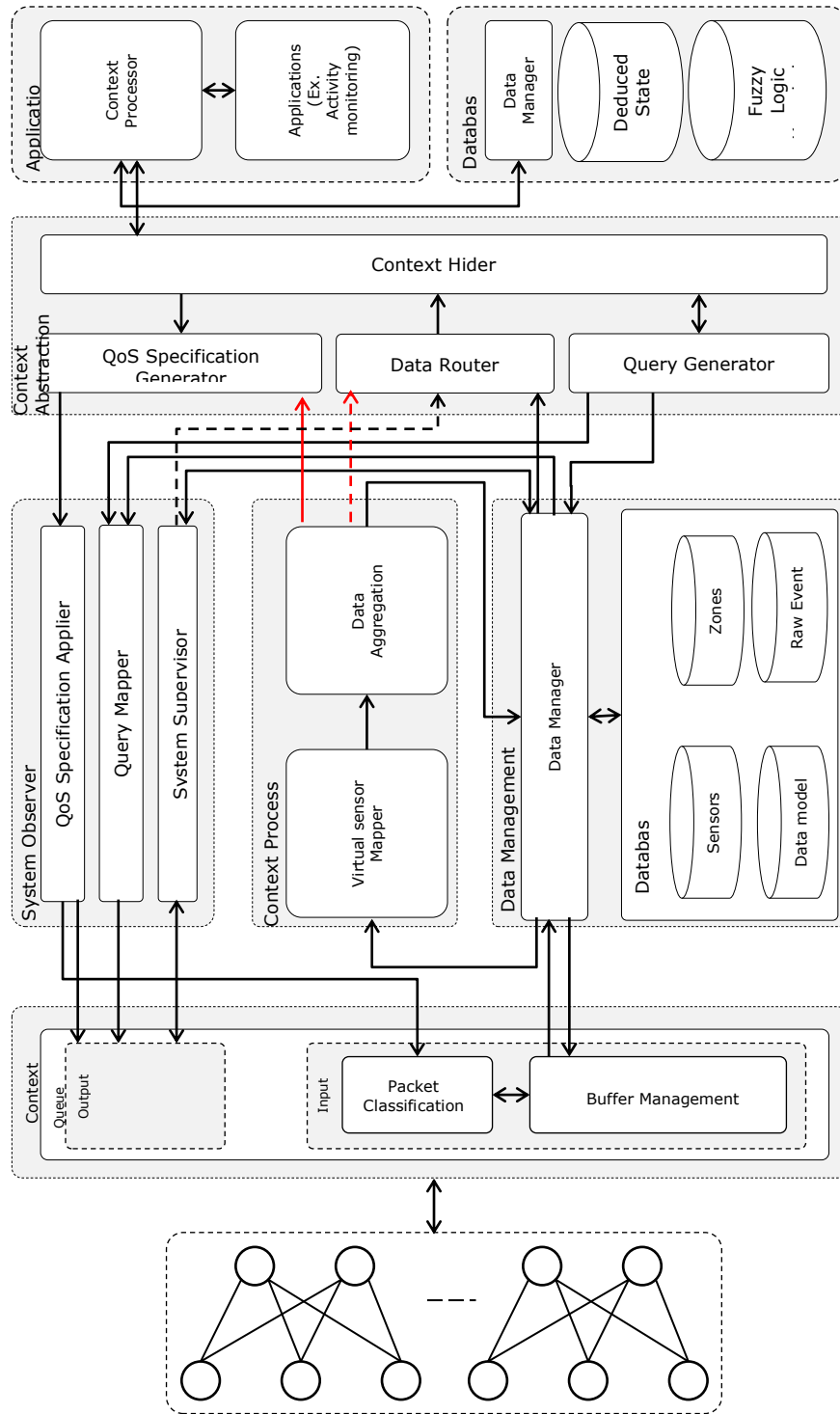
Figure 36. Modified architecture
