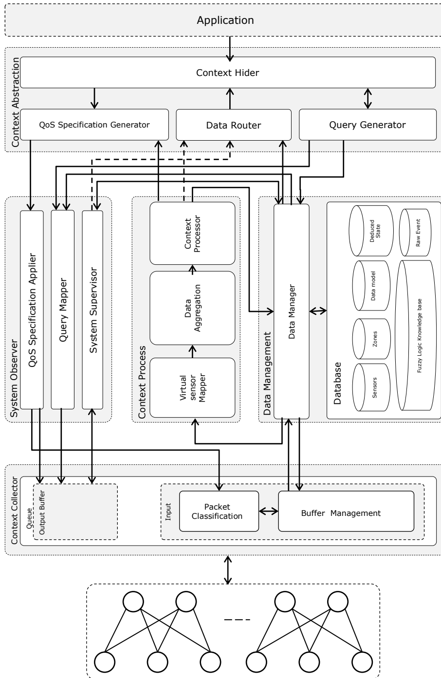
Figure 29. Middleware architecture
