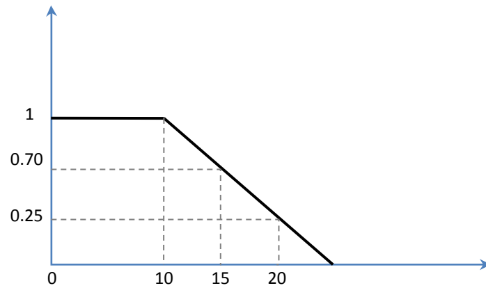
Figure 57. fuzzy set for “near” distance
