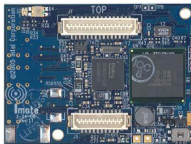
Figure 66. Imote2 sensor board
