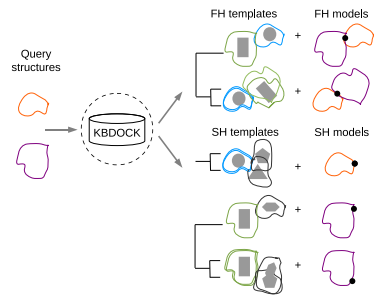
Figure 3. Schematic illustration of how KBDOCK processes a docking query. Here, dots represent the calculated binding site centre residues. When a FH template is available, KBDOCK superposes the query domains onto the template to propose a docking model. When only SH templates exist, KBDOCK proposes one or more binding site(s) on each query domain. For each selected template, KBDOCK calculates the core, rim, and binding site centre residues.
