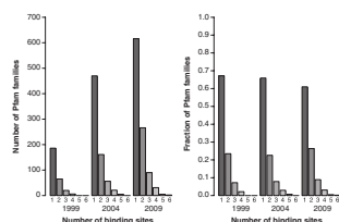
Fig. 5. The calculated number of hetero binding sites per domain family by PDB deposition date for all Pfam families except the C1-ser immunoglobulin domains.
