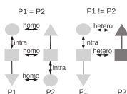
Fig. 2. Schematic illustration of the different types of DDI that may occur between two protein chains, P1 and P2. Protein chains can contain one or more domains connected by linker regions (straight lines). Each shape (circle, rectangle, triangle) represents a different Pfam domain. Lines with arrowheads represent DDIs.
