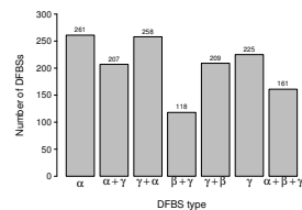
Fig. 1. The distribution of DFBSs over the 7 selected binding site types.
