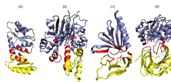
Fig. 2. Examples of different types of DFI: (a) \alpha with \alpha (PDB code 1VRC, chains A, C); (b) \alpha + \gamma with \alpha (PDB code 2CG5, chains A, B); (c) \beta + \gamma with \gamma (PDB code 2YIB, chains F, B); (d) \gamma + \alpha with \gamma + \beta (PDB code 1TE1, chains A, B). Binding site SSEs are shown in red.
