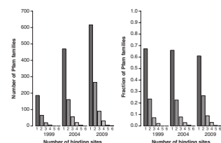
Fig. 5. The calculated number of hetero binding sites per domain family by PDB deposition date for all Pfam families except the C1-ser immunoglobulin domains.
