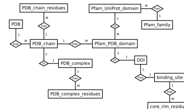
Figure 2. A simplified view of the entity-relationship diagram of the KBDOCK database.
