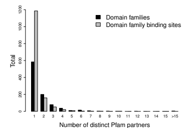
Fig. 3. Histogram of the number of different Pfam domain partners by Pfam domain and by DFBS.
