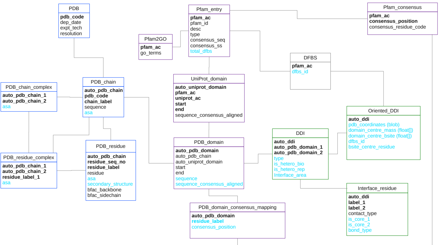
Figure 3.9: A relational data model of the KBDOCK database. Attributes which we calculated are in cyan. The DFBS entity is described in Chapter 4.
