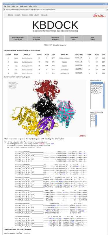
Figure 5. A screenshot of the KBDOCK results for the query domain family, Kunitz_legume. The results page consists of four sections: (i) a non-redundant list of hetero DDIs grouped by their binding site, (ii) a Jmol view of the DDIs in the coordinate frame of the query domain (the query domain is shown in black and interface residues are shown in wireframe), (iii) a Pfam consensus-based sequence alignment of the domains annotated with the core (green), rim (blue), and centre (red) binding site residues, (iv) a link to download the superposed PDB files as a single compressed file for further analysis.
