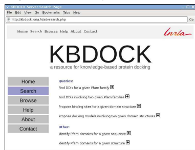
Figure 4. A screenshot of the KBDOCK "Search" page.
