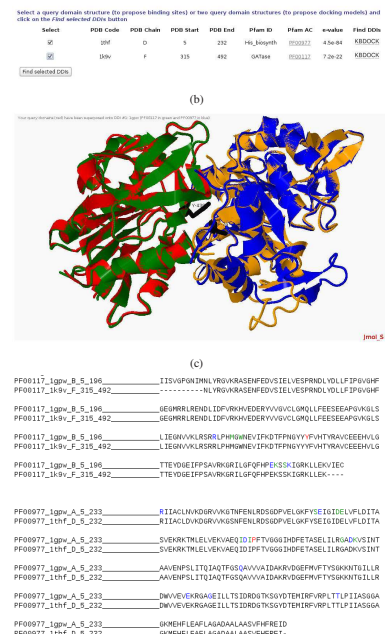
Figure 6. A screenshot showing (a) the selection of two domains for which a docking model is requested, (b) a Jmol view of the resulting FH template with the query domains superposed onto the template, (c) sequence alignments of the query and template domains highlighting the template core, rim, and centre binding site residues.
