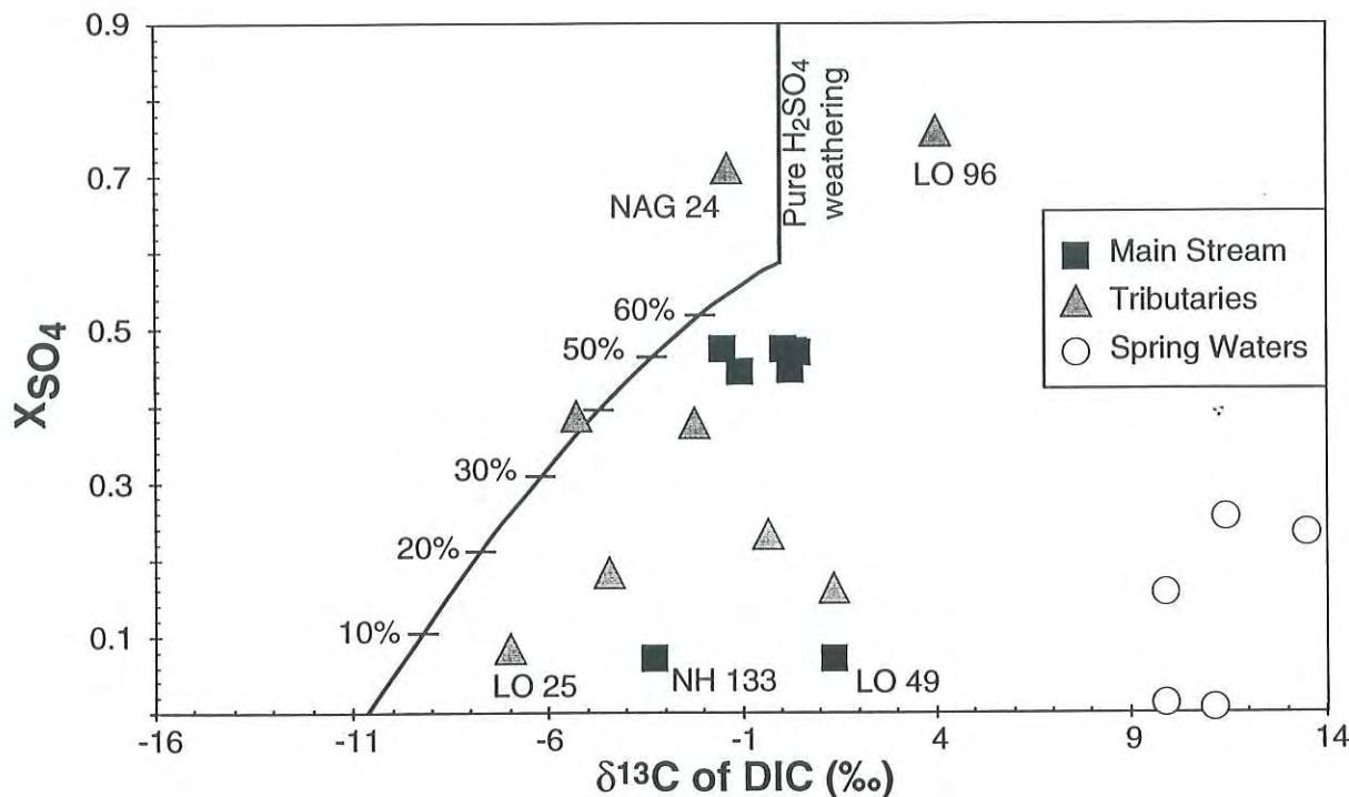
Fig. 6a : Plot of \delta^{13}\text{C}_{\text{DIC}} versus X_{\text{SO}_4} in the Kali Gandaki head waters. Data for thermal springs sampled near the river show high \delta^{13}\text{C} values, implying a metamorphic origin for the \text{CO}_2 . The mixing curve corresponds to the alteration by sulphuric acid and respired carbonic acid of 70% of carbonate and 30% of silicate. The fact that rivers plot to the right of the mixing curve implies that \text{CO}_2 rich in ^{13}\text{C} is involved in the alteration reaction in addition to biologic \text{CO}_2 . The contribution of metamorphic \text{CO}_2 dissolved in ground water as sampled in thermal springs is clearly identified at several locations.
