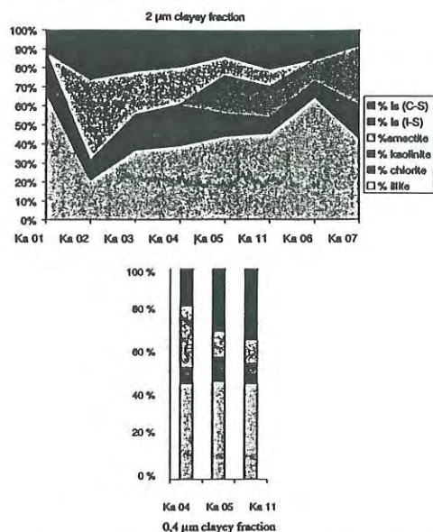
Fig. 6: Clay mineralogy through the shear zone. a : for the <2 \mu\text{m} fraction; b : for the <0.4 \mu\text{m} fraction.
