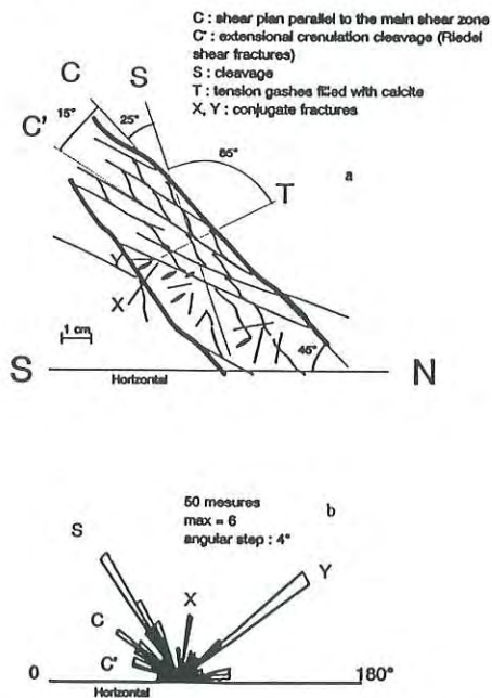
Fig. 2: Typical pattern observed at outcrop along the main Karnali shear zone. (a): main tectonic features; (C): shear plane parallel to the shear zone boundary; (C'): Extensional crenulation cleavage (Riedel shear fractures), (S): cleavage and (T): tension gashes filled with calcite. b: statistical analysis of the distribution of the fractures and cleavage.
