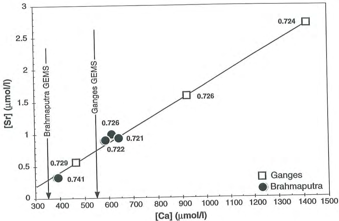
Fig. 10 : Ca versus Sr concentration relationship for Ganges (square) and Brahmaputra (circle) near their mouth. Data are from this study, Palmer and Edmond (1989); Sarin et al., (1989). ^{87}\text{Sr}/^{86}\text{Sr} values for each sample are indicated. During the monsoon, waters are more radiogenic and less concentrated. Based on this relationship and on the [Ca] yearly average given by the GEMS water program (arrows), average [Sr] for the Ganges and Brahmaputra should be 0.75 and 0.2 \mu\text{mol/l} respectively.
