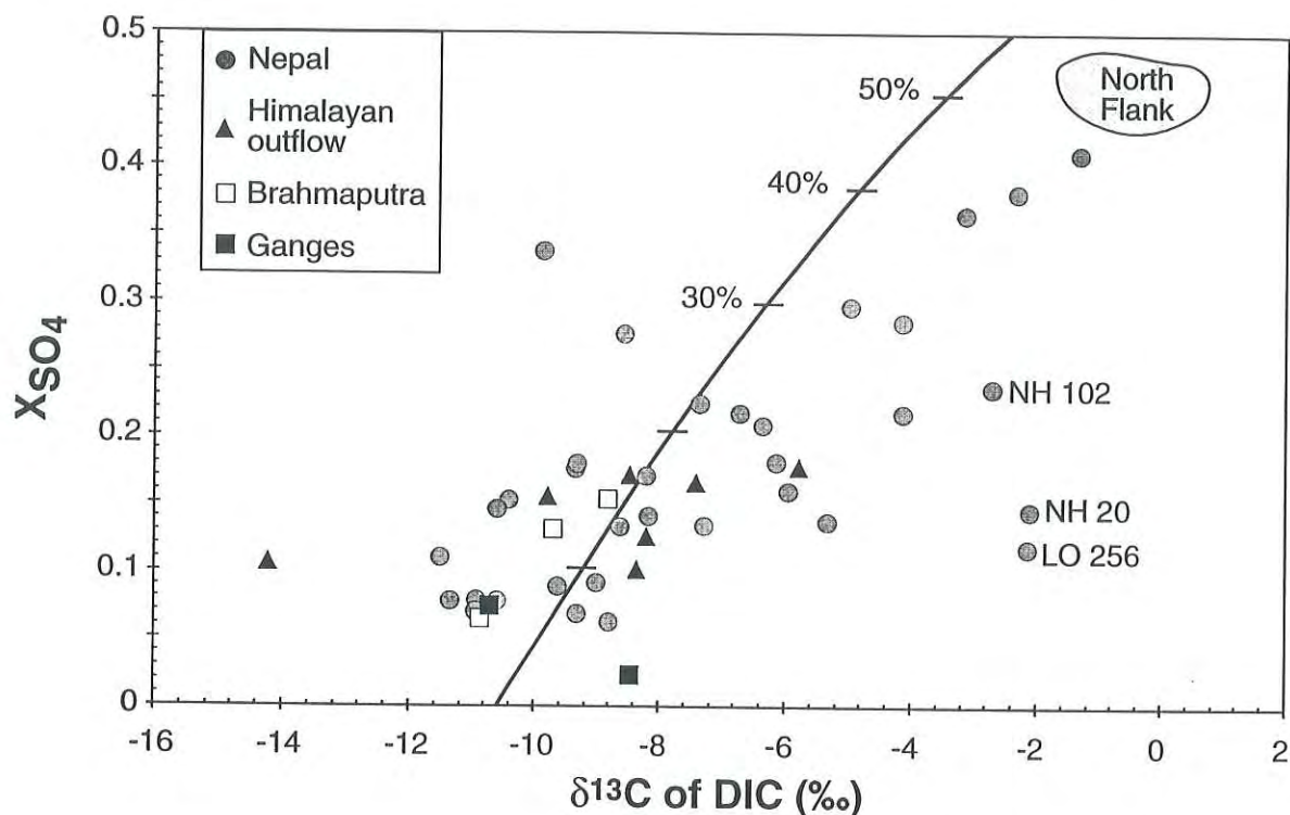
Fig. 6b : Plot of \delta^{13}C_{DIC} versus X_{SO_4} for main Himalayan rivers, Ganges and Brahmaputra. The mixing trend corresponds to the alteration by sulphuric acid and biologic carbonic acid of 70% of carbonate and 30% of silicate. Most samples are compatible with a model of alteration driven by soil CO_2 mixed with variable proportion of H_2SO_4 . The 3 labelled samples are close to the MCT, where spring waters are known and may locally influence the TDS.
