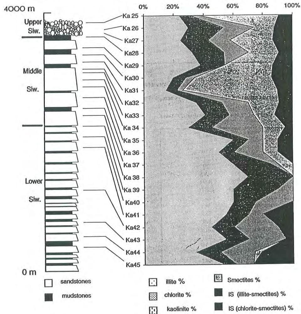
Fig. 8: Clay mineralogy for the Siwalik sediments sampled along the Karnali River.
