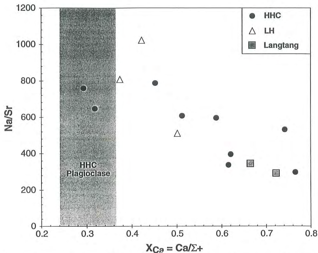
Fig 6 : Variation of dissolved Na/Sr molar ratio with X_{Ca} (eq%) for rivers draining basin of silicate composition (except Langtang samples). All data are corrected for rain water contribution. Dissolution of discrete carbonate present in altered formations is sufficient in some cases to significantly increase X_{Ca} and [Sr]. The shaded zone indicate X_{Ca} value for HHC plagioclase after Brouand (1989).
