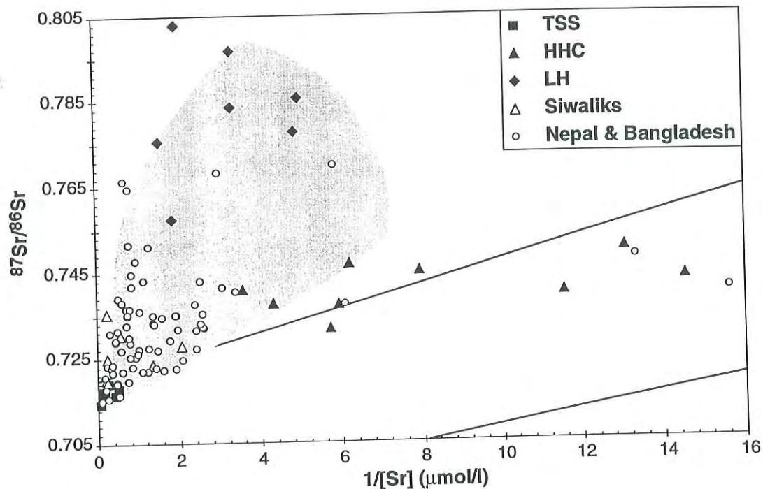
Fig 3 : Isotopic composition of dissolved Sr versus 1/[\text{Sr}] . Samples with watershed in the TSS, HHC, LH and Siwaliks are individualised. All other samples are rivers combining drainage of several geological formations in Nepal and Bangladesh. The shaded area corresponds to published data for Himalayan tributaries of G-B (Palmer and Edmond, 1992 ; Krishnaswami et al., 1992 ; Trivedi et al., 1995 ; Harris et al., 1998). The two lines bracket the riverine composition of dissolved Sr in other major world rivers (after Edmond, 1992).
