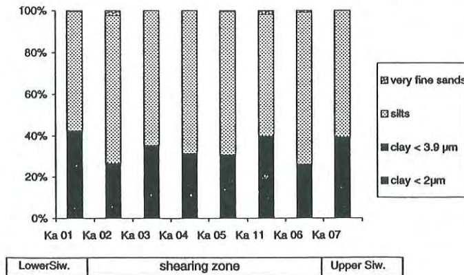
Fig. 4: Grain-size analysis through the shear zone.
