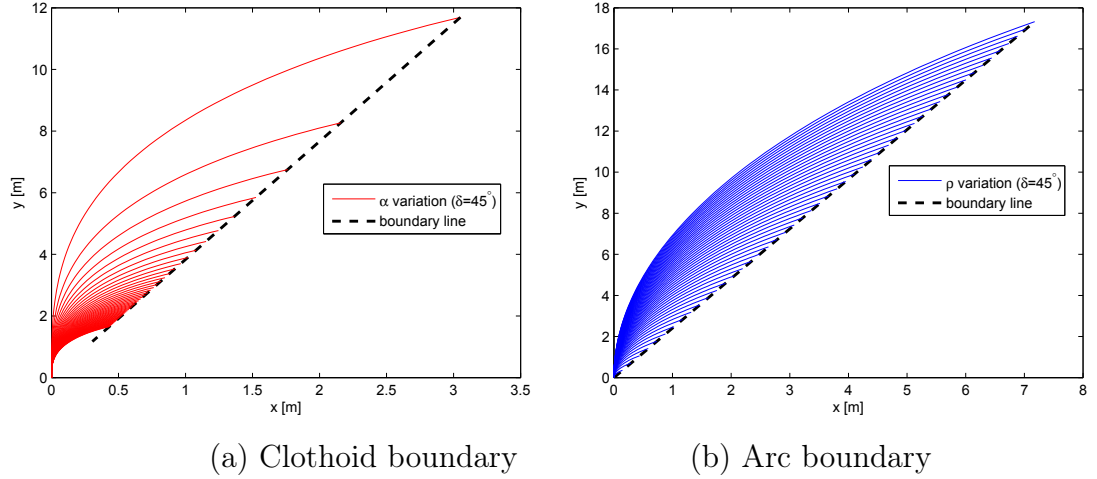
Figure B.2: Boundary lines for fixed \delta = 45^\circ [deg]
