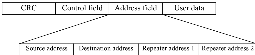
Figure 4.1: Structure of address field 1
