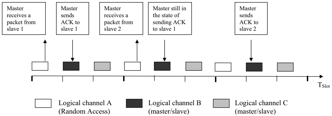
Figure 7.5: ACK delay in Master/slave channel
