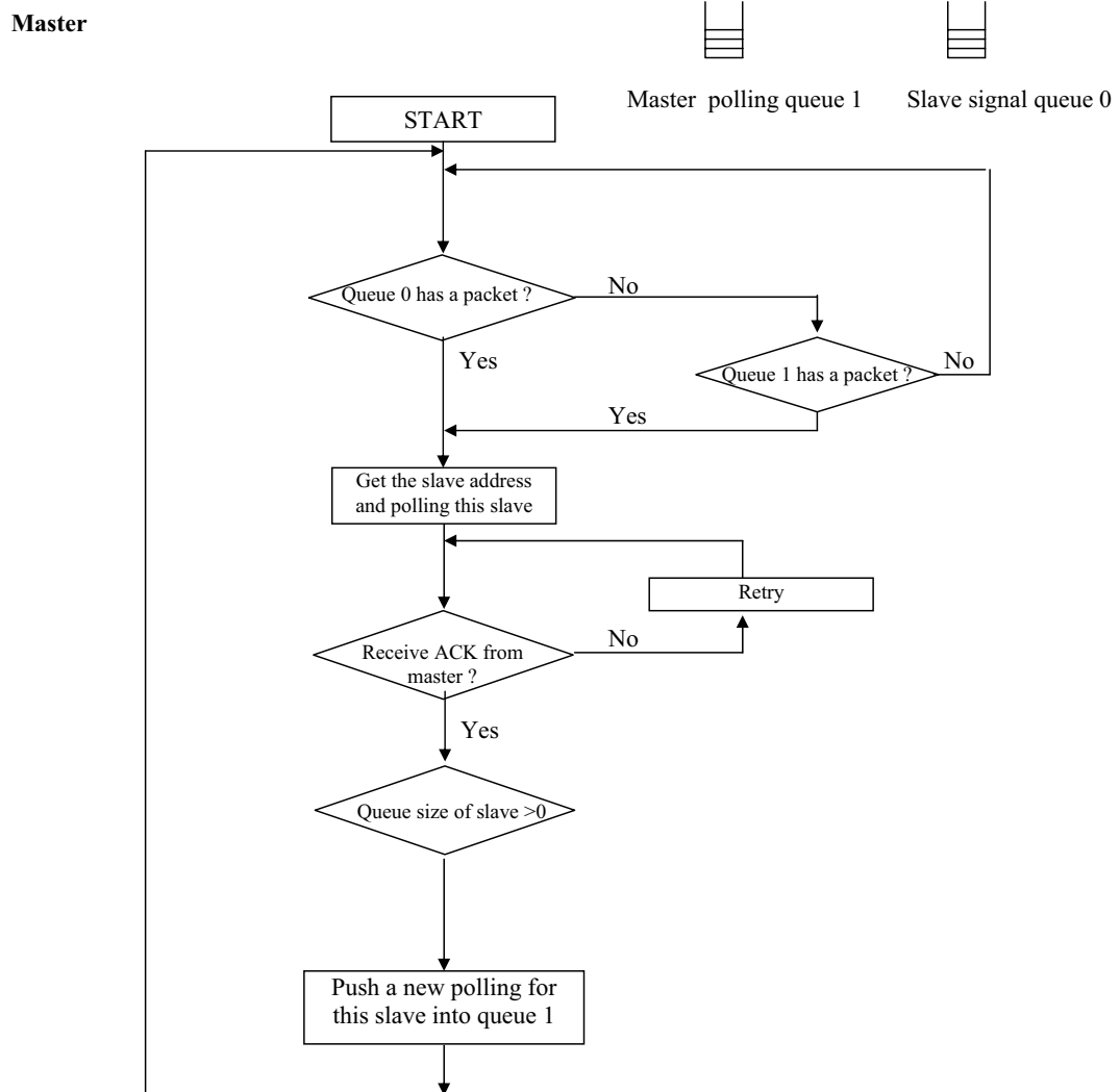
Figure 7.12: Block diagram of the master transmission
