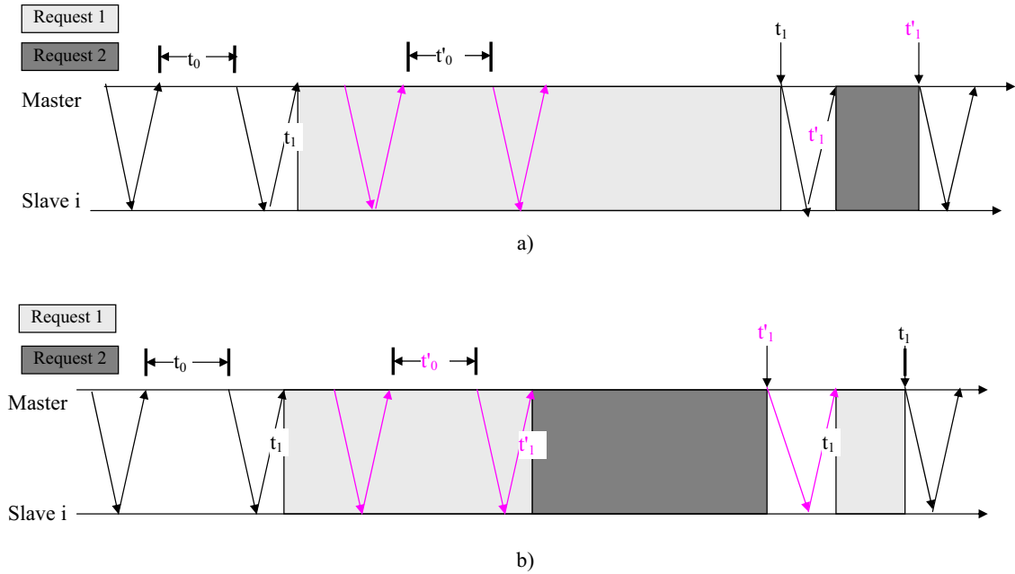
Figure 6.3: Master poll strategy for determination of Slave Application Layer response
