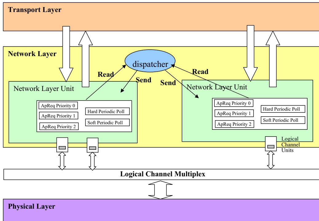
Figure 6.2: Dispatcher location and priority system for each Network Layer Unit
