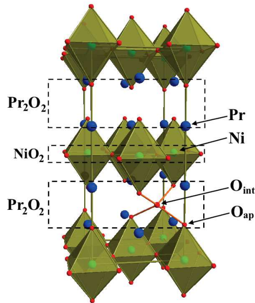
Figure 8.1: Structure of \text{Pr}_2\text{NiO}_{4+\delta} , described as a succession of \text{NiO}_2 and \text{Pr}_2\text{O}_2 layers. Excess oxygen ( \text{O}_{int} ) stays in the interstitial position inside the \text{Pr}_2\text{O}_2 layer coordinated by 4 apical oxygen atoms ( \text{O}_{ap} ).
