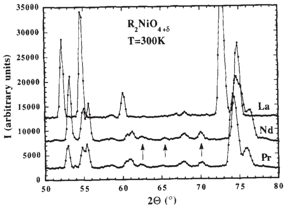
Figure 8.7: Portion of the diffraction pattern for \text{R}_2\text{NiO}_{4+\delta} (R = La, Pr and Nd). Arrows indicate the main differences between the different patterns. Taken from FIG. 2 of ref. [107]
