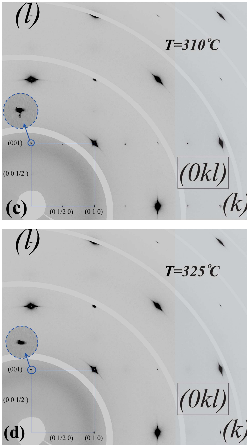
Figure 7.5: Evolution of the (0kl) plane during heating of \text{SrFeO}_{2.5} single crystal in air (c) at 310^\circ\text{C} and (d) 325^\circ\text{C} . The pseudocubic cell is outlined in the blue square.
