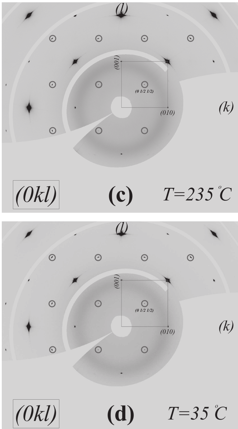
Figure 7.10: Evolution of the (0kl) plane (reconstructed in the pseudocubic cell) during cooling of SrFeO 2.5 single crystal (c) 235 °C and (d) 35 °C. The pseudocubic cell is marked in grey square. The encircled reflections indicate the newly growing reflection.
