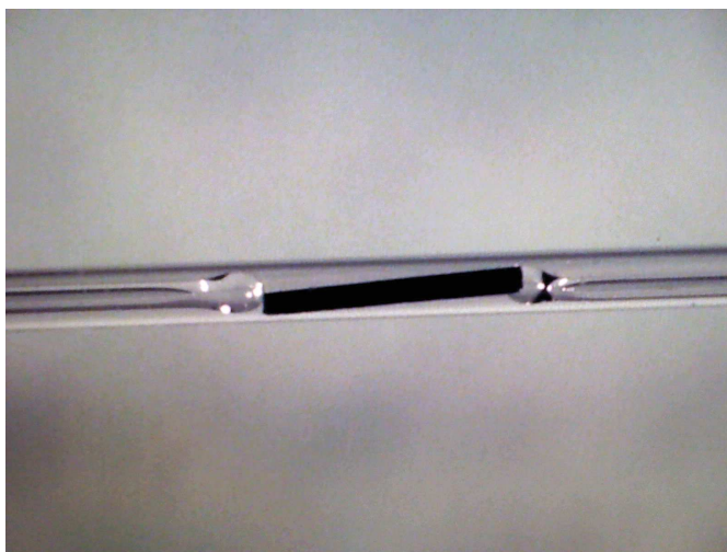
Figure 7.1: Cylindrical shaped single crystal of SrFeO 2.5 of \sim 100\mu\text{m} in diameter inside a 300\mu\text{m} quartz capillary supported by other two quartz capillaries from the two ends. The choice of such cylindrical shaped crystal was preferential for absorption related problems.
