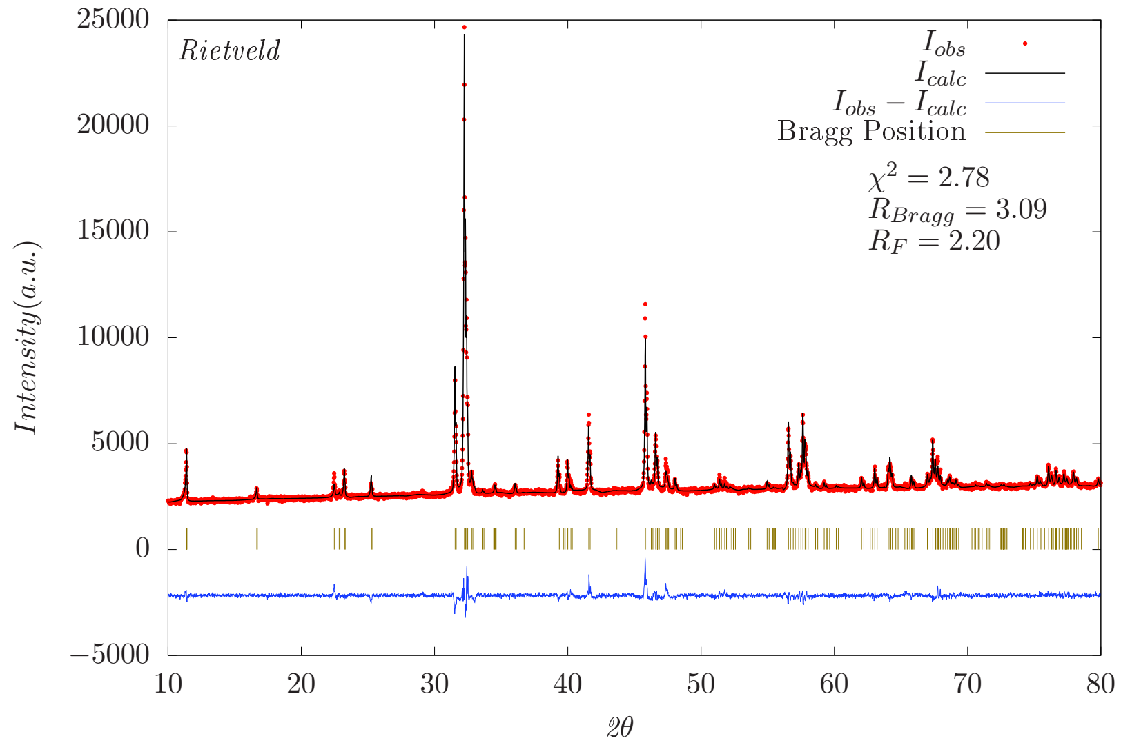
Figure 5.2: Rietveld refinement on X-ray powder diffraction data obtained from ground as grown SrFeO 2.5 single crystal in Imma structure model.
