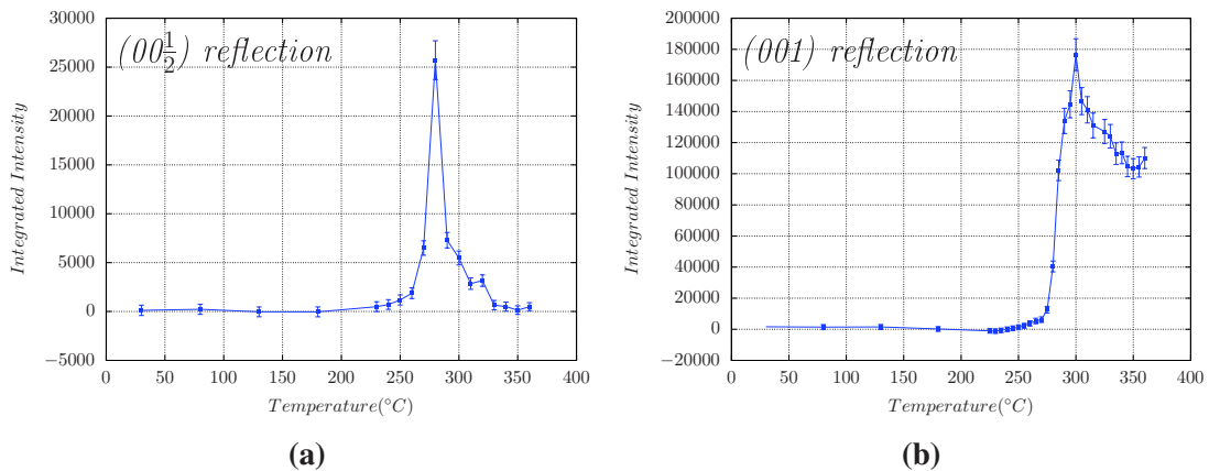
Figure 7.6: Integrated intensity followed on the newly grown (a) (00\frac{1}{2})_p reflection and (b) (001)_p reflection in the temperature range 35\text{ }^\circ\text{C} - 360\text{ }^\circ\text{C} .
