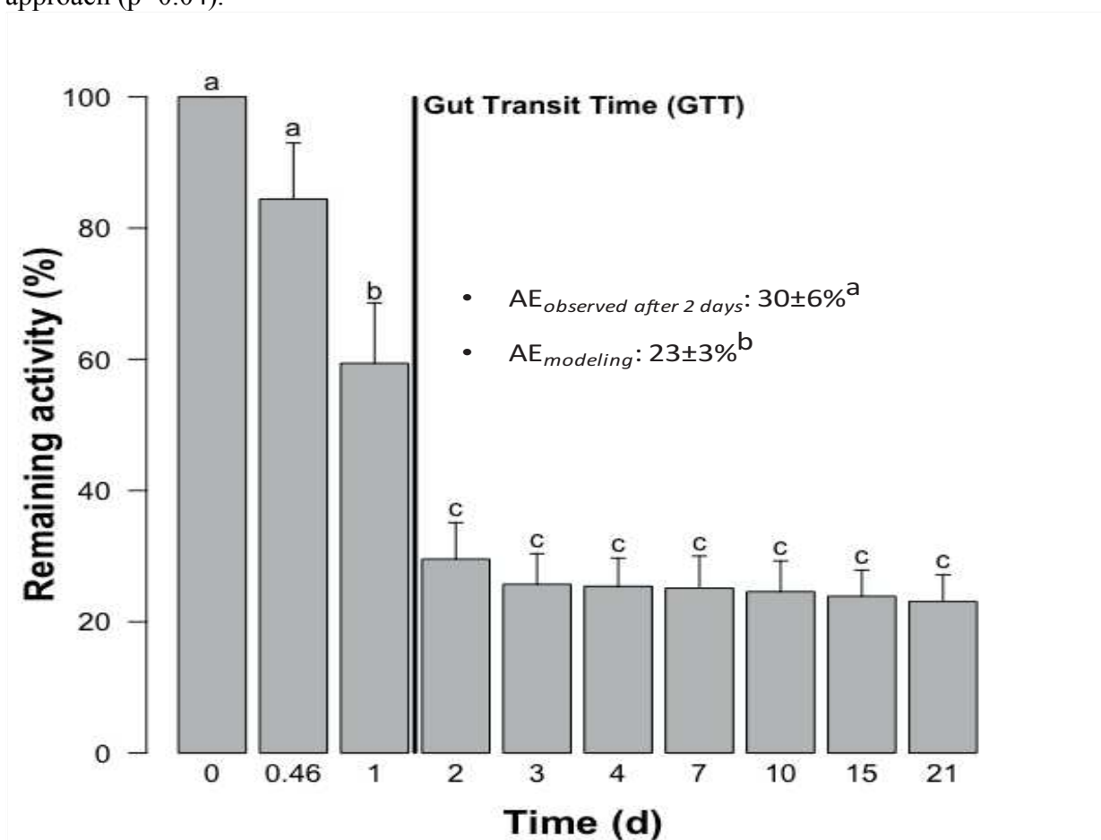
Figure 1. Remaining activities of ^{54}\text{Mn} during a 21-d depuration in turbot ( n=12 ) fed radiolabelled with pellets. Data from Pouil et al. (2017, supplementary material). For comparison, AE observed after 2 days of depuration (“short-term” approach) and AEs estimated using kinetic modeling (“long-term” approach) are indicated as bullet-points. Letters indicated significant differences ( p<0.05 ).
