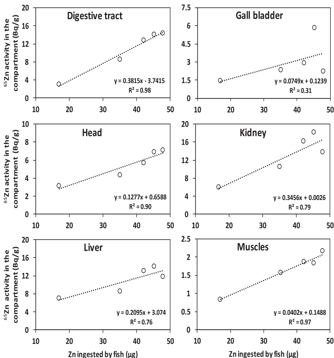
Figure 2. Relationship between the estimated Zn ingested by fish ( \mu\text{g} ) and ^{65}\text{Zn} stored in each body compartments ( \text{Bq g}^{-1} wet wt) for the five single-fed turbot from the Experiment 2.
