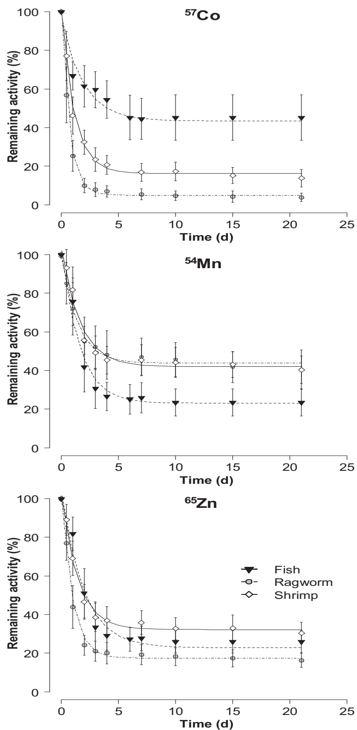
Figure 3. Influence of type of food (see Table 2) on whole-body depuration of ^{57}\text{Co} , ^{54}\text{Mn} and ^{65}\text{Zn} in turbot (% remaining activities, means \pm SD). Parameters and statistics of depuration kinetics are given in Table 4.
