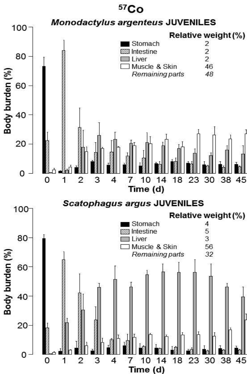
Figure 2. ^{57}\text{Co} distribution among 4 body compartments (intestine, stomach, liver, and muscles and skin) of juvenile silver moony ( M. argenteus ) and juvenile spotted scated ( S. argus ) over the depuration phase after feeding with radiolabelled brine shrimp. At each time three fish were dissected. All the values are expressed as percentage of the whole-body activity (means + SD).
