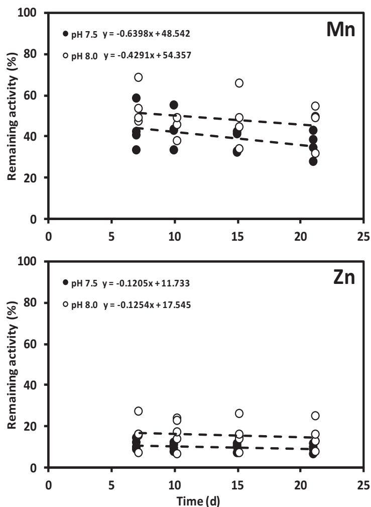
Figure S1. Remaining activities of Mn and Zn after a radiolabeled single-feeding using mussels in turbot's acclimated at two different pH (7.5 and 8.0) and pre-exposed for three weeks to dietary brevetoxins.
