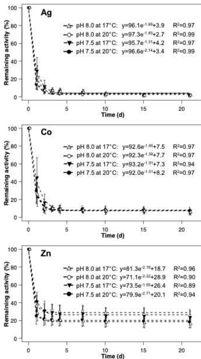
Figure 1. Influence of temperature and pH (see details of experimental conditions in Table 1) on whole-body depuration of ^{110m}\text{Ag} , ^{57}\text{Co} and ^{65}\text{Zn} in juvenile turbot ( n = 6-8 ; percent remaining activities, means \pm SD).
