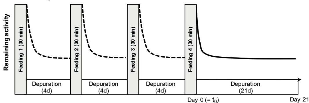
Figure 1. Protocols of (A) single-feeding and (B) multi-feeding experiments. For each radiolabeled pellet feeding, turbot were fed ad libitum for 30 min and the uneaten food was then removed. For comparison between single-feeding and multi-feeding experiments, we considered the Day 0 and the Day 21 respectively as the beginning and the end of the depuration period after the last feeding.
