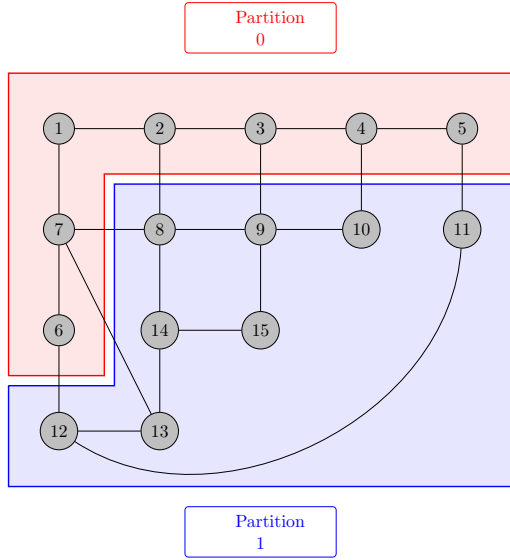
Figure 3.3 – Row partitioning
