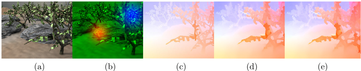
Figure 4.1: Visualization of the robustness of the proposed ROF-NND method against illumination changes. (a) Original frame10 of Grove3. (b) Frame11 of Grove3 with illumination. (c) Ground truth flow. (d) Result with ROF-NND before illumination changes ( AEPE/AAE = 0.58/6.05 ). (e) Result of ROF-NND after illumination changes ( AEPE/AAE = 0.58/6.05 ).
