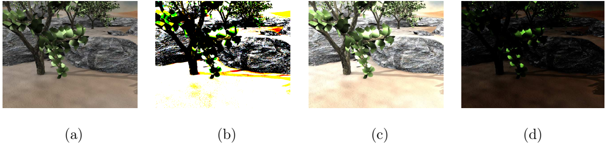
Figure 4.9: Simulated illumination changes on the second image of the Grove2 image pair. a) Original image I_{in} b) I_{out} with an additive term a = 30 , c) I_{out} with multiplicative m = 1.8 and d) I_{out} with \gamma = 3.5 .
