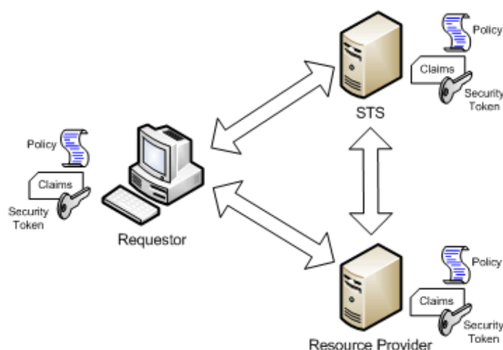
FIGURE 3.5 – WS-Trust [4].
