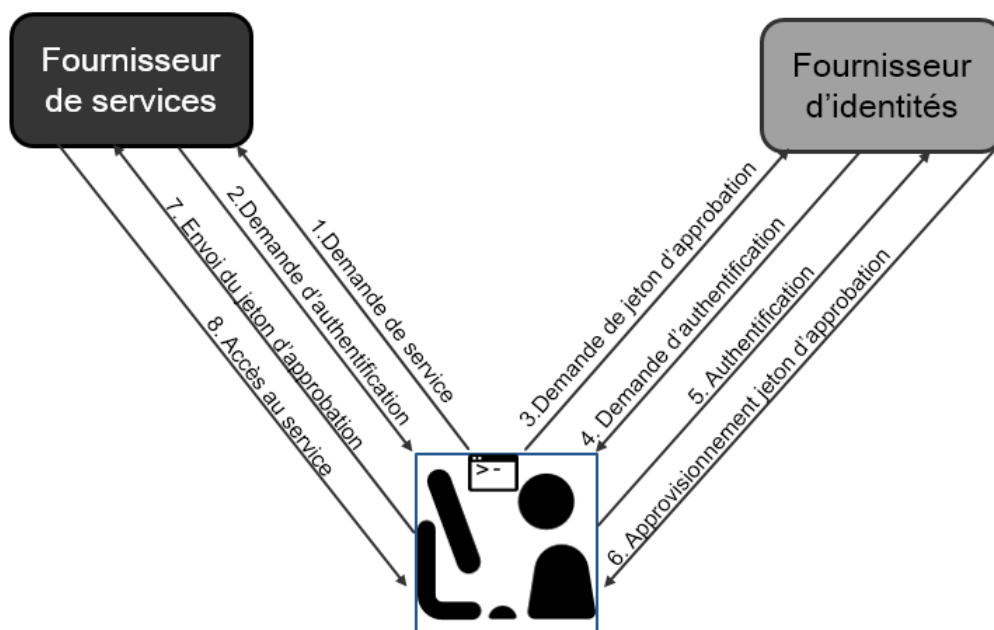
FIGURE 4.5 – Authentication Active-client .
