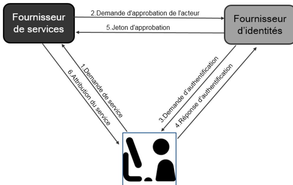
FIGURE 4.4 – Authentication Interactive .
