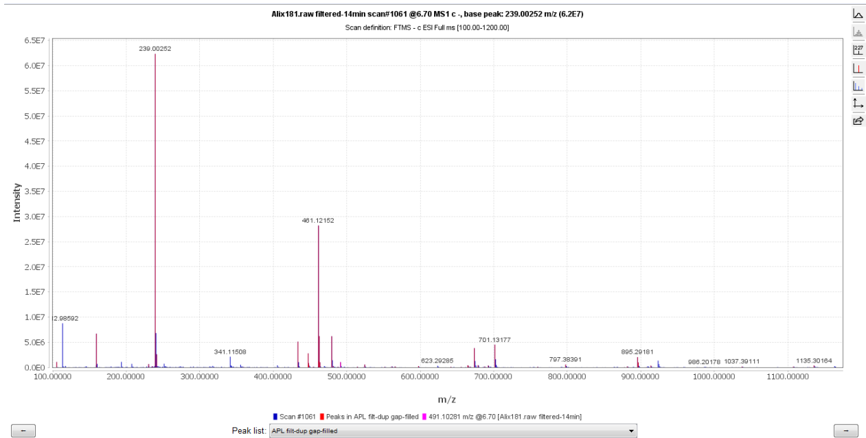
Figure 116: Moellendorffiline
