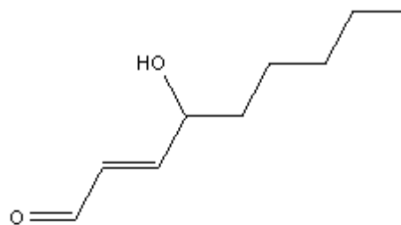
Figure 8: 4-hydroxynonéal
