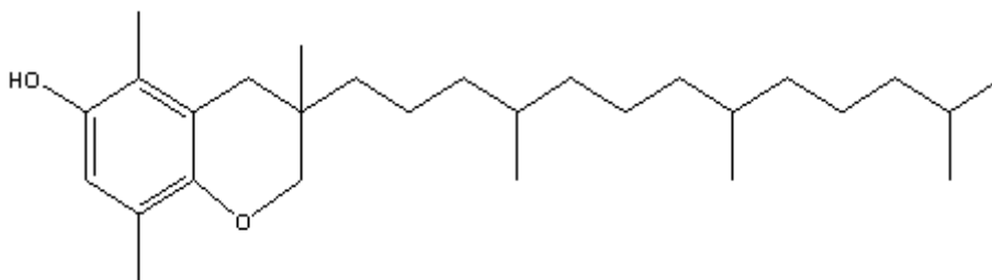
Figure 11: vitamine E.
