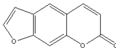
Figure 28: Le psoralène.
