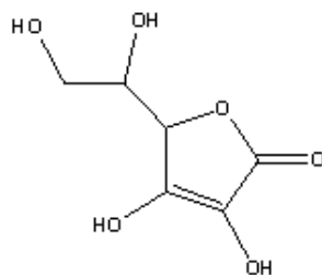
Figure 12: Vitamine C.
