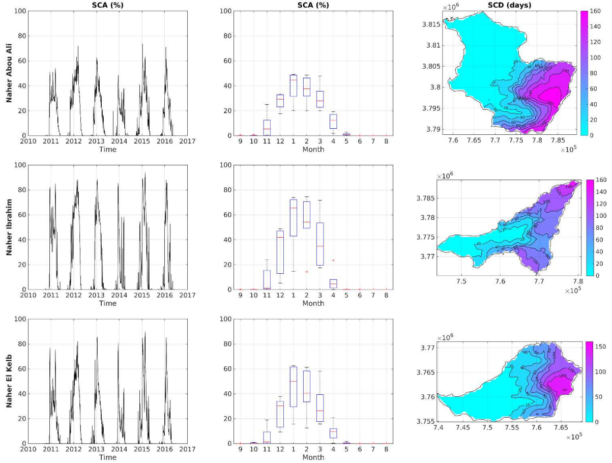
Fig. 3.9. From left to right: time series of the snow cover area (SCA, percentage of the basin area), box plot of mean monthly SCA, and snow cover duration (SCD) for (from top to bottom) the Abou Ali, Ibrahim, and El Kelb River basins.
