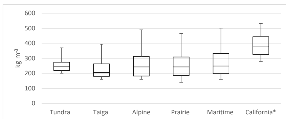
Fig. 2.1. Variation in the mean monthly snow density (Oct-June) ( \text{kg m}^{-3} ) adopted from Brown and Mote (2009) for the major climate regions. *California monthly snow density means (Jan-June) are based on long-term monthly data records (more than 20 years) retrieved from 46 snow courses and 26 SNOTEL stations (data are available online at wcc.nrcs.usda.gov/snow/ ). The average snow depth and standard deviation, not shown, were as follows: Tundra (43.8 cm, 24.7 std dev), Taiga (59.6, 22.7), Alpine (130, 82.5), Prairie (88.5, 72.8), and Maritime (176.6, 149.9) (Sturm et al., 2010), and the average for California calculated from long term monthly snow courses and SNOTEL data was 146.1 cm (std dev = 97.5).
