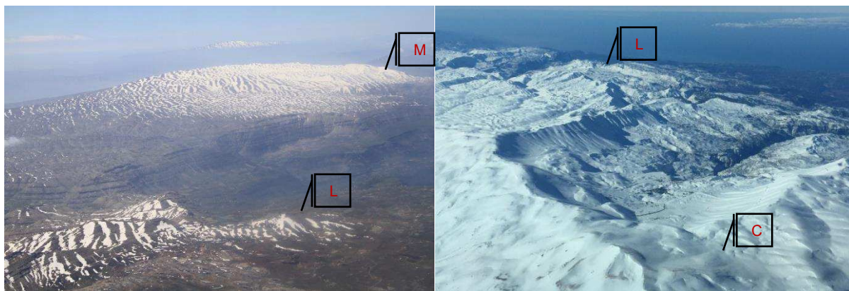
Fig. 3.2. Overview of the mountain topography at (a) Laqlouq and Mzar, and (b) Cedars, Mount Lebanon. The images were captured on 6 May 2011 (a) and 21 February 2015 (b) (courtesy of the author). The locations of the AWSs are shown approximately on the images where the letters M, L, and C represent the stations at MZA, LAQ, and CED, respectively (see Table 3.1). The topography near Laqlouq (LAQ) is a relatively low plain (elevation between 1600 and 1800 m a.s.l.) and low-elevation mountains (1900 – 2100 m a.s.l.). The region near Mzar (MZA) is characterized by rugged terrain (1600 – 2200 m a.s.l.) and mid-elevation plateau (elevation range 2300 – 2500 m). The high-elevation plateau (shown partially in (b) near Cedars (CED)) have an elevation range between 2700 and 3000 m a.s.l. Snow persists until the end of May in the mid-elevation mountain regions (plateau and rugged terrain region above 2300 m a.s.l.). The low-elevation and mid-elevation regions (1300 – 2000 m a.s.l.) are usually snow-free by mid-March to mid-April.
