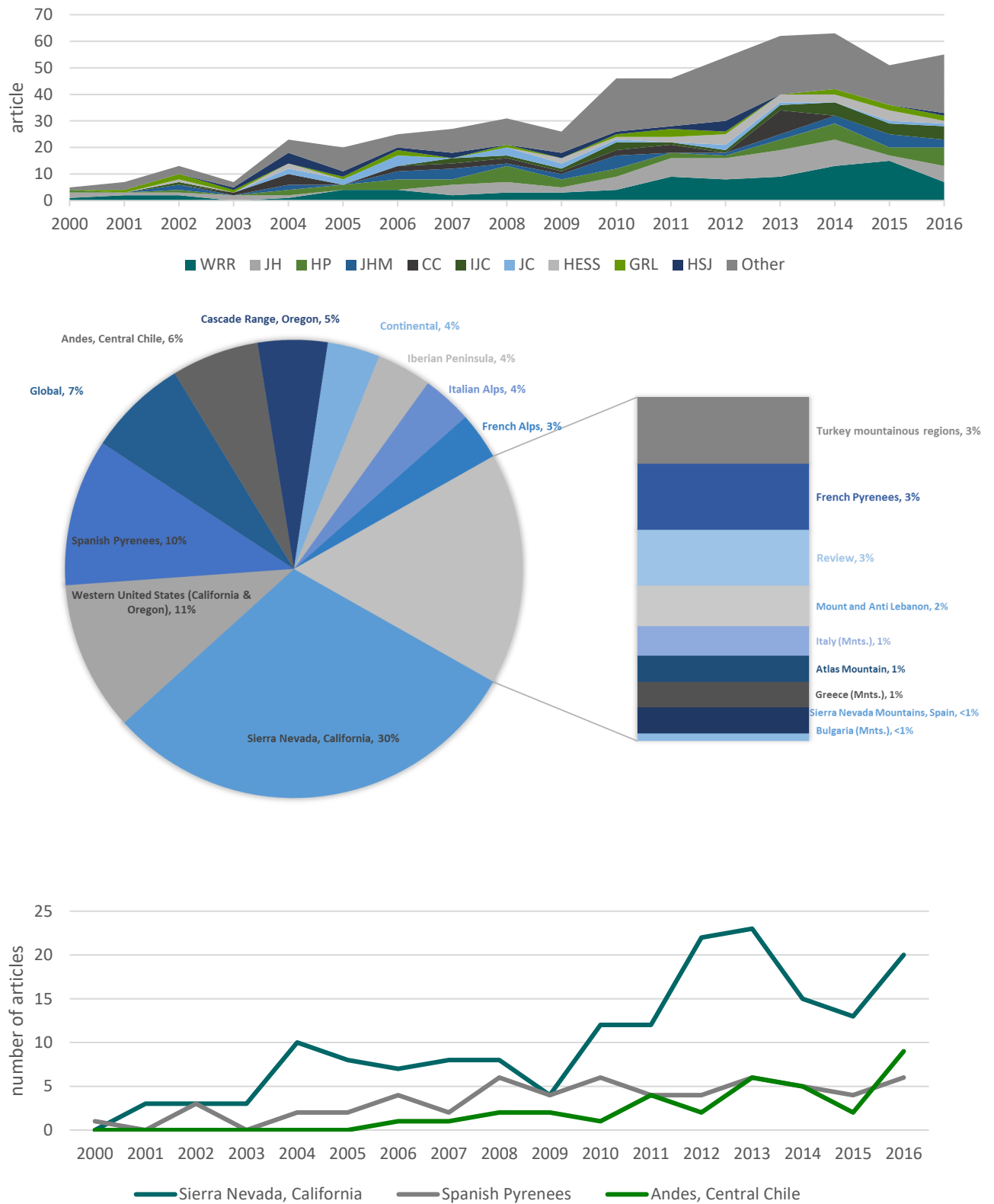
Fig. 2.3. Key bibliometric indicators were the following (from top to bottom): (a) cumulative yearly number of publications per journal (based on 561 articles published between 2000 and 2016); (b) Distribution of studies by major mountain regions shown; and (c) number of yearly published papers in California (excluding western US regional studies) (30%), Spanish Pyrenees (10%), and Chilean Central Andes (6%).
