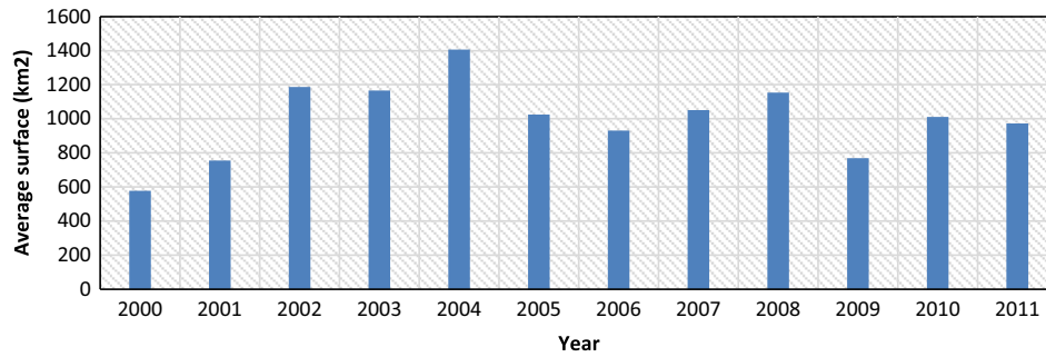
Fig. 8. Average yearly distribution of snow surface between 2000 and 2011.
