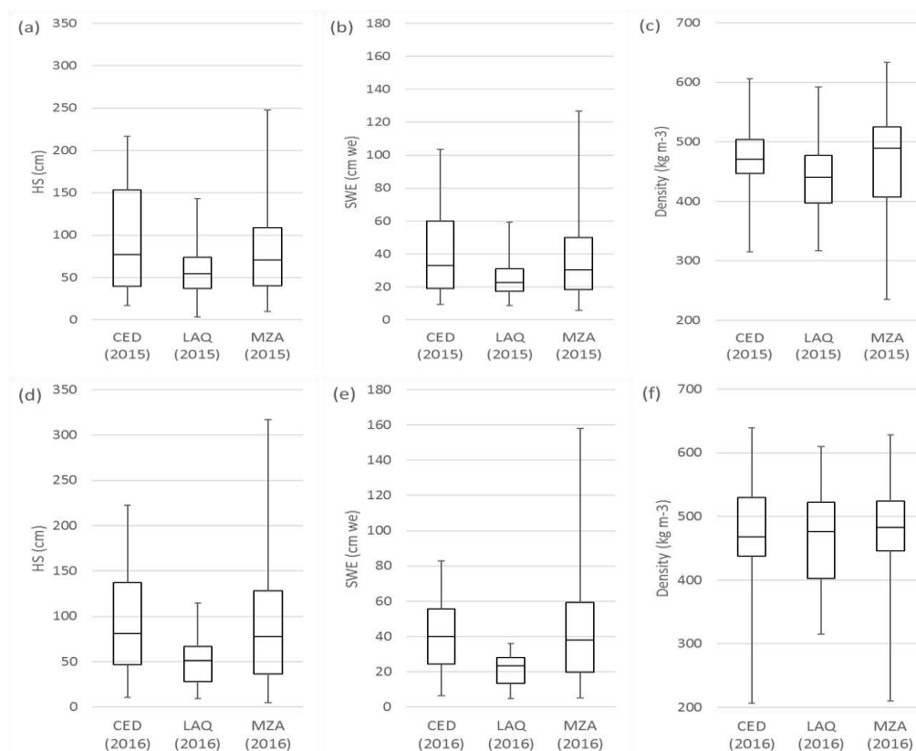
Fig. 3.7. Box-and-whisker plots for nonzero data: (a) snow height, (b) SWE, and (c) snow density over two snow season 2014–2015 ( n = 311 ) and (d) snow height, (e) SWE, and (f) snow density over snow season 2015–2016 ( n = 371 ) distributed by region where CED (elevation range, 1650–2900 m), LAQ (1300 – 1850 m), and MZA (1350 – 2350 m). The box brackets represent 25% and 75% of the data (lower and upper boxes, respectively). The whiskers are at minimum and maximum values.
