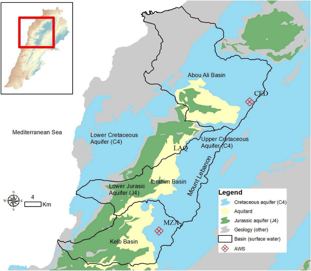
Fig. 1.5. Major groundwater system showing the major upper Cretaceous aquifer (C4) where most the snow falls in the Mount Lebanon. Both the Cretaceous (C4) and Jurassic (J4) aquifer systems are chareteized by their high Karstification.
