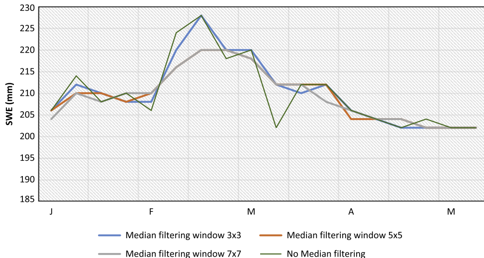
Fig. 5. Comparison between median filtered SWE and raw SWE in 2010.
