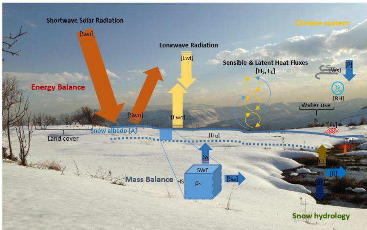
Fig. 2.4. Major climate forcing and snow processes in Mediterranean-like mountainous regions with emphasis on the specific objectives shown here for mountain hydrology and snowpack dynamics. Where SWi and SWo are incoming and outgoing shortwave radiation, respectively; Lwo and Lwi are the emitted and incoming longwave radiation, respectively; P is precipitation, Ws is wind speed, and RH is relative humidity; HM is sensible heat flux; Ts is surface temperature and Tg is ground temperature; HS is snow depth, ds is snow density, and SWE is snow water equivalent; Ss is snow sublimation and Sm is snow melt; ET is evapotranspiration, R is surface runoff, G is subsurface and groundwater flow. The background image was taken in Laqlouq at 1850 m a.s.l. (Mount-Lebanon) on February 20th, 2016 (courtesy of the author).
