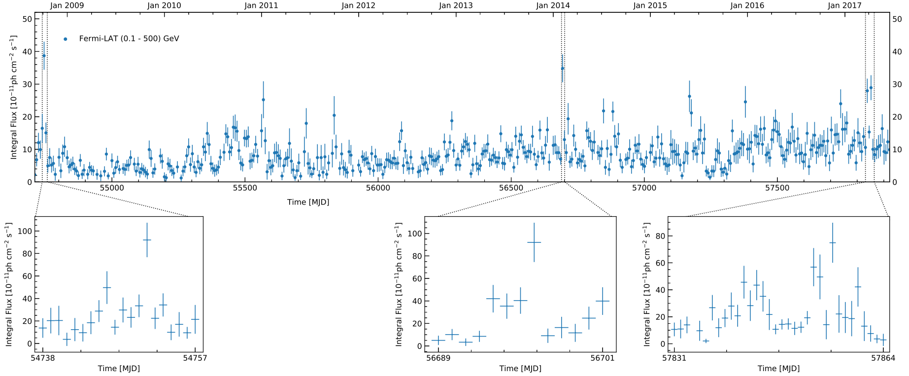
Figure 4.5: Top panel: Long-term lightcurve of B2 1215+30, from 2008 September 1st to 2017 June 30. The integral fluxes are calculated in one week time bins. The major flares, with weekly averaged flux \Phi > 3.0 \times 10^{-07} \text{ cm}^{-2} \text{ s}^{-1} are indicated by dashed black lines. Bottom panel: lightcurve in one day time bins around the major flares detected during October 2008, February 2014 and April 2017.
