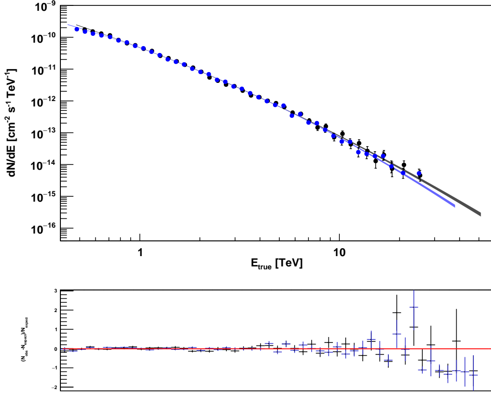
Figure 5.18: Superimposed Crab Nebula spectrum from two different seasons as described in the text. The first season is represented by the black points and the second season by the blue ones. The 1\sigma confidence interval of the fitted spectrum shape are plotted by solid lines. The spectra are fitted with a curved power-law spectral shape and are compatible within the estimated H. E. S. S. systematic uncertainties. The residual plot in the form (N_{\text{obs}} - N_{\text{exp}})/N_{\text{exp}} are shown in the bottom part.
