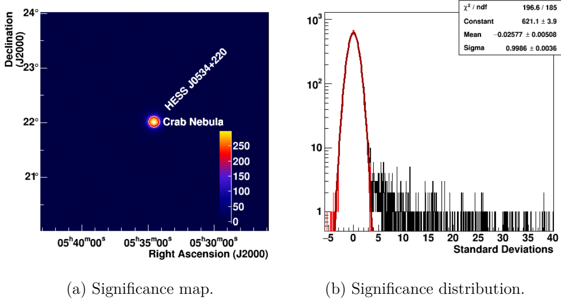
Figure 5.7: (a) The significance map of the Crab Nebula using all the H. E. S. S. I data set with Std cuts. The position of the Crab Nebula is showed in the center. (b) The corresponding significance distribution of the whole map is shown in black. The distribution after excluding a circular region of 0.25 degrees around the source with a Gaussian fit is shown in red and the fit values are shown in the plot.
