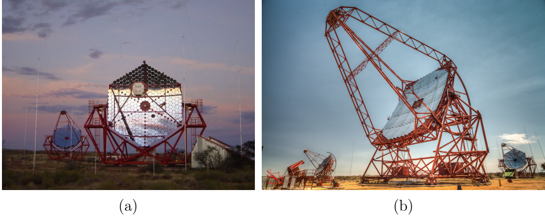
Figure 3.3: (a) The H. E. S. S. I telescopes with reflective area made of facet mirrors arranged in Davies-Cotton fashion. (b) The H. E. S. S. II telescope with refractive area made of facets arranged in parabolic fashion. Image courtesy of H. E. S. S.
