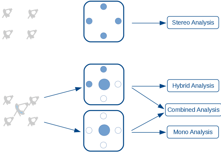
Figure 3.9: Schematic illustration of different event trigger and reconstruction types of the H.E.S.S. experiment. The top part of the figure correspond to the trigger of H.E.S.S. Phase-I which are reconstructed with Stereo. In the bottom are shown the H.E.S.S. Phase-II trigger modes. The array can trigger CT5 and CT1-4 and only CT5 and reconstruct events by using the Combined, Hybrid and Mono.
