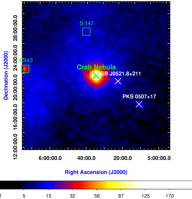
Figure 6.8: A 15^\circ \times 15^\circ RoI counts map centered on the position of the Crab Nebula. This correspond to the period of the 2016 flare and the brightness of the Crab Nebula is visible. The Crab Nebula is marked with green cross and other bright sources are marked as well. The squared symbols indicate two extended sources located within RoI.
