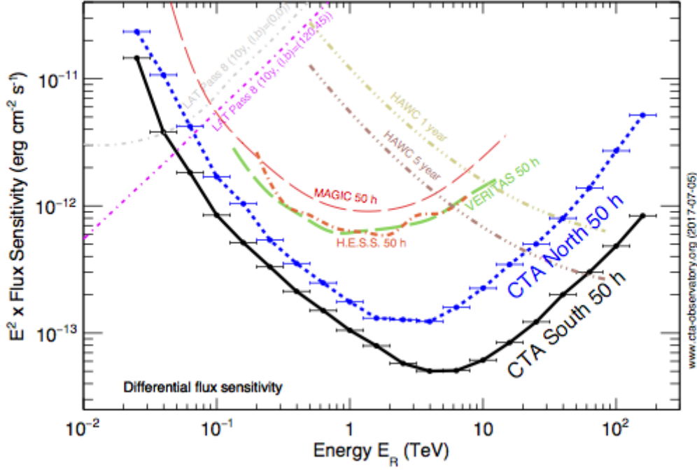
Figure 2.14: The differential sensitivity of CTA South and North compared to H.E.S.S., MAGIC, VERITAS and HAWC experiments. The CTA South and North, for 50 h of observations are expected to have a higher sensitivity with respect to other experiments and extend up to 100 TeV. Image courtesy [96].
