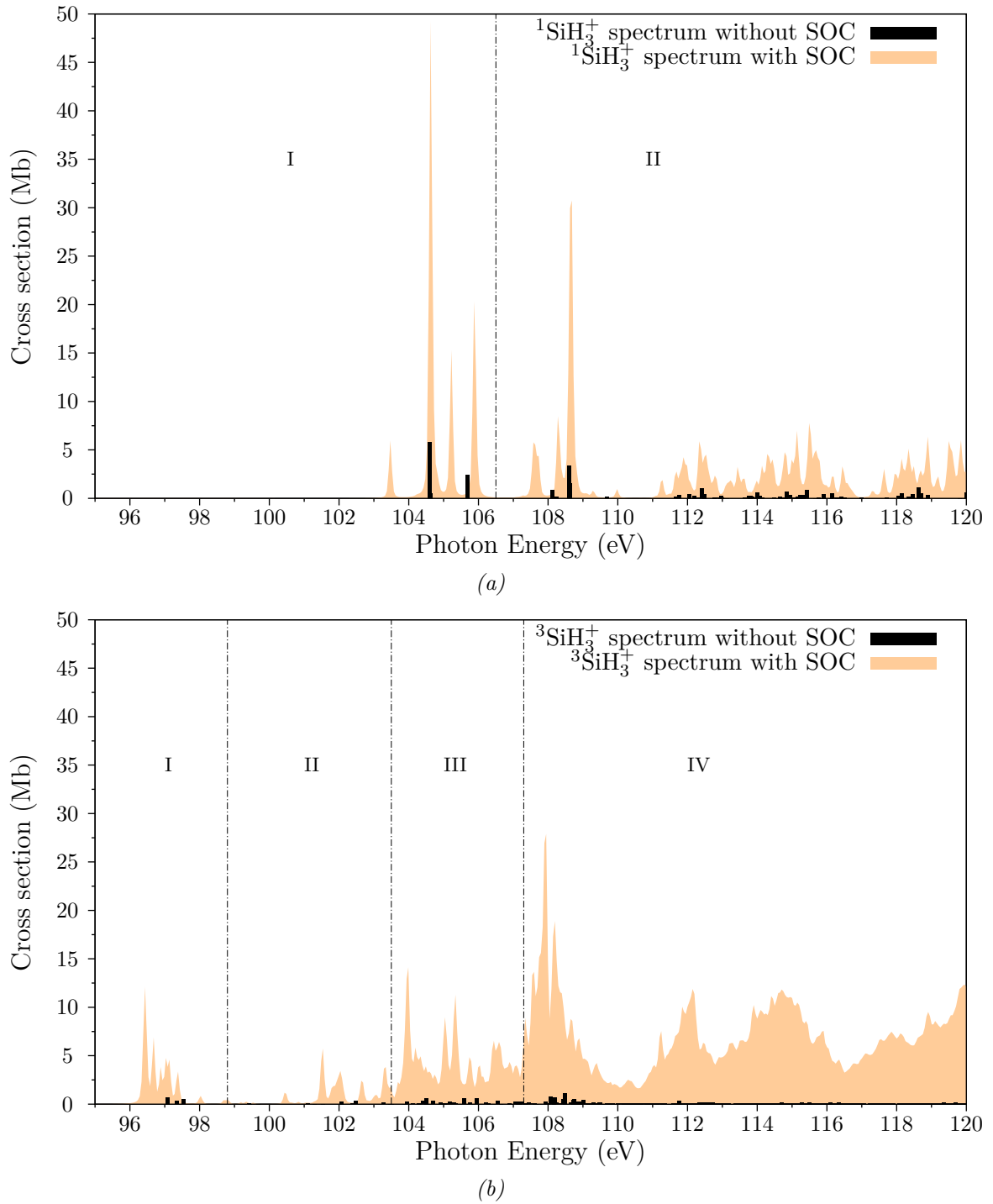
Figure B.7: Vertical X-ray photoabsorption spectra of ^1\text{SiH}_3^+ (top) and ^3\text{SiH}_3^+ (bottom)
