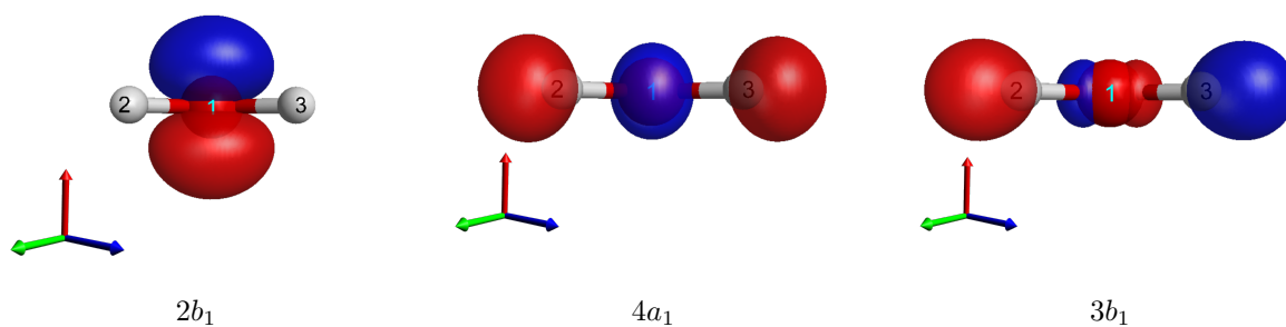
Figure 5.14: OH_2^+ molecular orbitals involved in the electronic transition.
