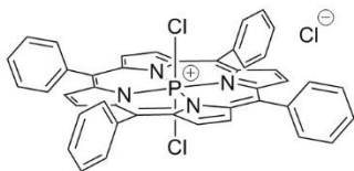
15, [P(TPP)Cl 2 ] + Cl -
