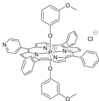
23, [P(MPyP)(OPhOMe) 2 ] + Cl -
