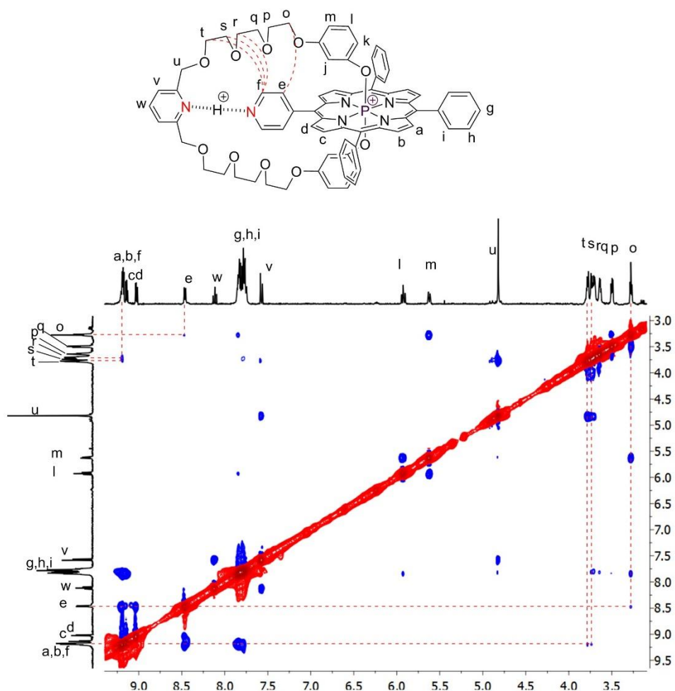
Fig. 1.71 NOESY spectrum ( \text{CD}_3\text{CN} , 400 MHz, 25 °C) of turnstile#1 in its closed state.
