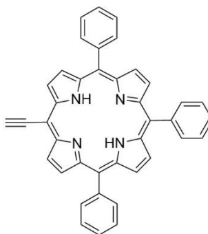
36, H 2 EtP
