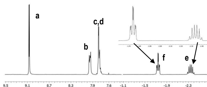
Fig. 1.31 ^1\text{H} -NMR ( \text{CDCl}_3 , 500 MHz, 25 °C) spectrum of [\text{P}(\text{TPP})(\text{OEt})_2]^+ and assignment of the signals, proton attributions are given in Fig. 1.30 .
