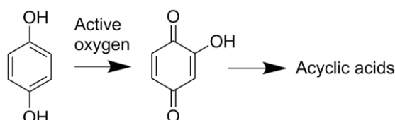
Fig. 2.25 HQ oxidation by active forms of oxygen.
