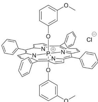
17, [P(TPP)(OPhOMe) 2 ] + Cl -
