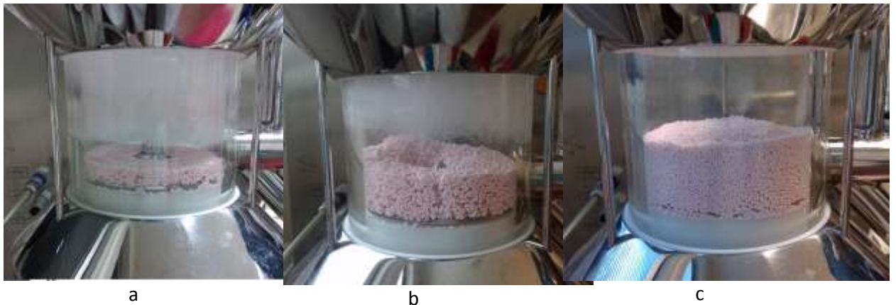
Figure 5.9. Depositing of coating material on the walls of the partition with three different inventories 15 % (a), 30% (b), 50% (c) of the maximum capacity in the product container IPC1.
